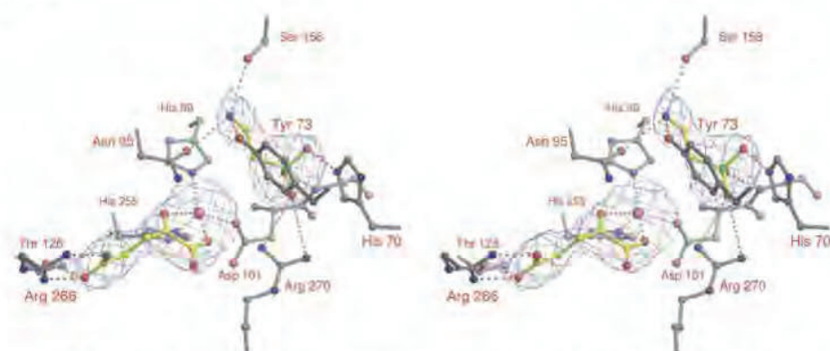
FIGURE 4: Stereodiagram of the active site of TauD. Shown are the protein ligands to the iron, the two substrates and other important protein side-chains. A 2mF_o - DF_o electron density map is shown contoured at 1.0 sigma around the substrate molecules.
