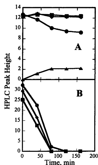
Fig. 3. D egradation of cinnamic acids by intact cells. The time dependence was examined for decomposition of 2,4-dichlorocinnamic acid (panel A) and cinnamic acid (panel B) by R. eutropha JMP134 (pJP4) (●), R. eutropha JMP228 (■), and R. eutropha JMP228 (pBH501aE) (◆) by using HPLC methods and analysis of the resulting absorbances at 230 nm. In addition, the time dependence was determined for production of the metabolite derived from 2,4-dichlorocinnamic acid by R. eutropha JMP134 (pJP4) (▲) in panel A.
