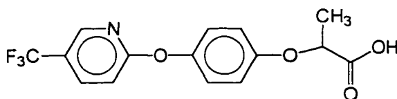
X=H 2-[4-[(5-trifluoromethyl)-2-pyridinyl]oxy]- phenoxy]propionic acid Fluazifop
