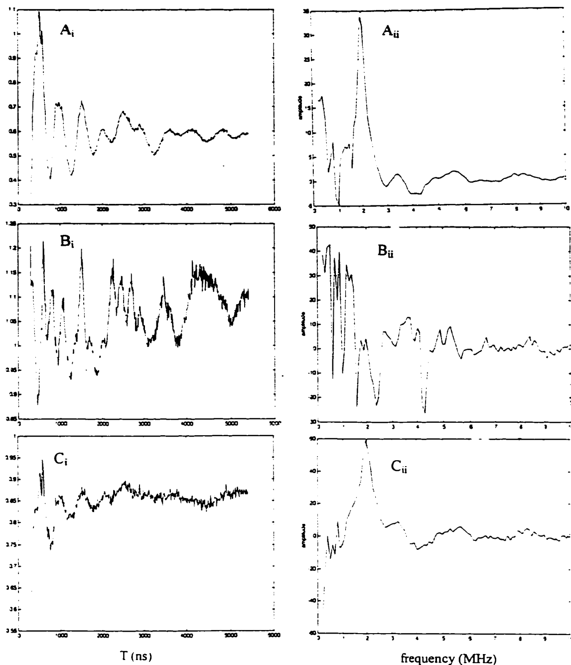
Figure 21. Three-pulse ESEEM spectra of resting and substrate-bound Cu-TfdA in deuterated versus protonated solvent.
