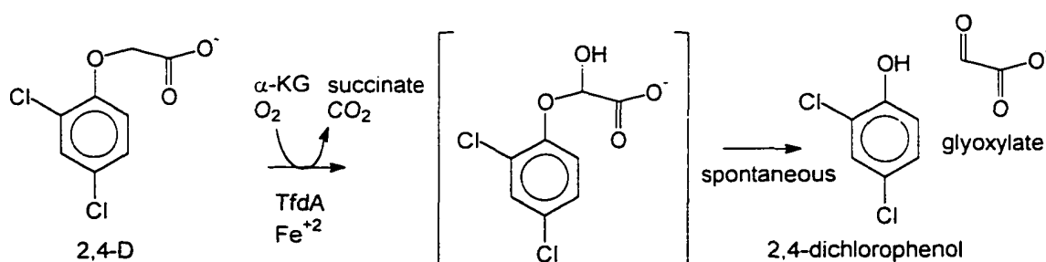
Scheme 13. Reaction catalyzed by TfdA
