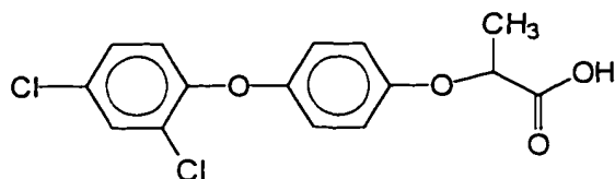
2-[4-(2,4-dichlorophenoxy)phenoxy]- propionic acid Diclofop
