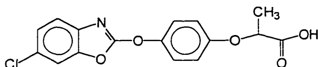
2-[4-[(6-chloro-2-benzoxazolyl)oxy]- phenoxy]propionic acid Fenoxaprop
