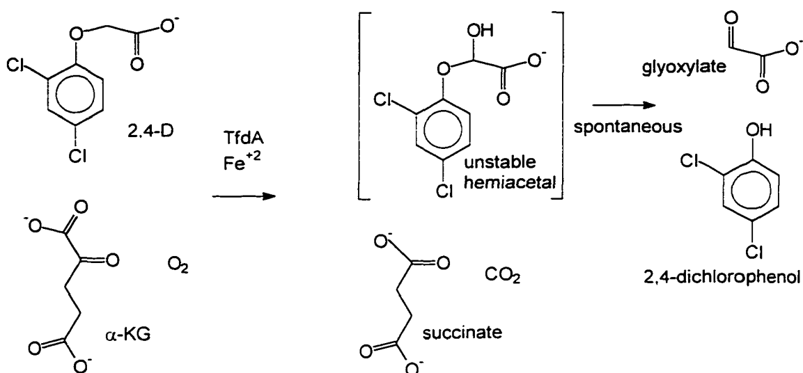
Scheme 2. Reaction catalyzed by TfdA.
