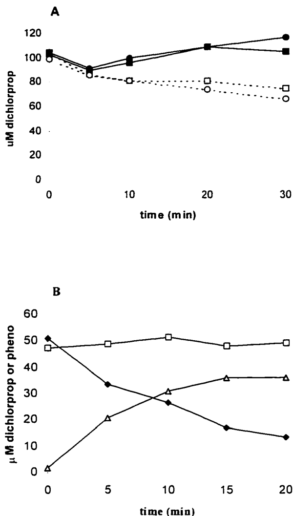
Figure 16. Stereospecificity of activity of cell extracts and purified protein towards racemic dichlorprop, measured by chiral HPLC.
