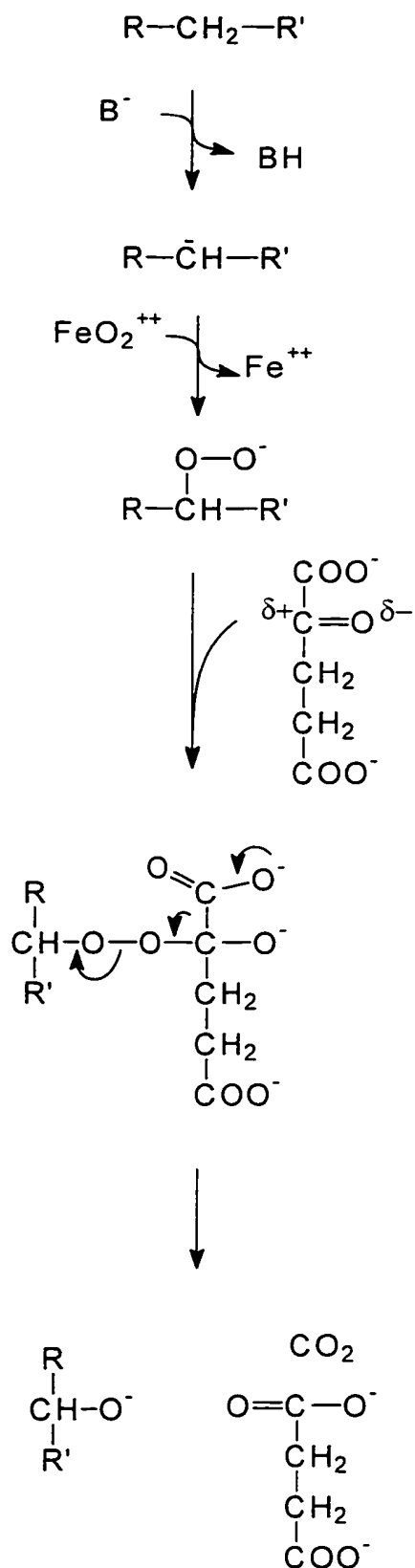
Scheme 8. Hydroperoxy mechanism for \alpha -KG-dependent dioxygenases.
