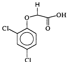
2,4-dichlorophenoxyacetic acid 2,4-D
