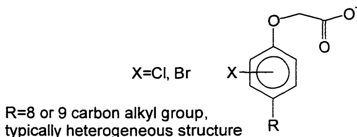
Scheme 15 General structure of halogenated alkylphenoxyacetic acids
