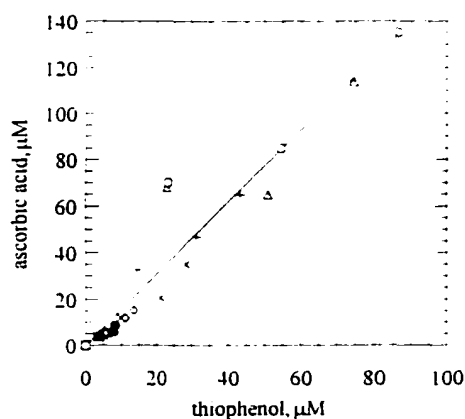
Figure 4. Stoichiometry of thiophenol production and ascorbate consumption during TPAA turnover.
