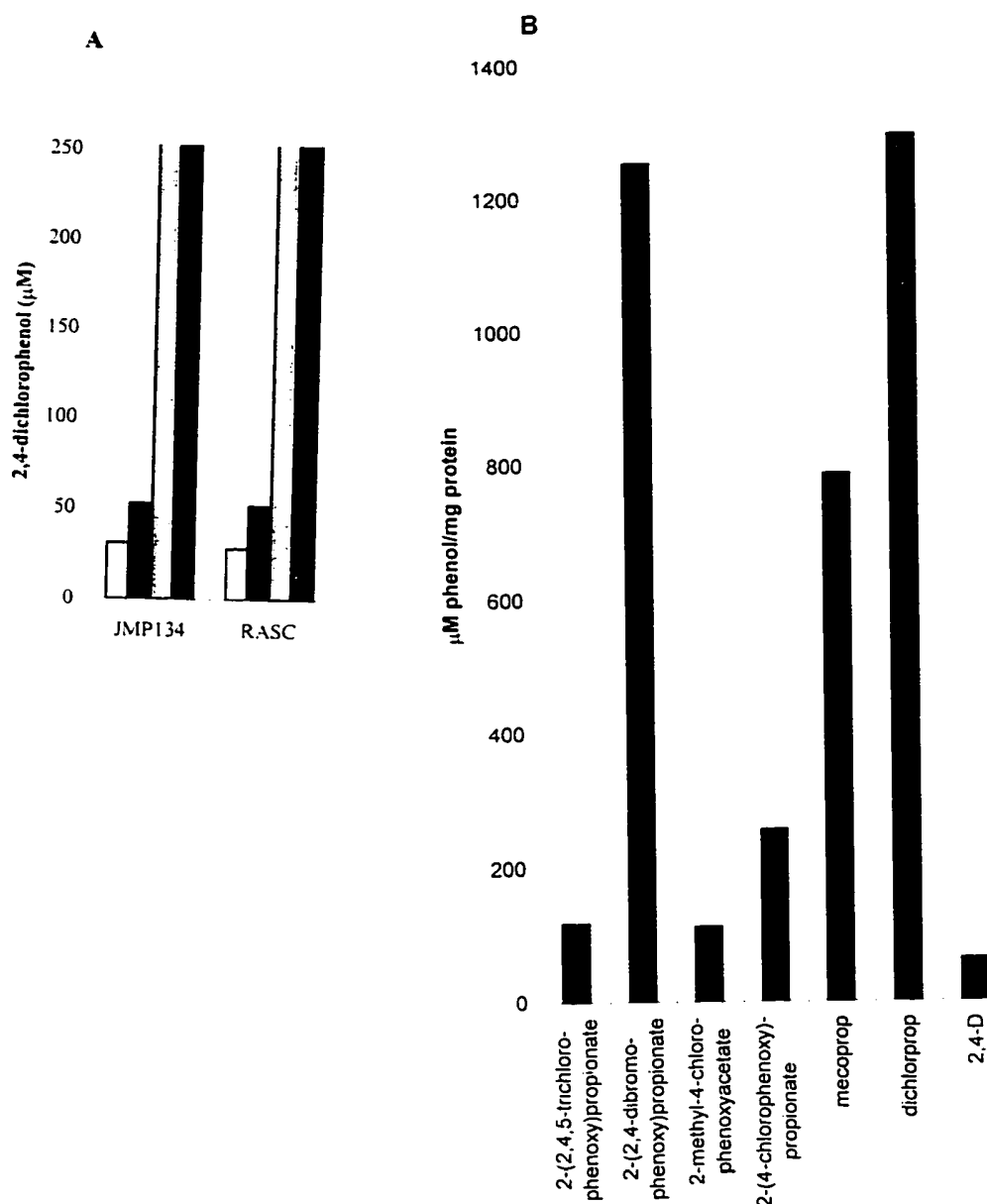
Figure 12. Activity of cell extracts towards phenoxy herbicides.
