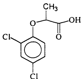
2-(2,4-dichlorophenoxy)propionic acid Dichlorprop
