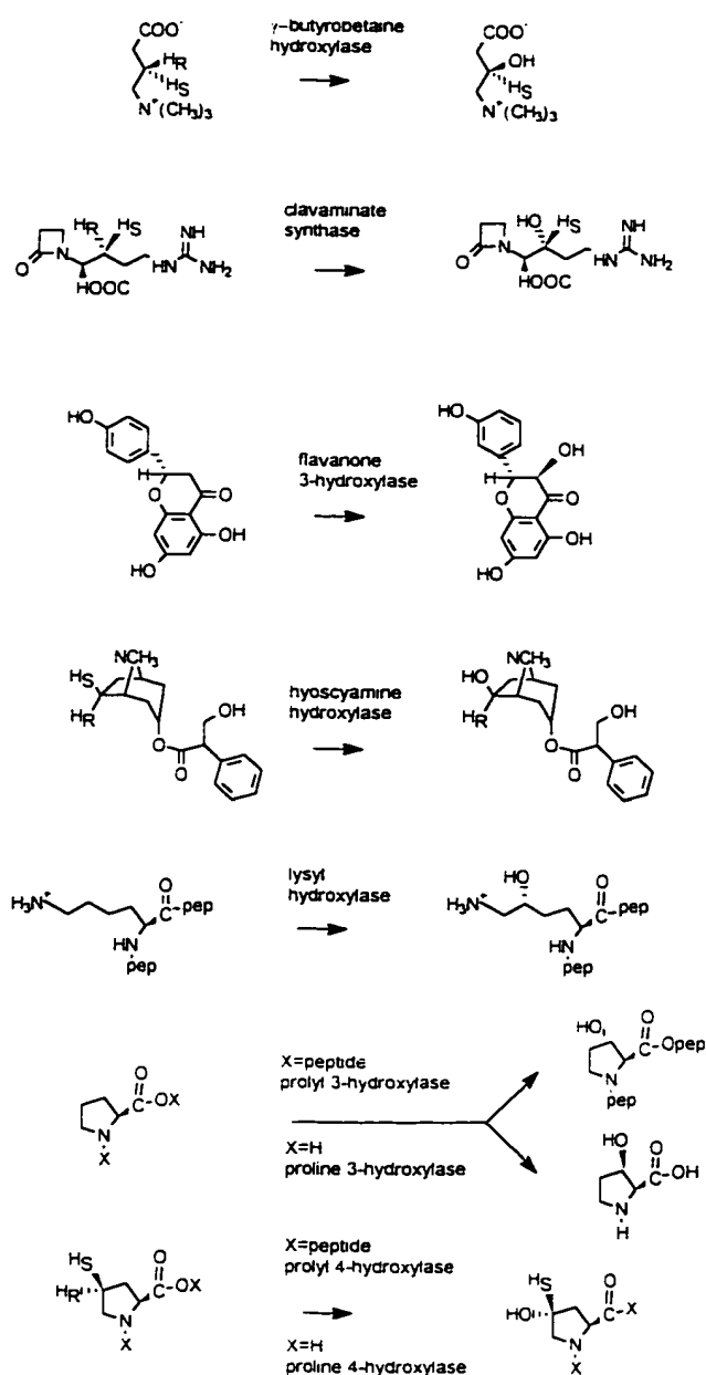
Figure 18. Stereospecificity of hydroxylations catalyzed by \alpha -KG-dependent dioxygenases.
