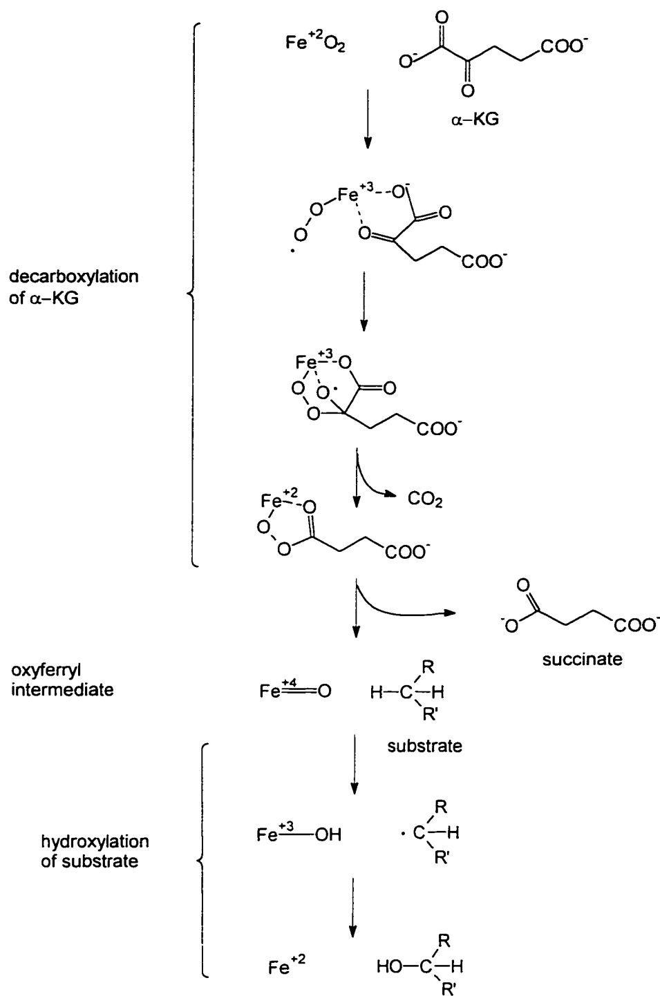
Scheme 9. Oxyferryl mechanism for \alpha -KG-dependent dioxygenases.
