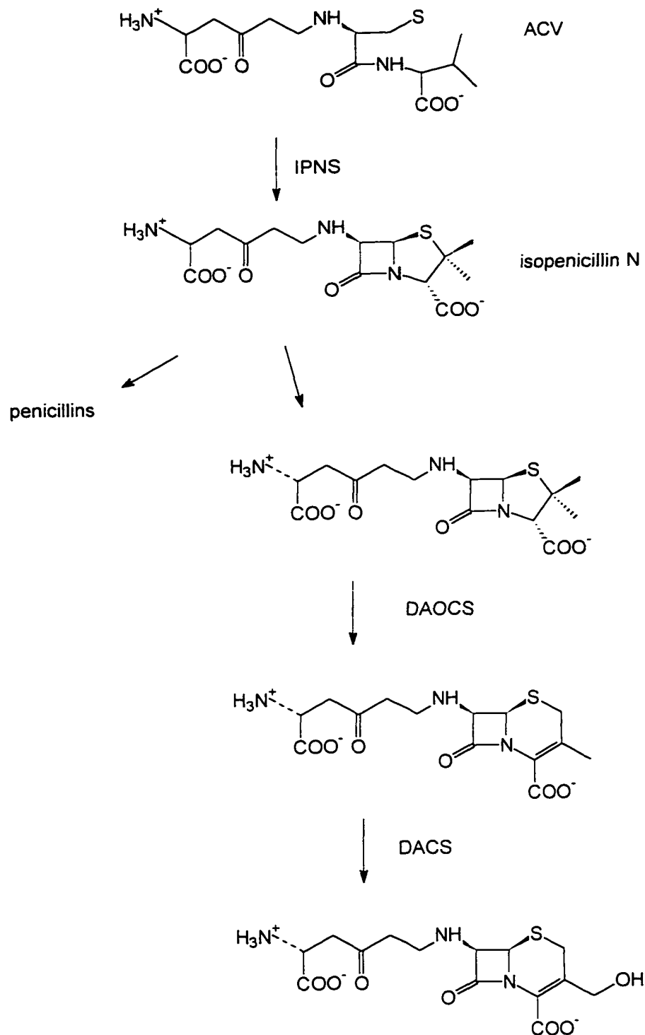
Scheme 5. Reactions catalyzed by IPNS, DAOCS and DACS.
