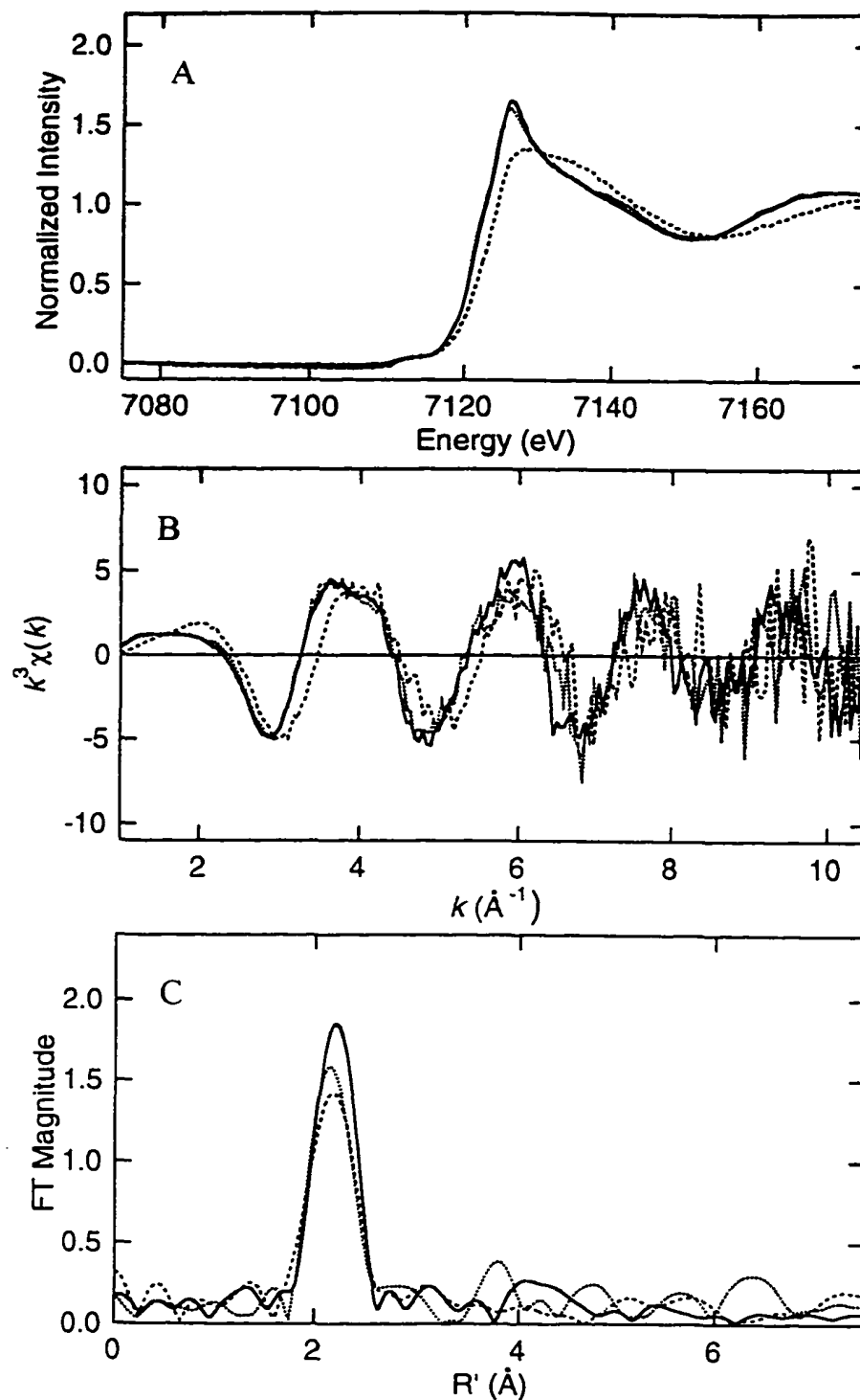
Figure 23. EXAFS spectra of resting and substrate-bound Fe-TfdA.
