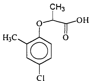
2-(2-methyl-4-chlorophenoxy)propionic acid Mecoprop
