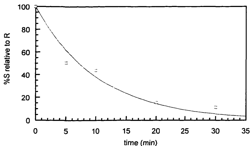
Figure 10. Loss of (S)-dichlorprop (relative to the R-enantiomer) catalyzed by TfdA.
