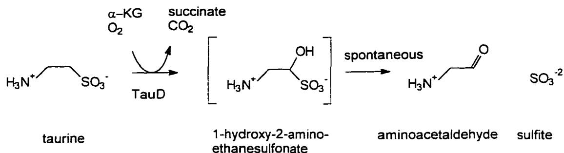
Scheme 7. Reaction catalyzed by TauD.
