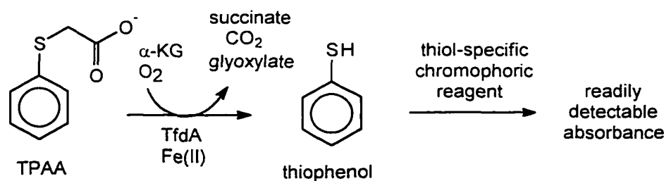
Scheme 12. Assay of TfdA using TPAA as a substrate
