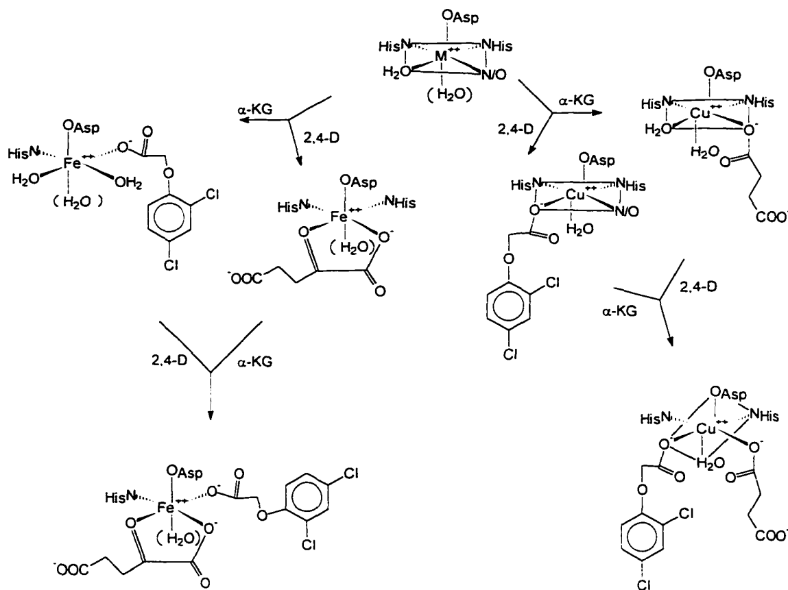
Figure 24. Proposed ligand identity and geometry for resting and substrate-bound TfdA.
