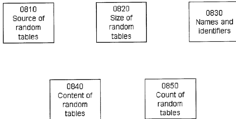
Figure 08: Random tables (0230)
