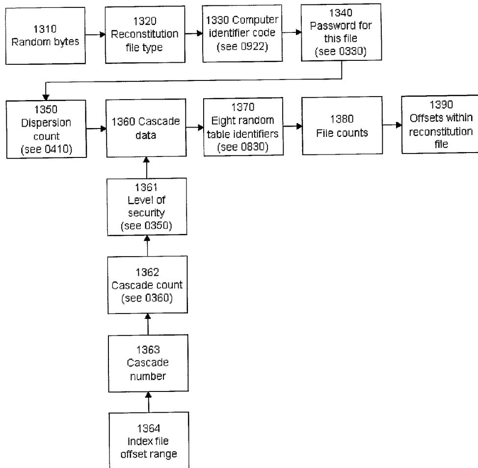
Figure 13: Reconstitution header (1250)
