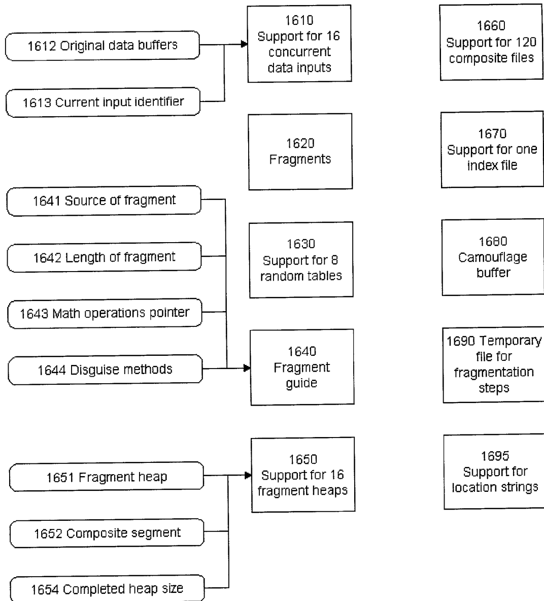
Figure 16: Intermediate objects (0280)
