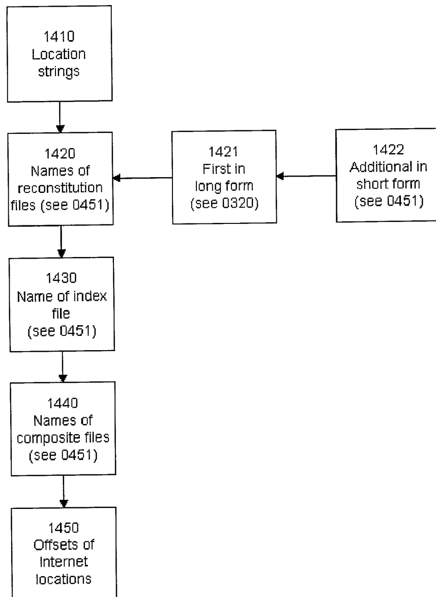
Figure 14: Reconstitution body (1260)
