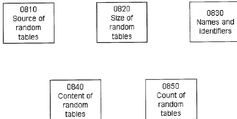
Figure 08: Random tables (0230)
