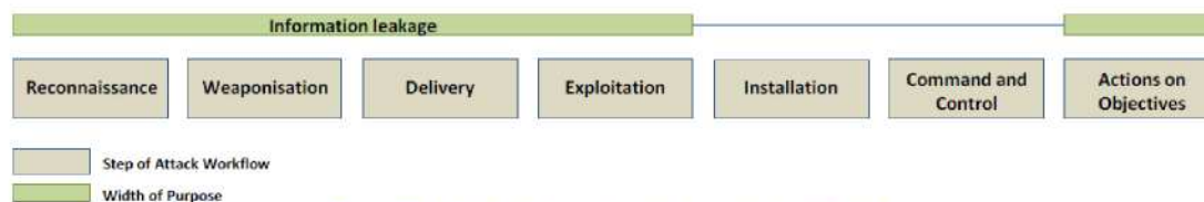
Figure 30: Position information leakage in the kill-chain
