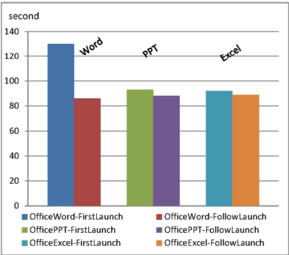
Fig. 10. Lengths of the unsmooth periods
