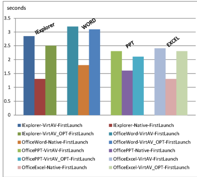
Fig. 11. a) performance comparison on the first launches
