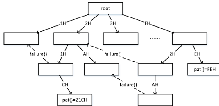
Fig. 4. An example trie built from memory signatures
