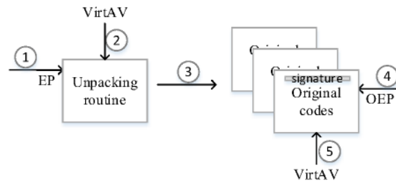
Fig. 6. virus scan for packed virus
