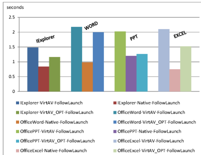
Fig. 11. b) performance comparison on the subsequent launches
