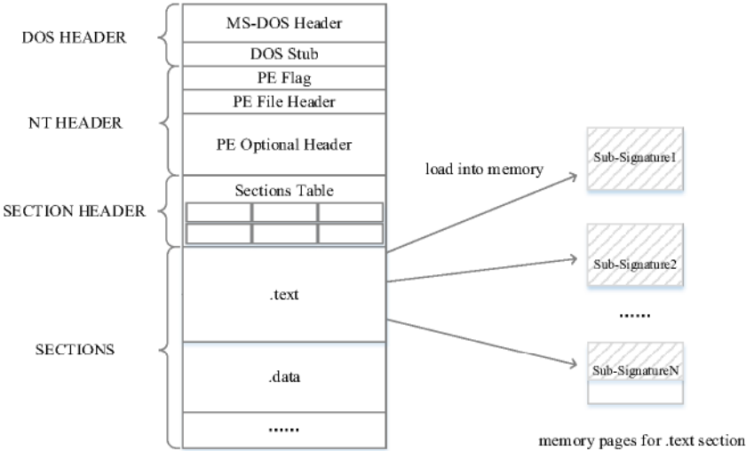
Fig. 2. Memory signature for virus in PE format
