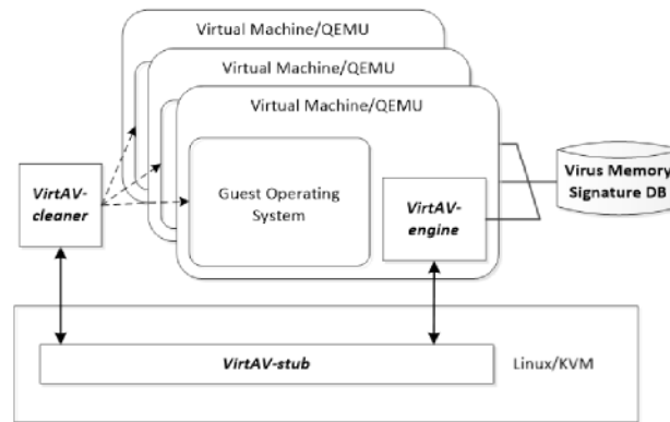
Fig. 1. Overall architecture of VirtAV
