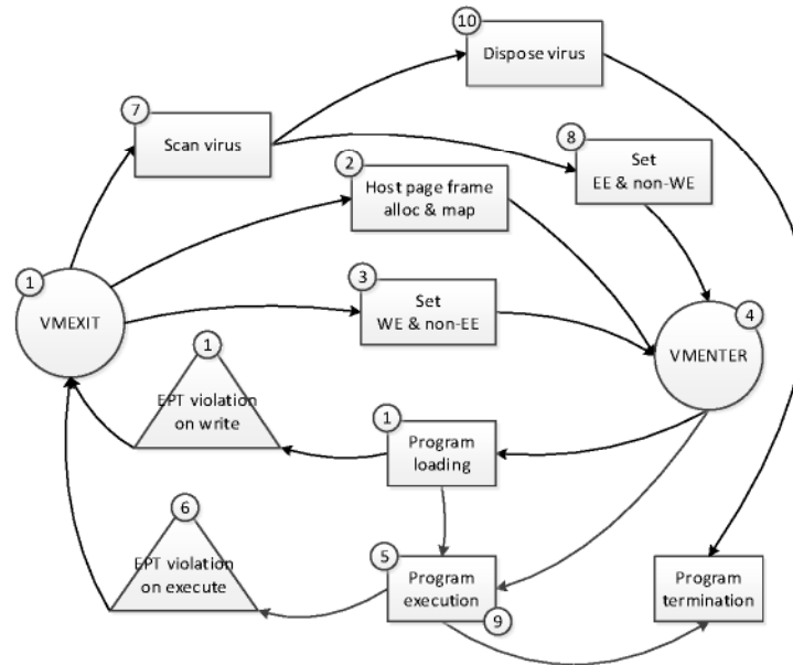
Fig. 5. Flow path of program execution in guest VM
