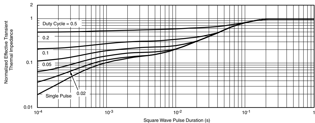
Normalized Thermal Transient Impedance, Junction-to-Source
