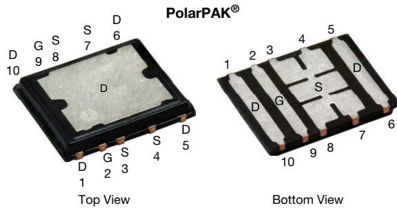
Top surface is connected to pins 1, 5, 6, and 10
