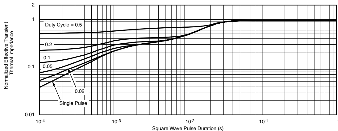
Normalized Thermal Transient Impedance, Junction-to-Case (Drain Top)
