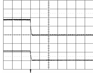
Shut-down enabled by disconnecting V_i at: T_{ref} = +25^{\circ}\text{C} , V_i = 53\text{ V} , I_O = 33\text{ A} resistive load.
