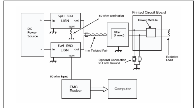
Test set-up
