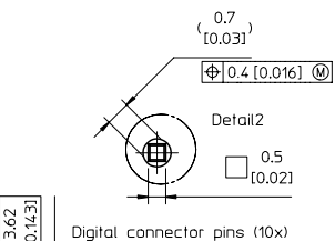
Digital connector pins (10x)
