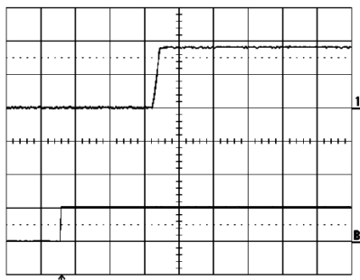
Start-up enabled by connecting V_I at: T_{ref} = +25^{\circ}\text{C} , V_I = 53\text{ V} , I_O = 33\text{ A} resistive load.
