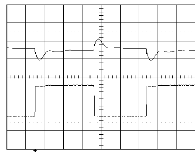
Output voltage response to load current step-Top trace: output voltage (0.5 V/div.). change (8.25-24.75-8.25 A) at: T_{ref} = +25^{\circ}\text{C} , V_I = 53\text{ V} . Bottom trace: output current (10A/div.). Time scale: (0.5 ms/div.).
