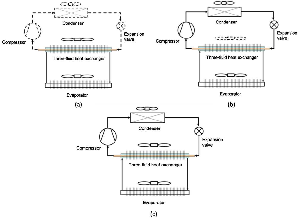
Fig. 21. Configurations of the three-fluid heat exchanger [40].
