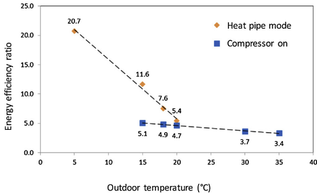
Fig. 24. Energy efficiency ratio against outdoor temperature.
