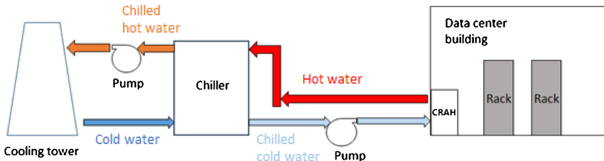
Fig. 10. Chiller bypass via heat exchanger economizer mode.
