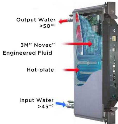
Fig. 13. Liquid-immersed module [27].
