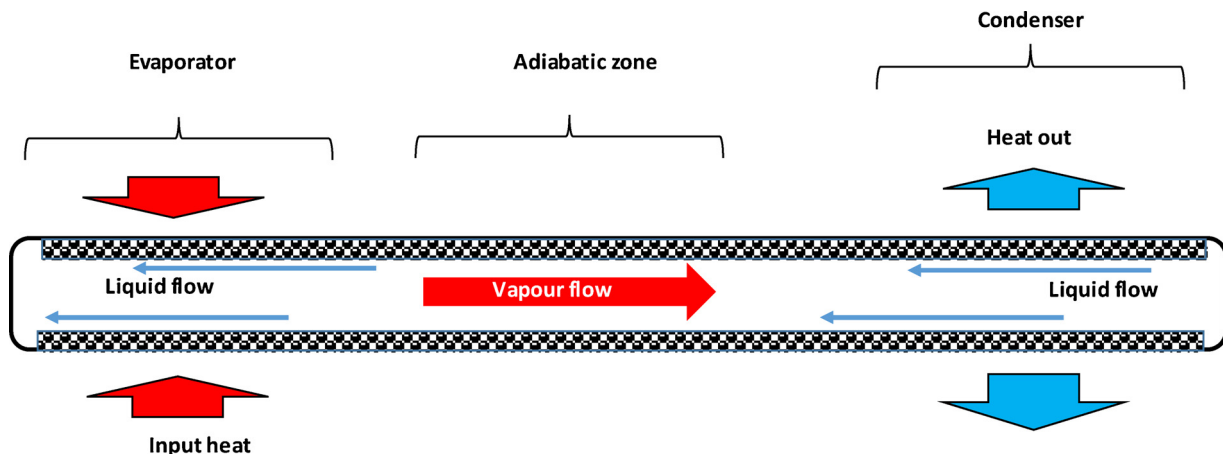
Fig. 14. Principle of the heat pipe.
