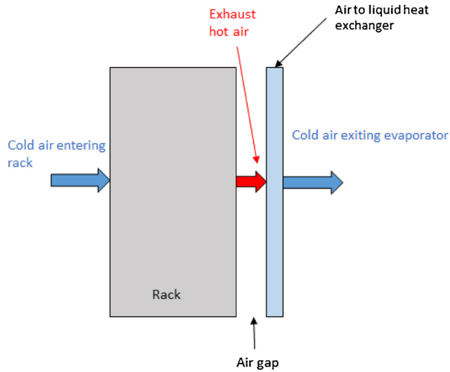
Fig. 12. Rack-level liquid cooling.
