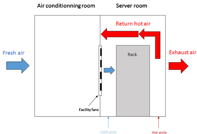
Fig. 27. Fresh-air container data center [47].
