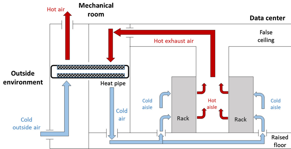
Fig. 15. Indirect free cooling unit with a heat pipe [36].
