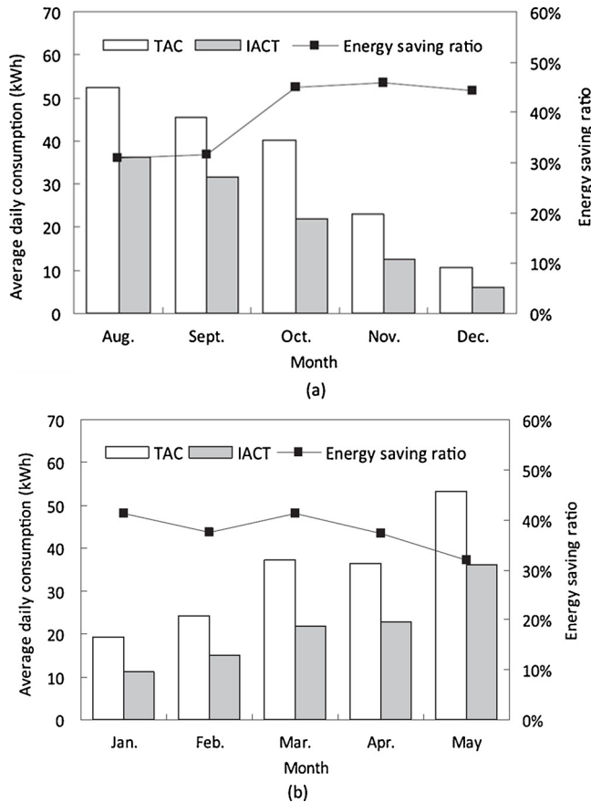
Fig. 20. Energy consumption in two mobile stations: (a) August to December; (b) January to May.
