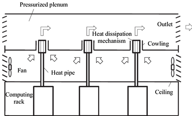
Fig. 16. Heat pipe thermosyphon [21].
