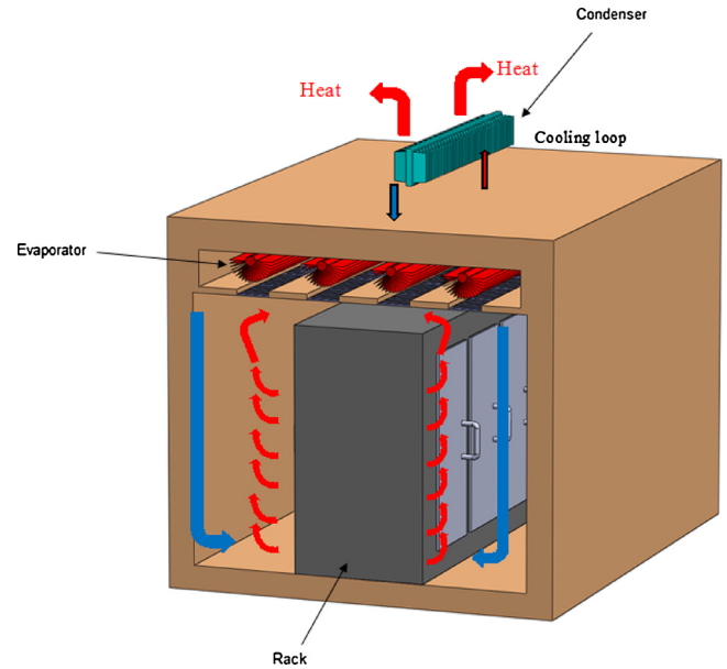
Fig. 18. Experimental setup of a two-phase thermosyphon loop.
