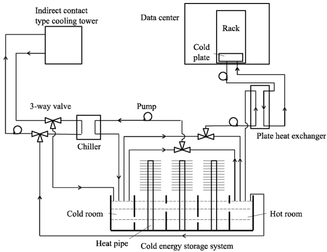
Fig. 17. Pipe based cold storage system combined with a chilled-cooling tower [38].
