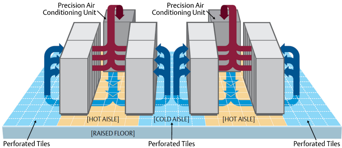
Fig. 5. Hot-aisle/cold-aisle configuration [16].
