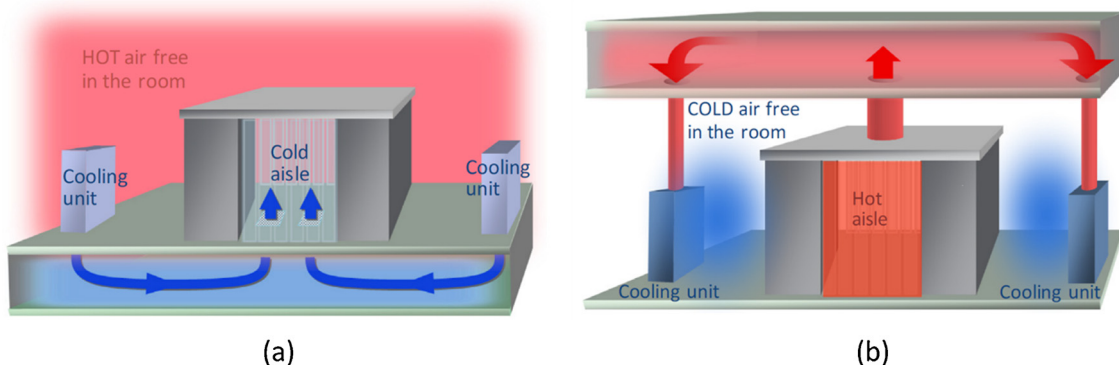
Fig. 6. Data center containment: (a) cold aisle containment; (b) hot aisle containment [17].
