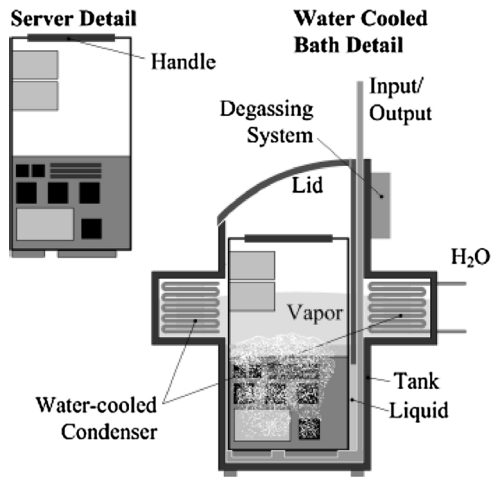
Fig. 26. Water-cooled open bath immersion concept [46].
