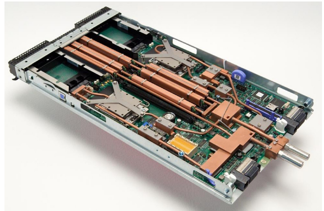
Fig. 11. Water cooled IBM blade center [29].
