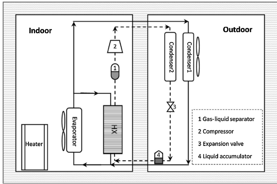
Fig. 23. Integrated system with a plate HX [42].
