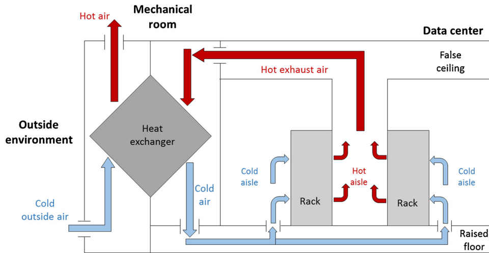
Fig. 9. Air-to-air heat exchanger for cooling data centers.
