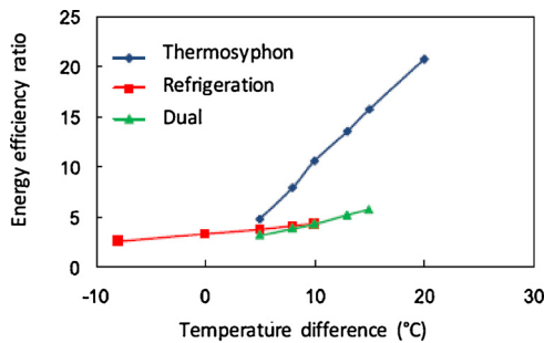
Fig. 22. Energy efficiency ratio against temperature difference.
