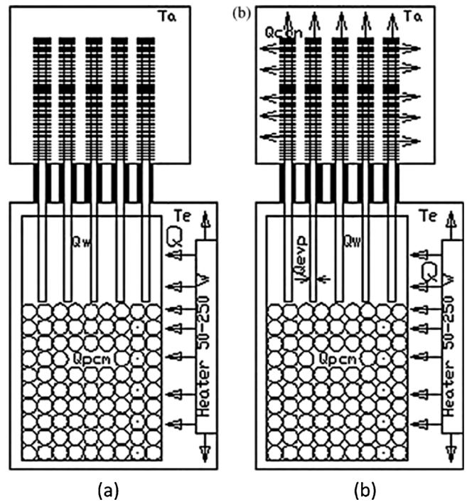
Fig. 28. Passive cooling system combining PCM and two-phase closed thermosyphon [50].
