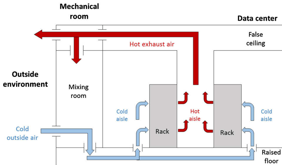
Fig. 8. Direct airside economizer.
