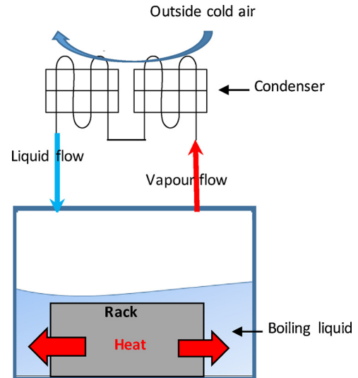
Fig. 25. Immersion cooling process.
