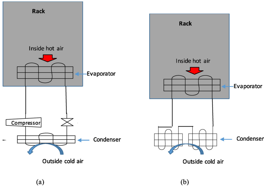
Fig. 19. Integrated air conditioner with thermosyphon: (a) vapor compression mode; (b) thermosyphon mode.
