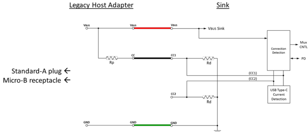
Figure 4-27 Legacy Host Port to Sink Functional Model
