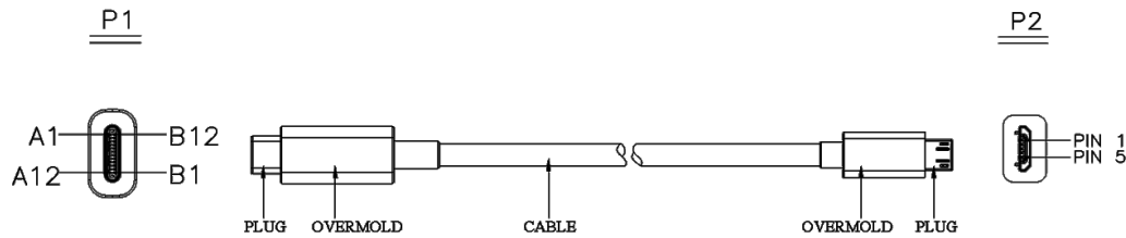
Figure 3-28 USB Type-C to USB 2.0 Micro-B Cable Assembly
