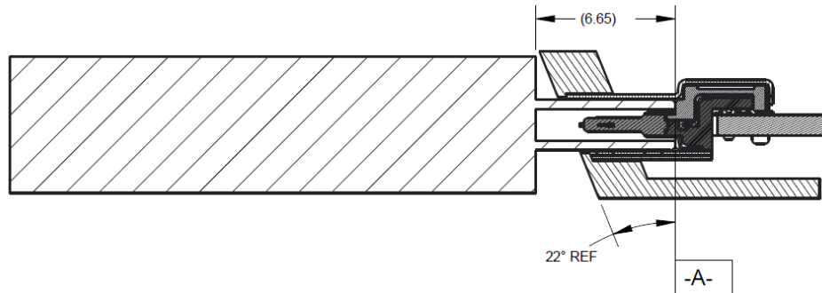
Figure 3-72 Cable Plug Overmold and an Angled Surface
