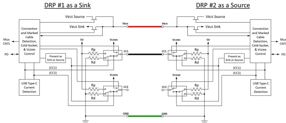
Figure 4-23 DRP to DRP Functional Model – CASE 2 & 3
