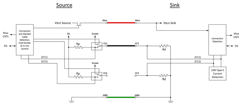
Figure 4-19 Source to Sink Functional Model
