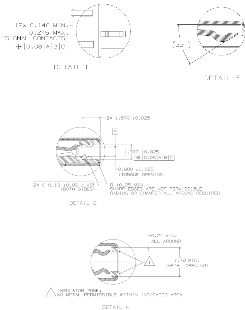
Figure 3-9 USB 2.0 Type-C Plug Interface Dimensions, cont.
