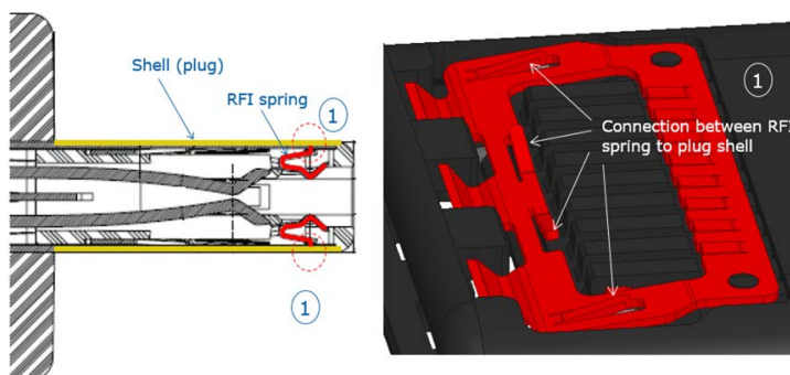
Figure 3-67 EMC Finger Connections to Plug Shell
