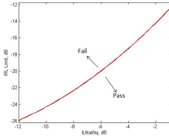
Figure 3-39 IRL Limit as Function of ILfitatNq
