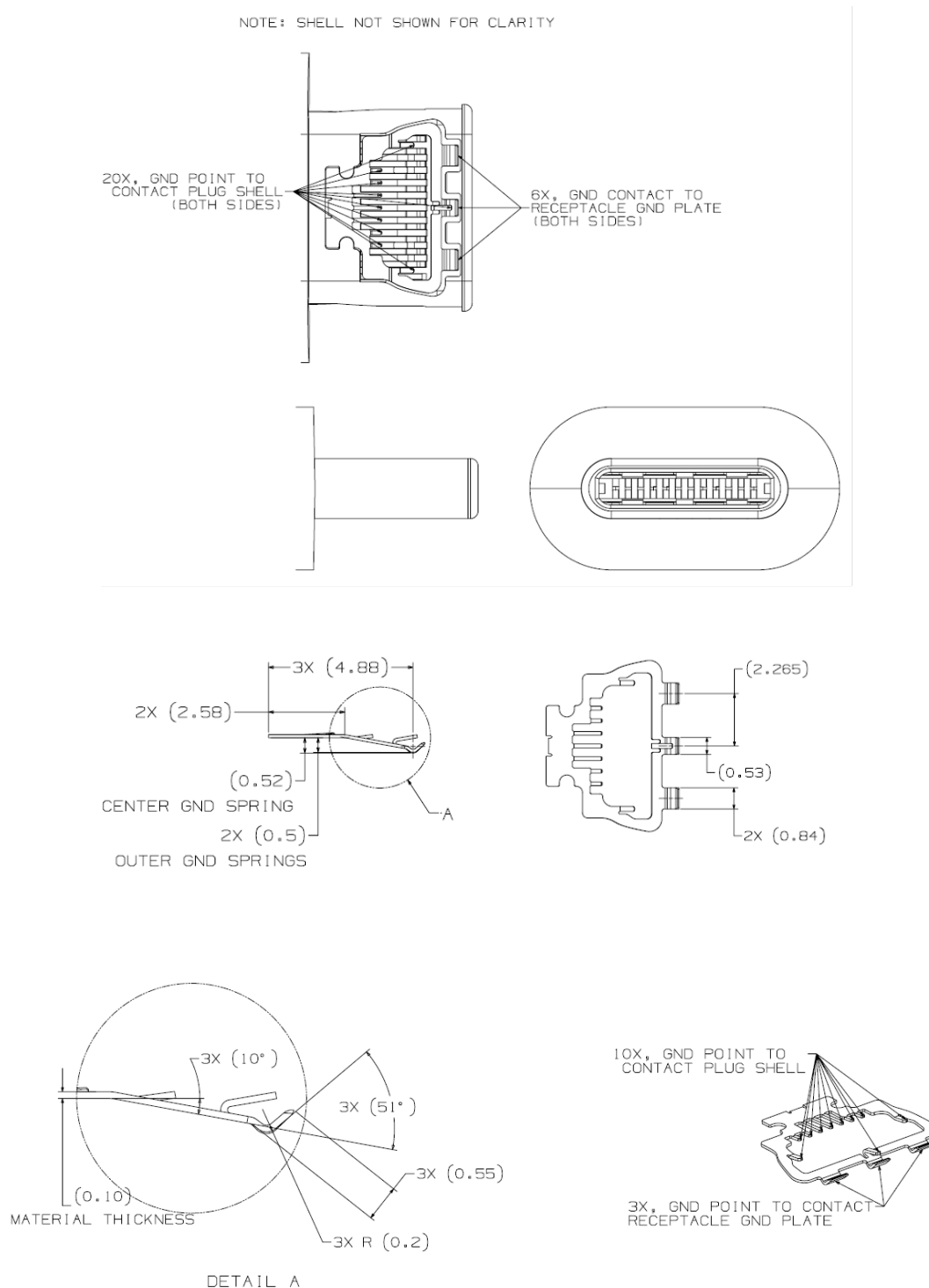
Figure 3-14 Reference Design of the USB Full-Featured Type-C Plug Internal EMC Spring
