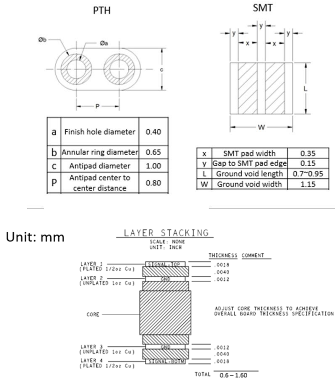
Figure 3-50 Recommended Ground Void Dimensions for USB Type-C Receptacle
