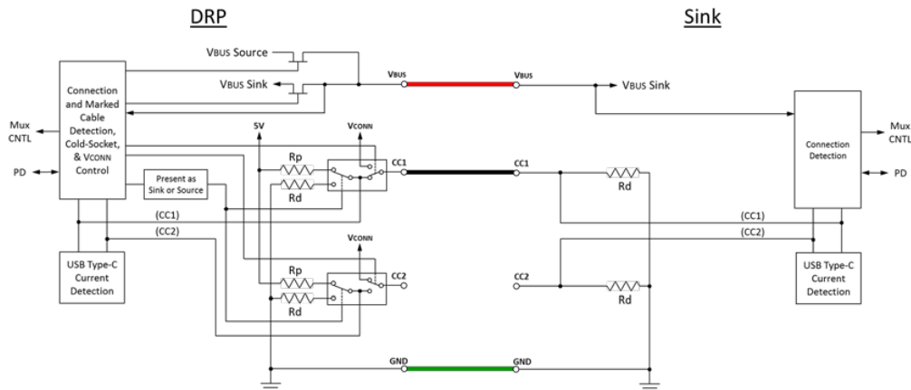
Figure 4-21 DRP to Sink Functional Model
