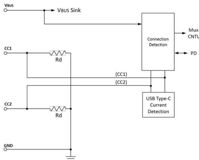
Figure 4-9 Sink Functional Model for CC1 and CC2
