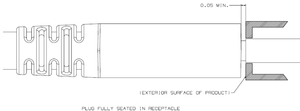
Figure 3-71 Recommended Minimum Plug Overmold Clearance
