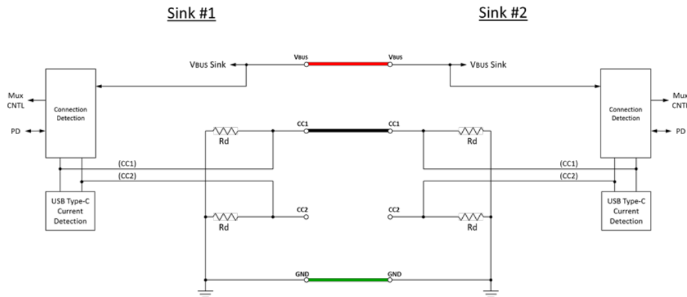
Figure 4-25 Sink to Sink Functional Model
