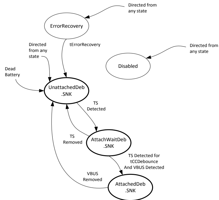
Figure B-4 Connection State Diagram: DTS Sink
