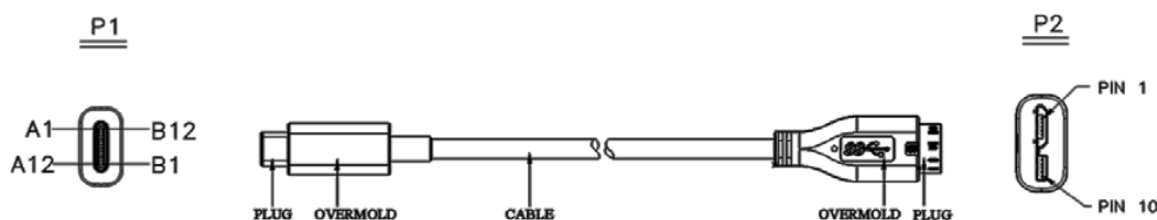
Figure 3-27 USB Type-C to USB 3.1 Micro-B Cable Assembly
