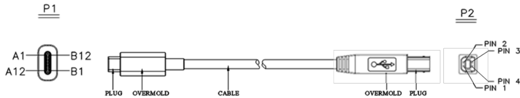
Figure 3-25 USB Type-C to USB 2.0 Standard-B Cable Assembly
