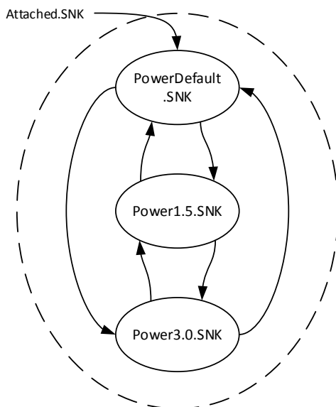
Figure 4-18 Sink Power Sub-States
