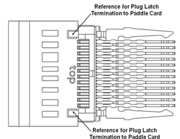
Figure 3-13 Illustration of the Latch Soldered to the Paddle Card Ground
