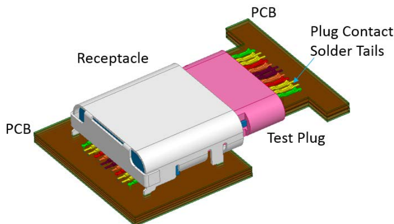
Figure 3-48 Illustration of USB Type-C Mated Connector
