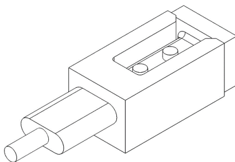
Figure 3-64 Wrenching Strength Test with Cable in Fixture
