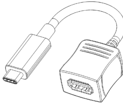
Figure 3-29 USB Type-C to USB 3.1 Standard-A Receptacle Adapter Assembly
