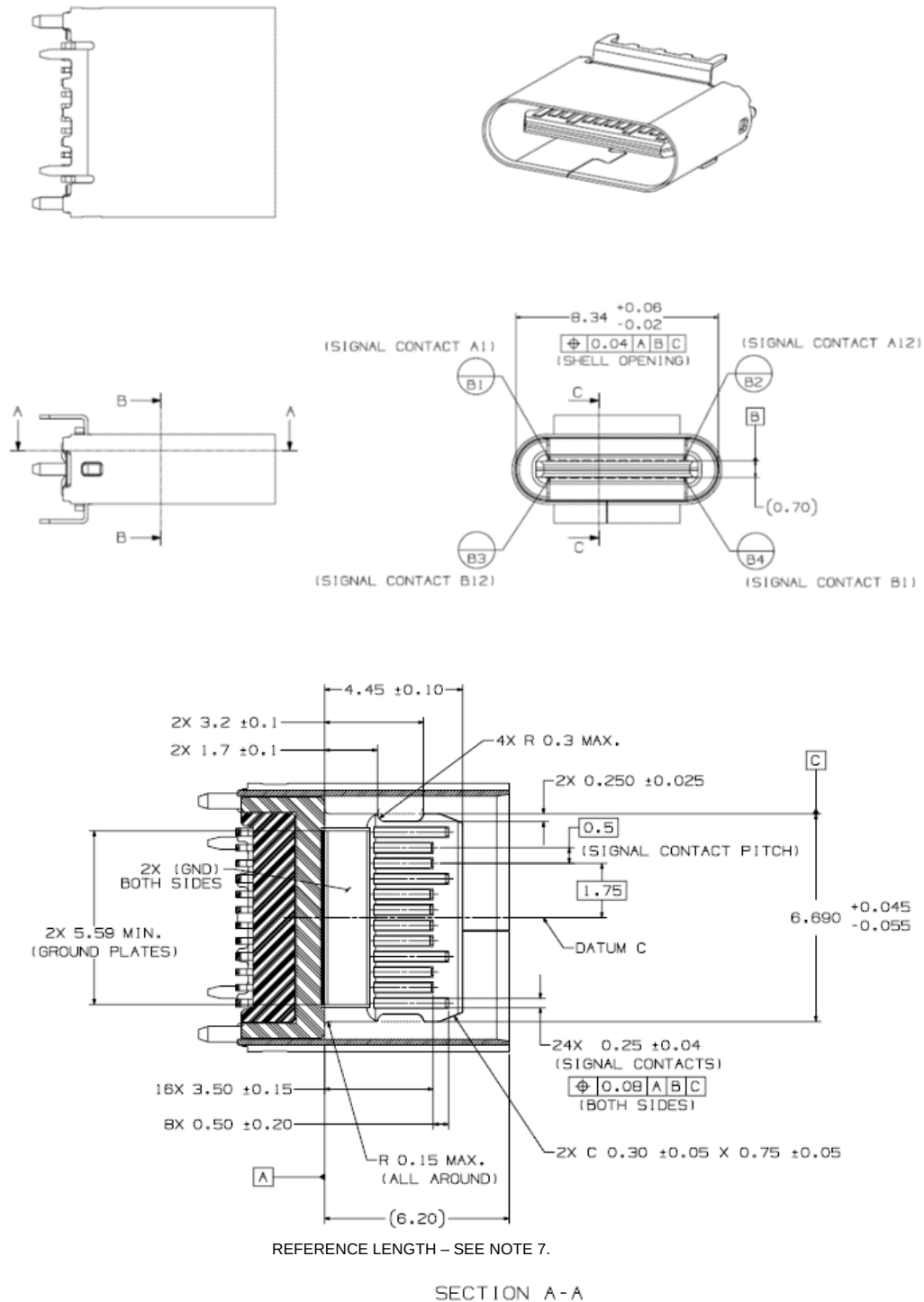
Figure 3-1 USB Type-C Receptacle Interface Dimensions
