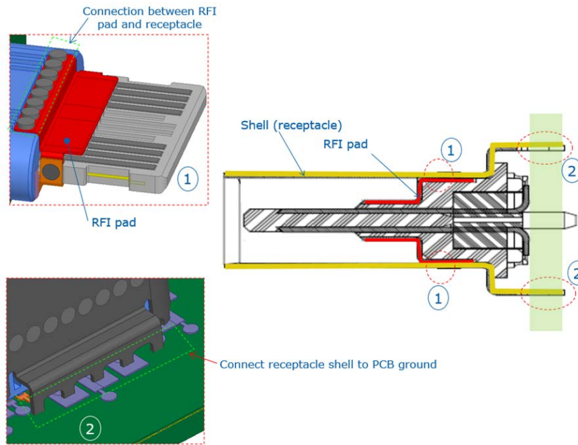
Figure 3-68 EMC Pad Connections to Receptacle Shell
