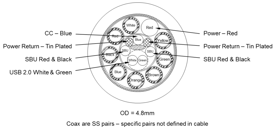
Figure 3-20 Illustration of a USB Full-Featured Type-C Cable Cross Section, a Coaxial Wire Example without VCONN
