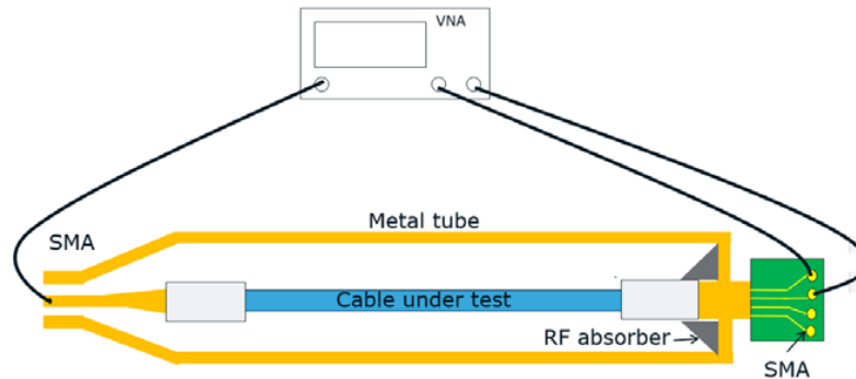
Figure 3-55 Cable Assembly Shielding Effectiveness Testing
