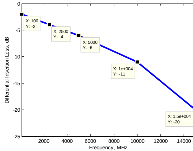
Figure 3-32 Recommended Differential Insertion Loss Requirement
