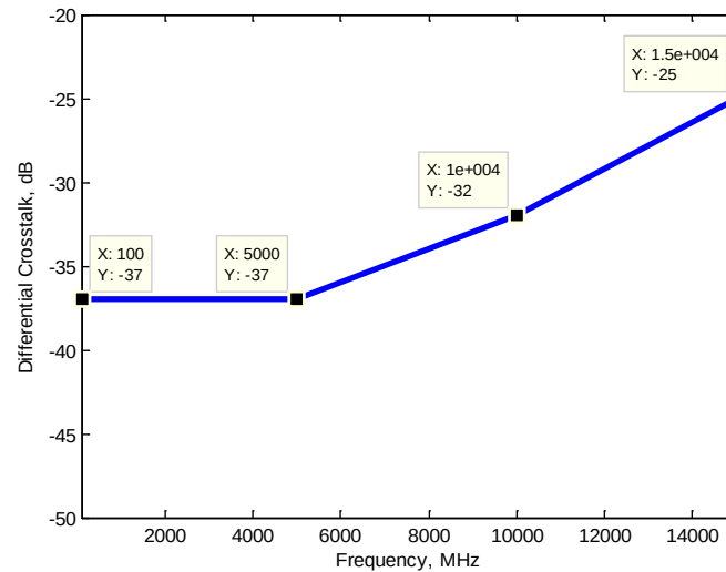
Figure 3-34 Recommended Differential Crosstalk Requirement
