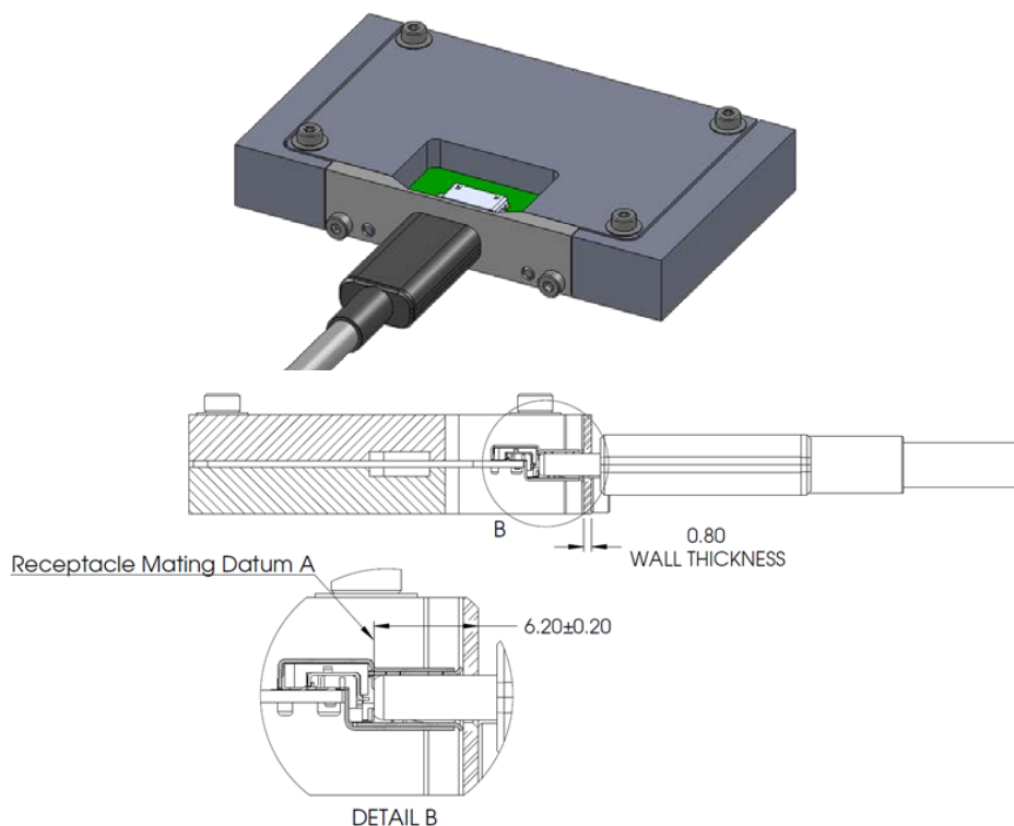
Figure 3-62 Reference Wrenching Strength Continuity Test Fixture
