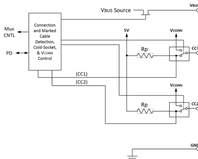
Figure 4-7 Source Functional Model for CC1 and CC2
