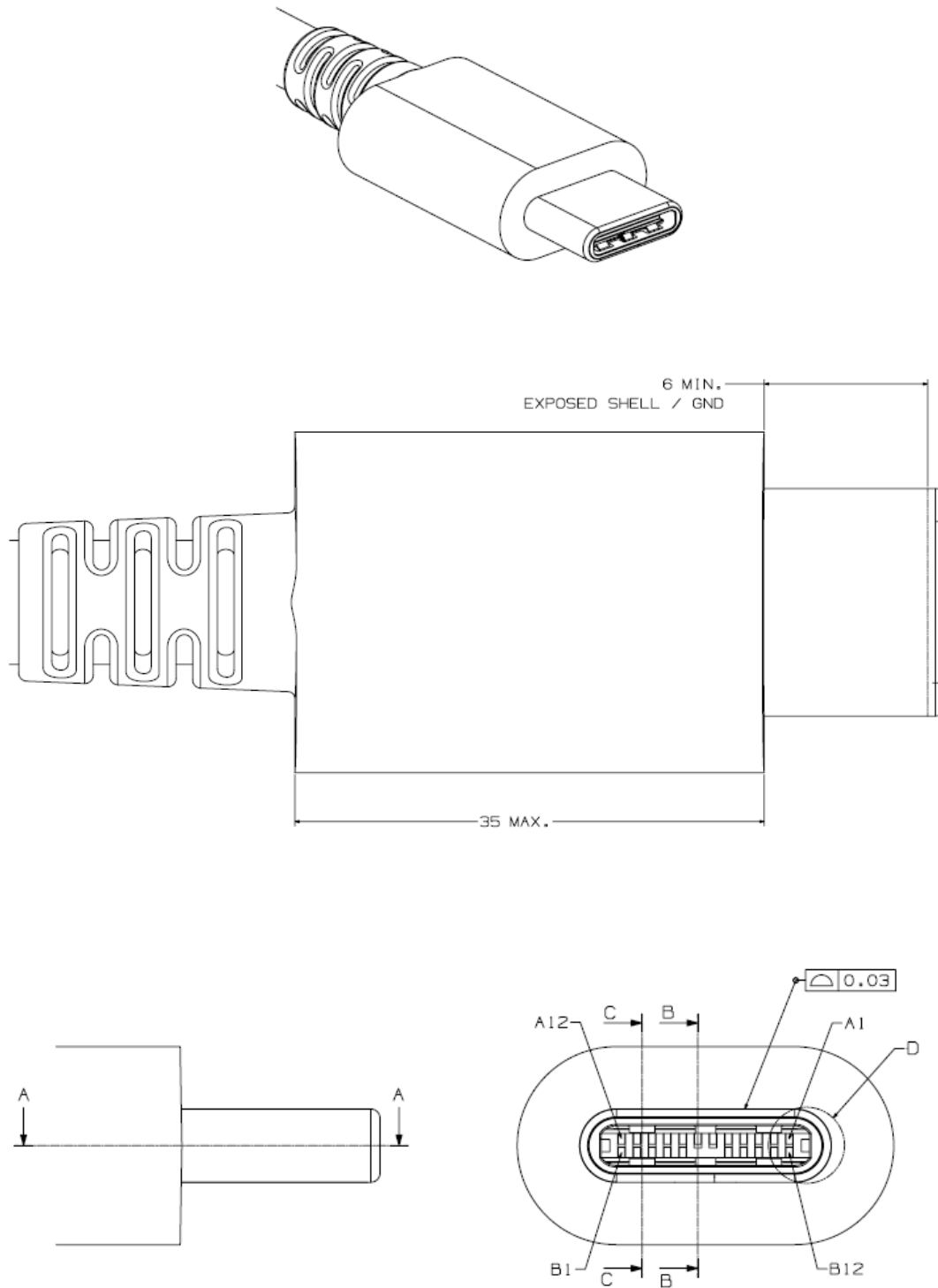
Figure 3-3 USB Full-Featured Type-C Plug Interface Dimensions
