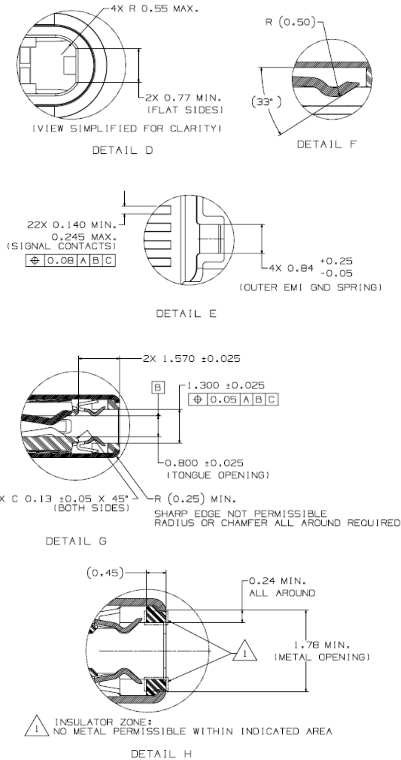
Figure 3-3 USB Full-Featured Type-C Plug Interface Dimensions, cont.
