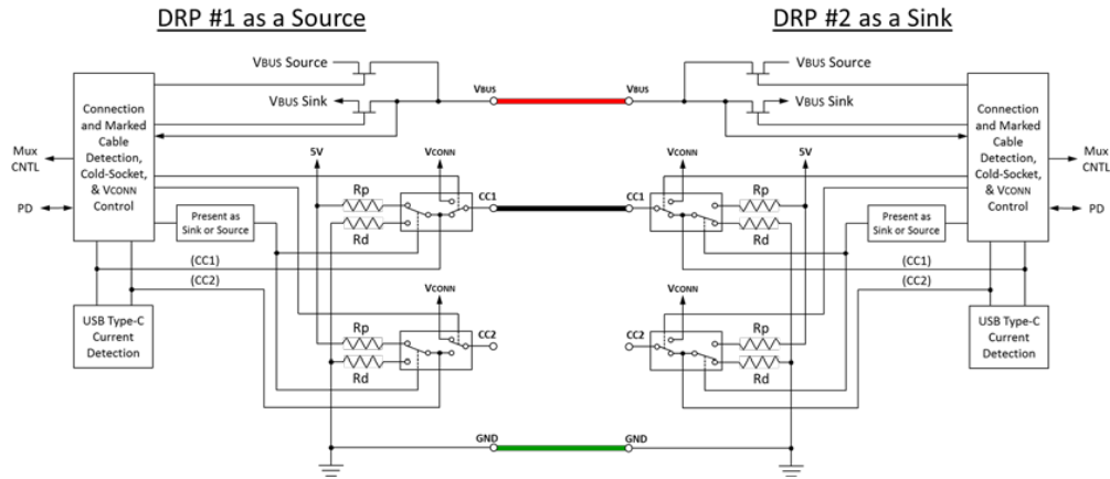
Figure 4-22 DRP to DRP Functional Model – CASE 1
