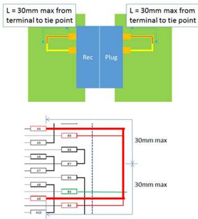
Figure 3-59 Example Current Rating Test Fixture Trace Configuration
