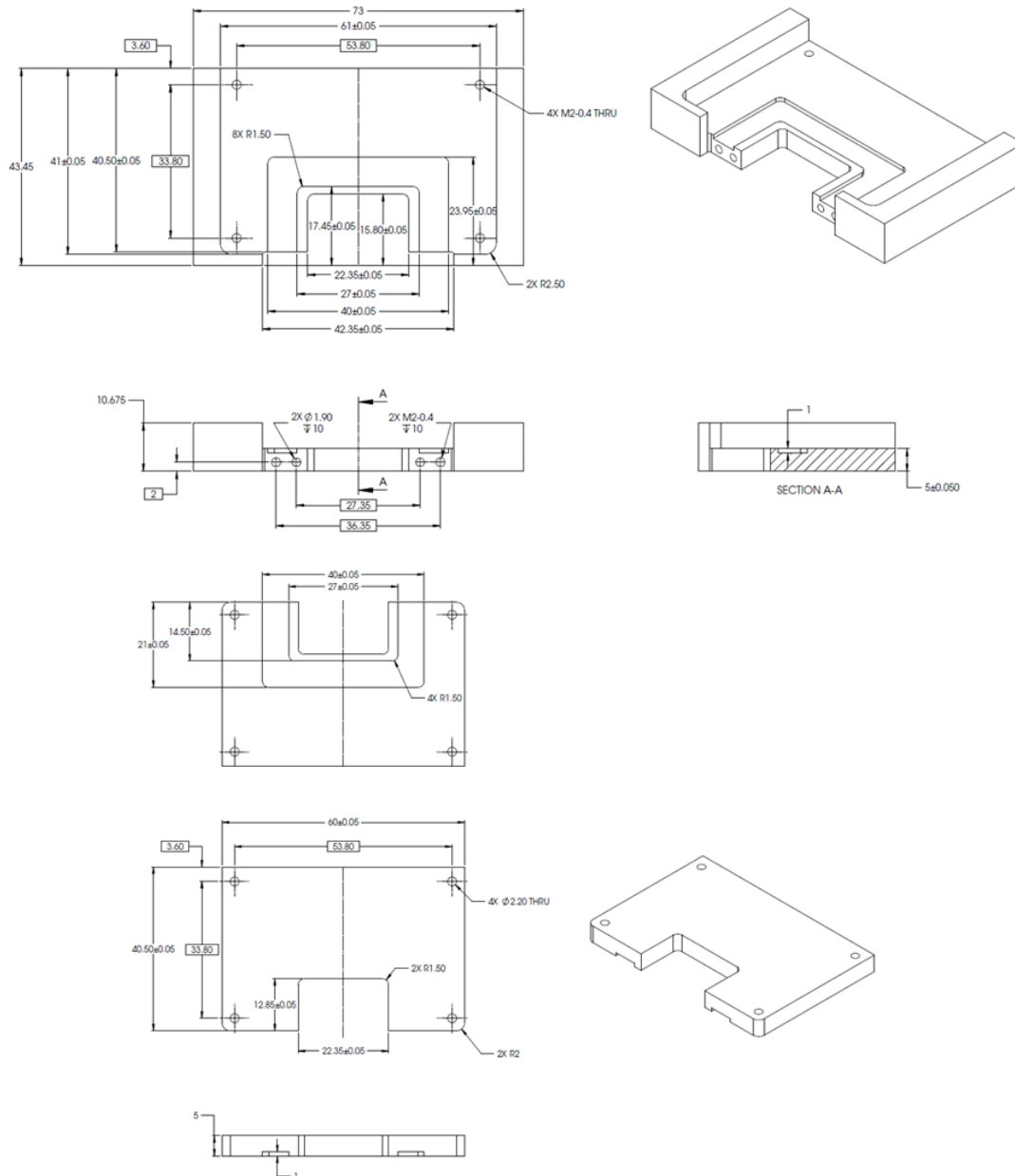
Figure 3-60 Example of 4-Axis Continuity Test Fixture
