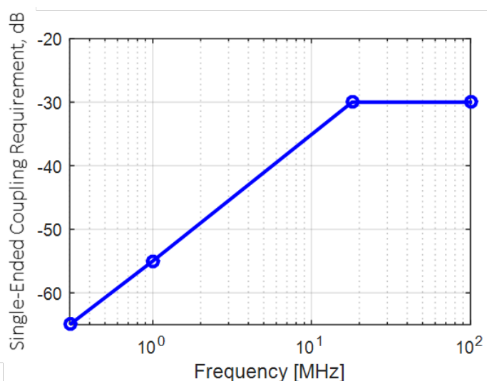
Figure 3-46 Requirement for Single-Ended Coupling between SBU_A/SBU_B and CC
