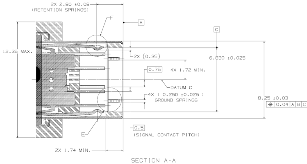
Figure 3-9 USB 2.0 Type-C Plug Interface Dimensions, cont.
