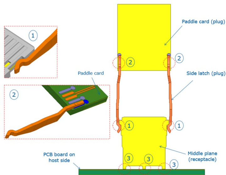
Figure 3-66 EMC Guidelines for Side Latch and Mid-plate
