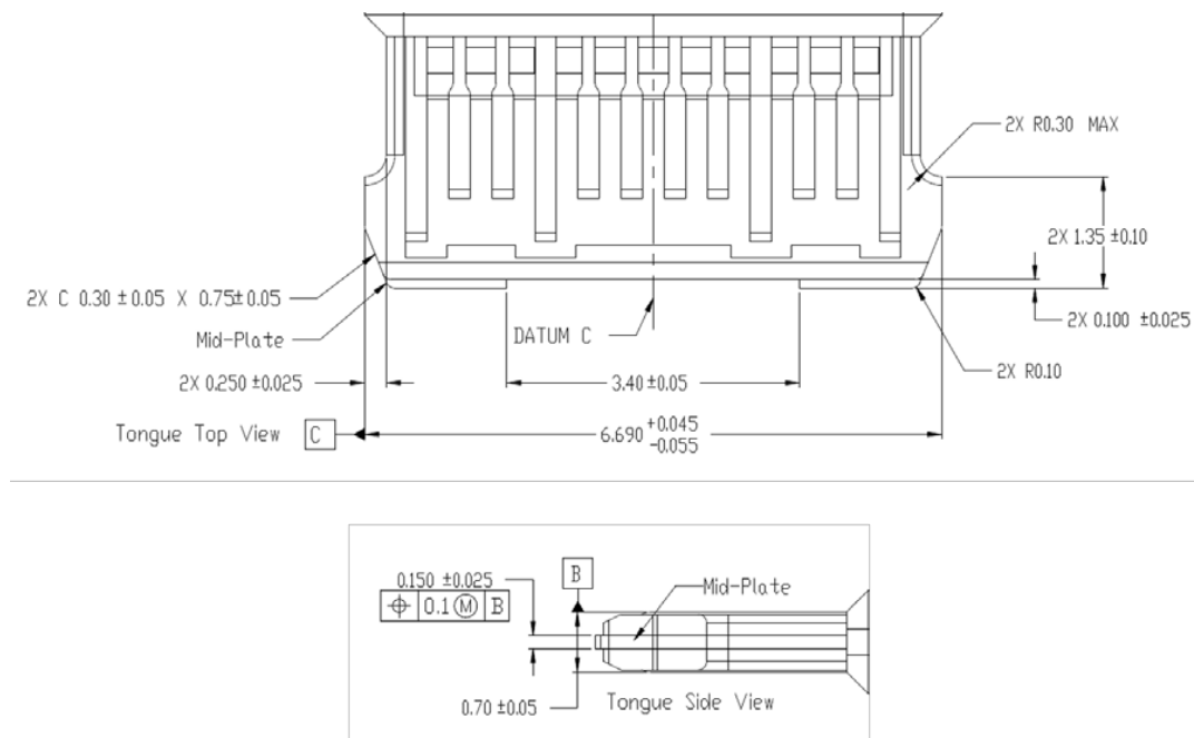
Figure 3-11 Reference Design of Receptacle Mid-Plate
