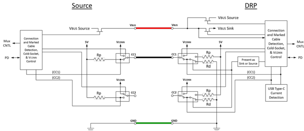
Figure 4-20 Source to DRP Functional Model
