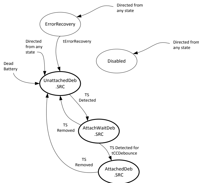
Figure B-3 Connection State Diagram: DTS Source
