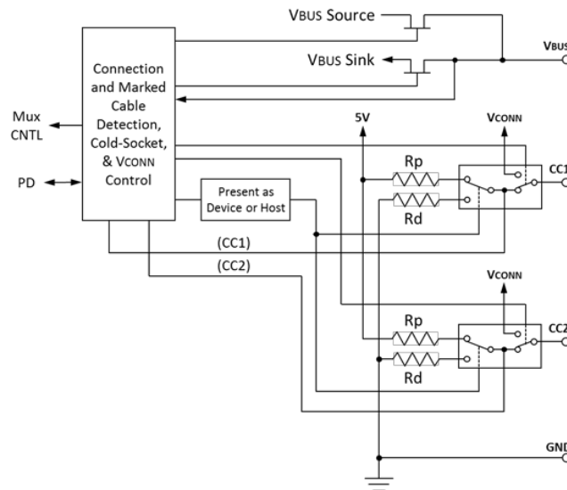
Figure 4-8 Source Functional Model Supporting USB PD PR_Swap
