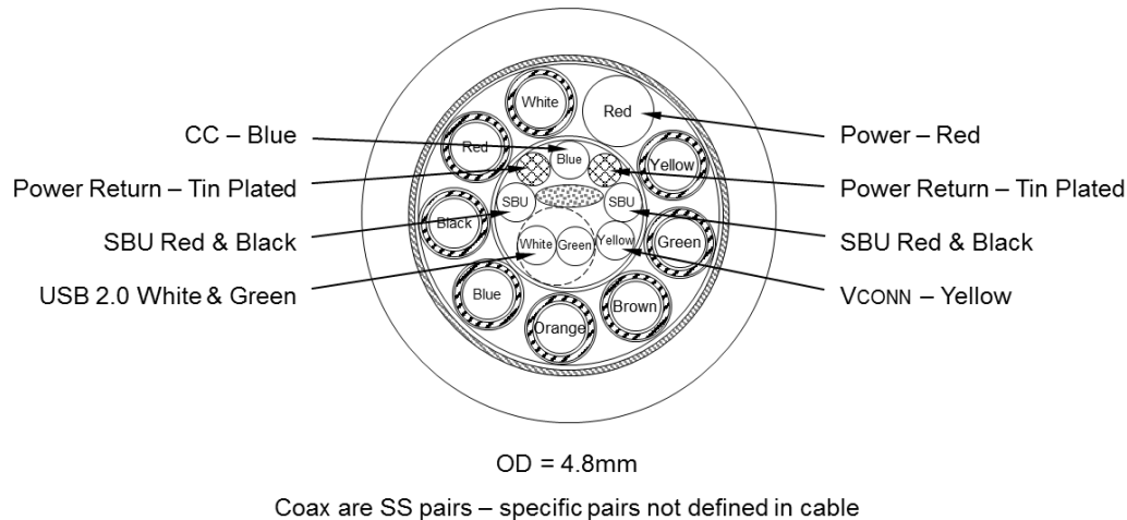
Figure 3-19 Illustration of a USB Full-Featured Type-C Cable Cross Section, a Coaxial Wire Example with VCONN
