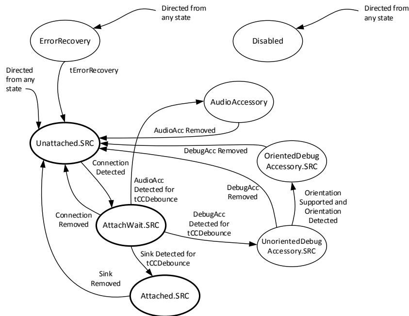
Figure 4-12 Connection State Diagram: Source
