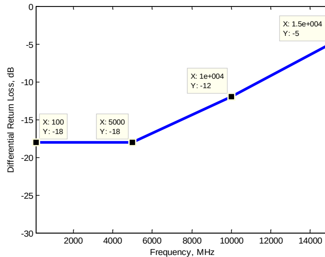
Figure 3-33 Recommended Differential Return Loss Requirement
