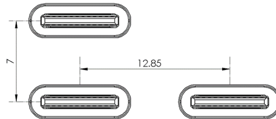
Figure 3-70 Recommended Minimum Spacing between Connectors
