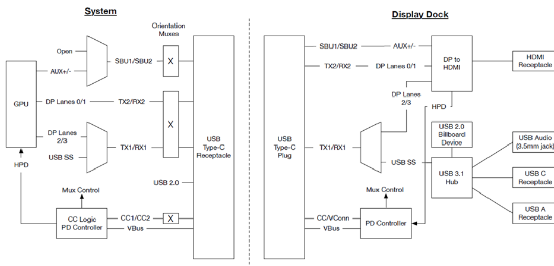
Figure 5-5 USB DisplayPort Dock Example
