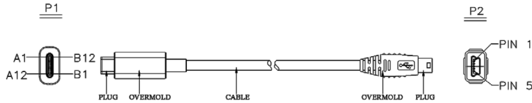
Figure 3-26 USB Type-C to USB 2.0 Mini-B Cable Assembly
