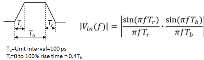
Figure 3-37 Input Pulse Spectrum
