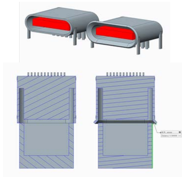
Figure 3-65 USB Type-C Cable Receptacle Flange Example
