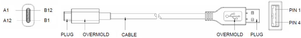
Figure 3-23 USB Type-C to USB 2.0 Standard-A Cable Assembly
