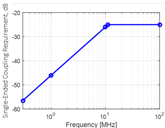
Figure 3-45 Requirement for Single-Ended Coupling between SBU_A and SBU_B
