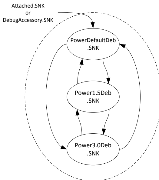
Figure B-6 TS Sink Power Sub-States
