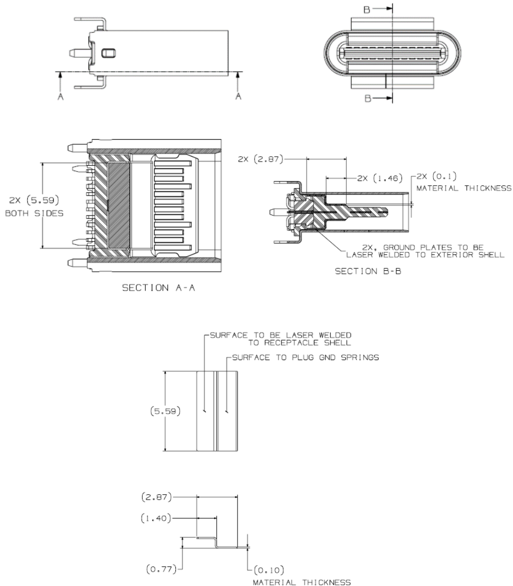
Figure 3-16 Reference Design of Internal EMC Pad
