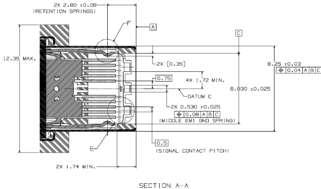
Figure 3-3 USB Full-Featured Type-C Plug Interface Dimensions, cont.
