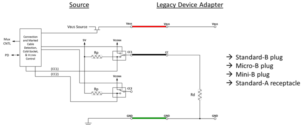
Figure 4-26 Source to Legacy Device Port Functional Model
