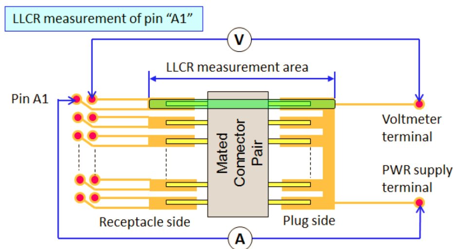
Figure 3-57 LLCR Measurement Diagram
