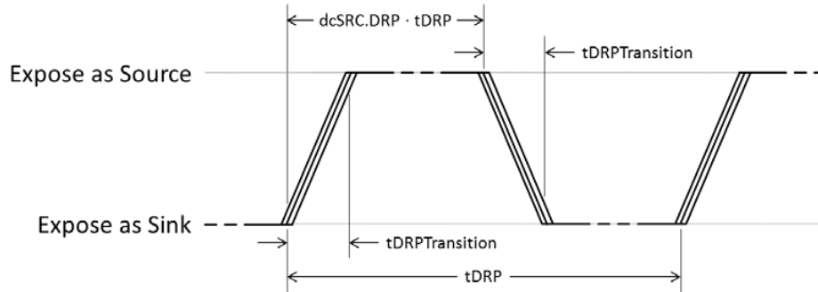
Figure 4-39 DRP Timing
