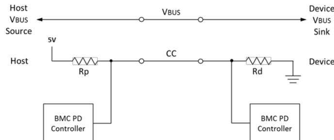
Figure 4-32 USB PD over CC Pins
