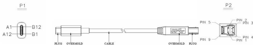
Figure 3-24 USB Type-C to USB 3.1 Standard-B Cable Assembly
