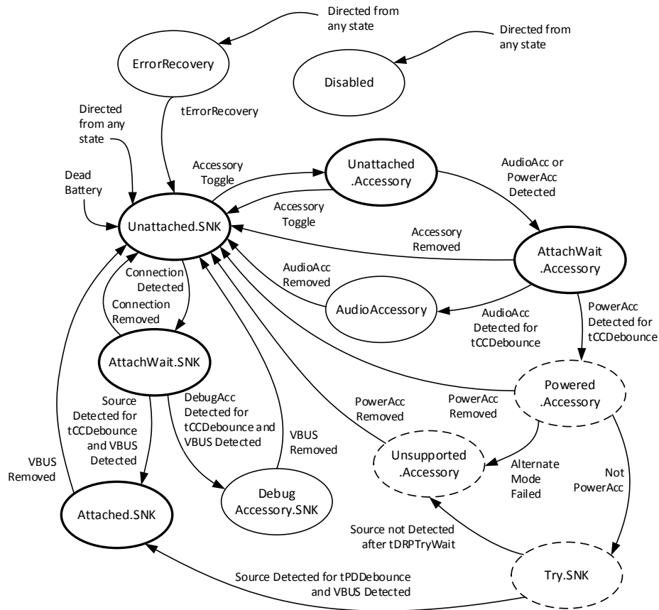
Figure 4-14 Connection State Diagram: Sink with Accessory Support
