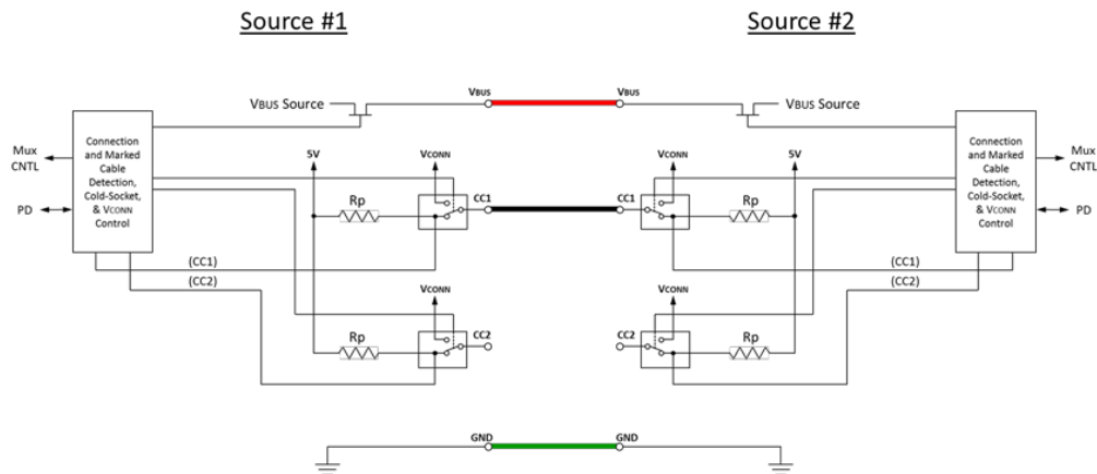
Figure 4-24 Source to Source Functional Model
