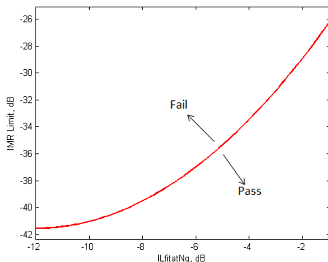
Figure 3-38 IMR Limit as Function of ILfitatNq
