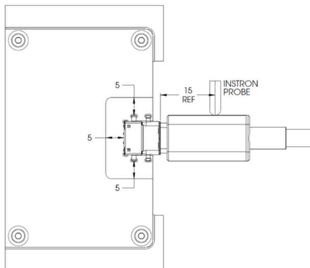
Figure 3-60 Example of 4-Axis Continuity Test Fixture, cont.
