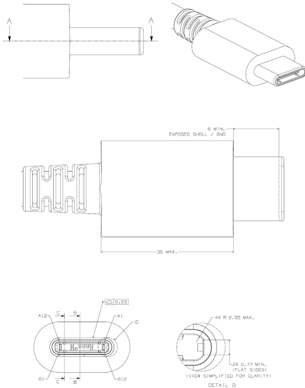
Figure 3-9 USB 2.0 Type-C Plug Interface Dimensions
