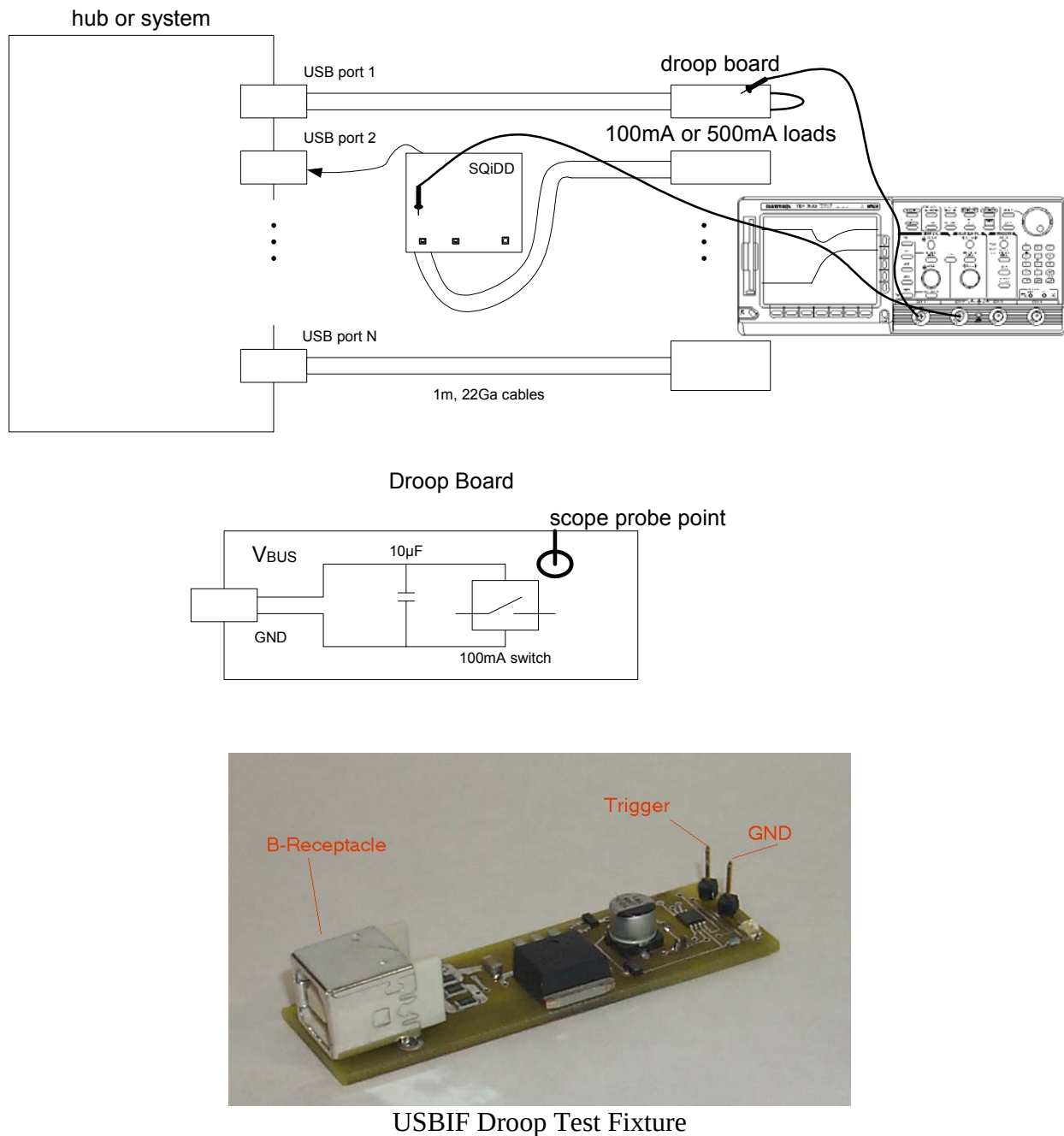
Figure B-4: Droop Test Setup & Fixture
