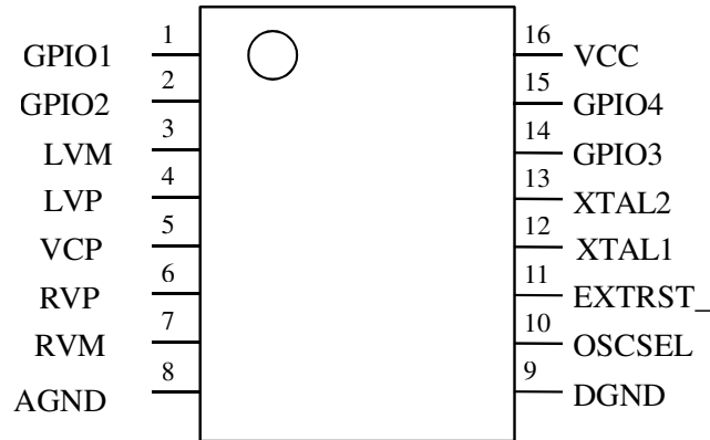
16-pin SOP
