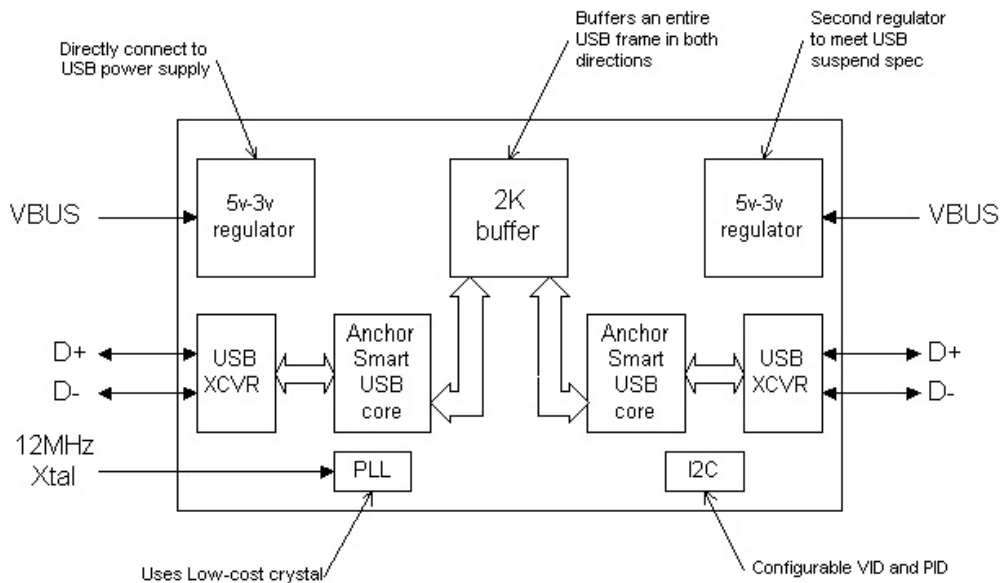
AN2720SC Block Diagram System Application
