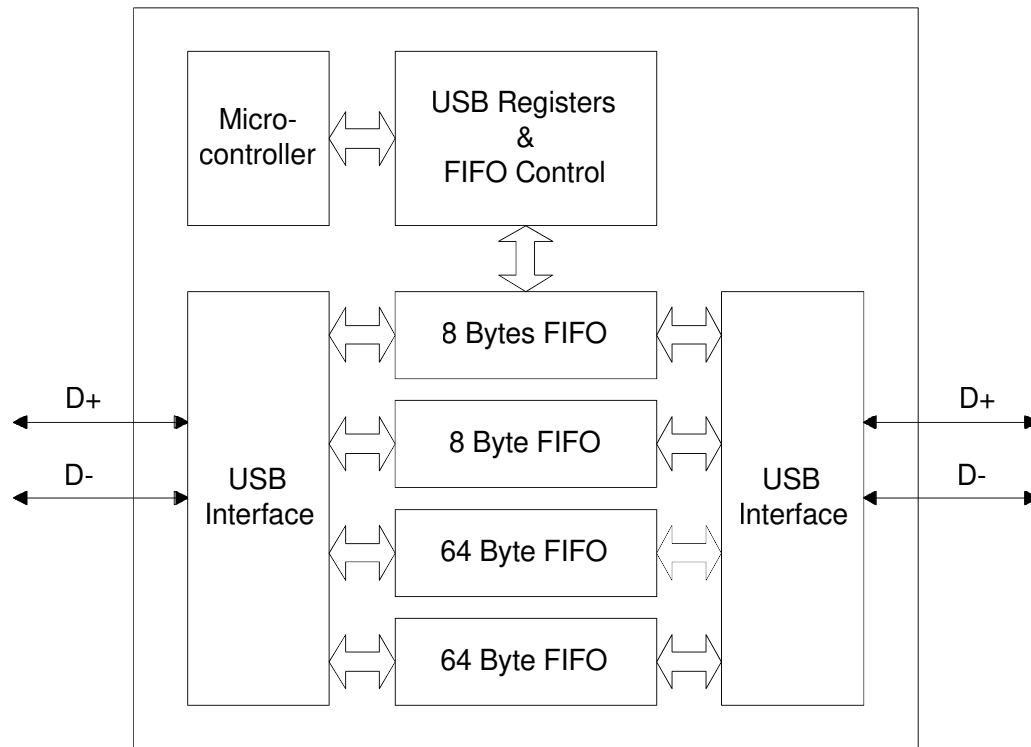
Block diagram of GL620USB-A
