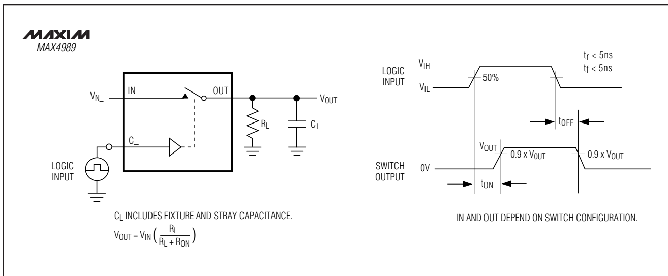
Figure 2. Switching Time
