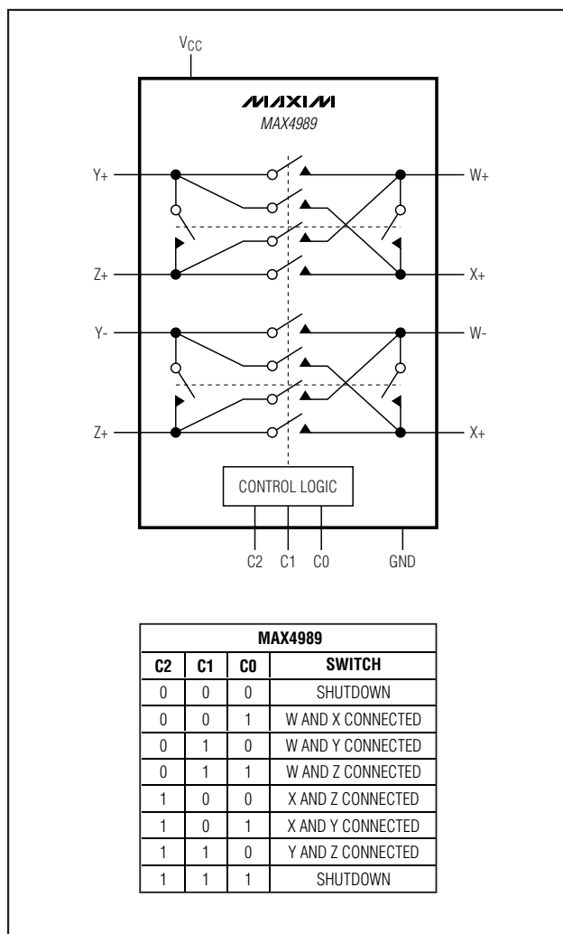
Figure 4. Typical Application Circuit
