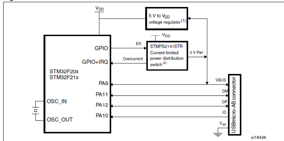
Figure 344. OTG A-B device connection
