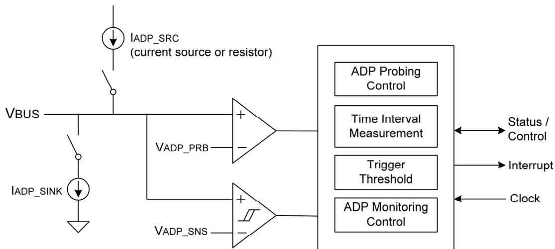
Figure 5-5: ADP Architecture
