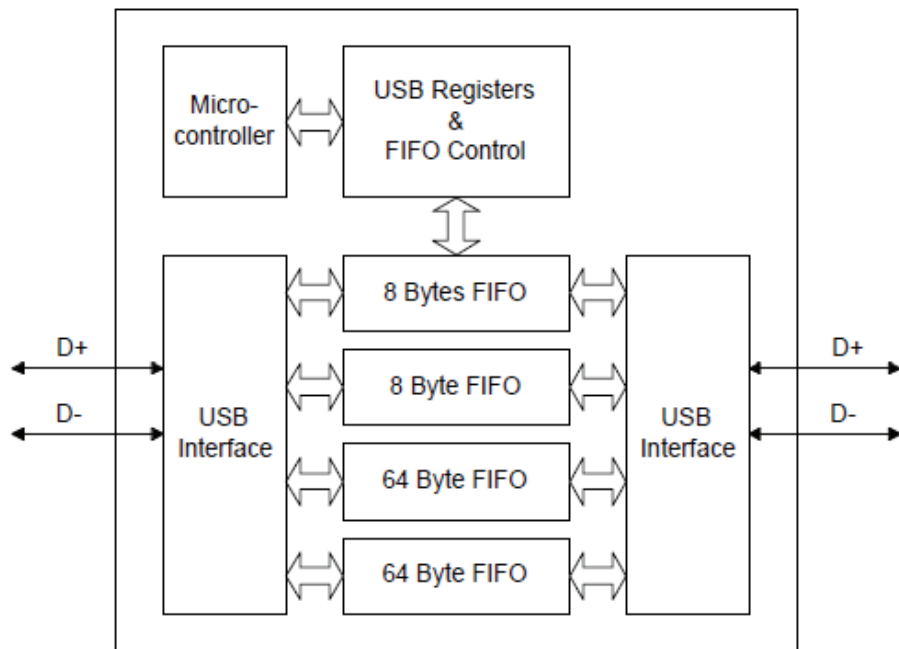
Block diagram of GL620USB-A
