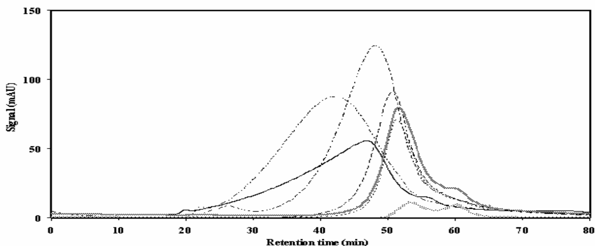
Fig.-1: UV detected SEC elution profiles of commercial SLS and their fractions obtained after diafiltration.
