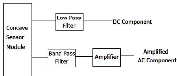
FIGURE 7. Diagram of signal processing module.
