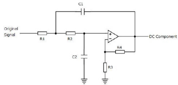
FIGURE 8. Circuit diagram of low pass filter.
