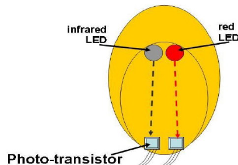
FIGURE 4. Top view of Concave Sensor Module.
