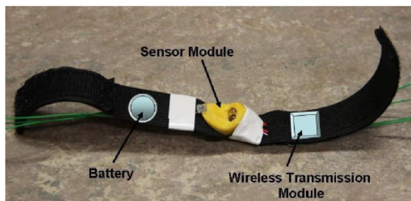
FIGURE 6. Photo of the sensor with further plan.
