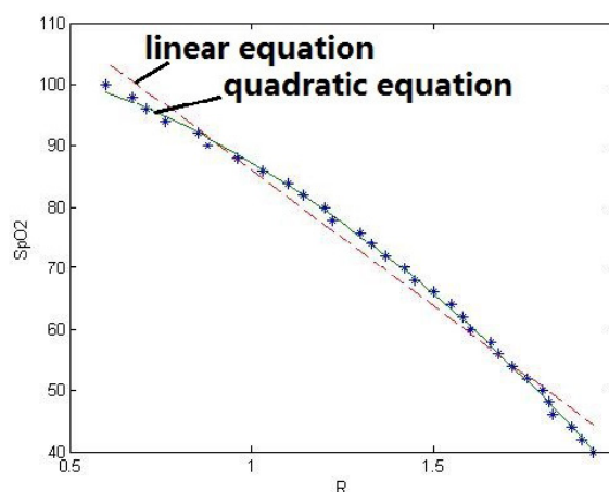
FIGURE 13. The R curve modeled by two relationships.
