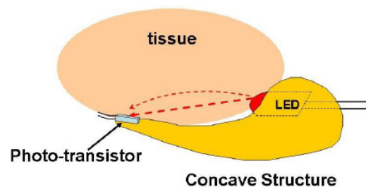
FIGURE 3. Section plan of Concave Sensor Module
