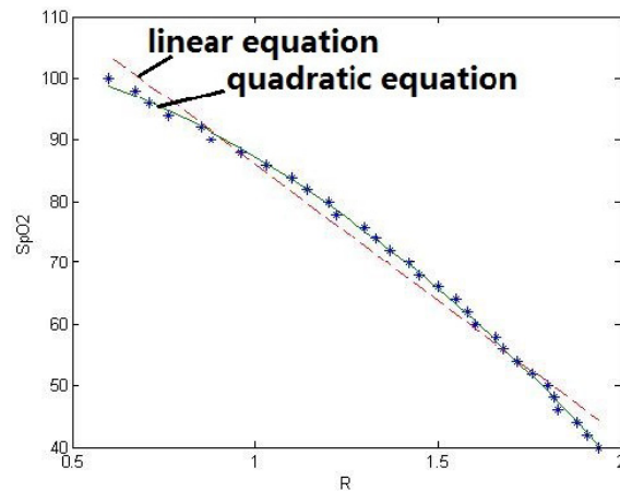
FIGURE 13. The R curve modeled by two relationships.
