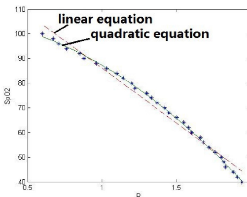
FIGURE 13. The R curve modeled by two relationships.
