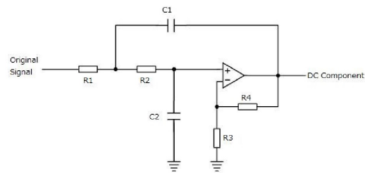
FIGURE 8. Circuit diagram of low pass filter.
