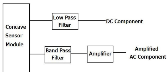
FIGURE 7. Diagram of signal processing module.
