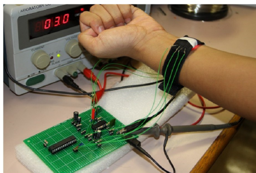
FIGURE 10. The photo of the overall implementation.
