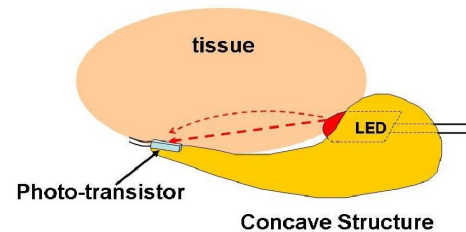
FIGURE 3. Section plan of Concave Sensor Module
