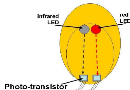
FIGURE 4. Top view of Concave Sensor Module.
