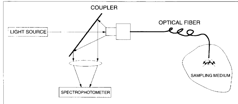
7. Basic block diagram of fiber-optic oximeter.
