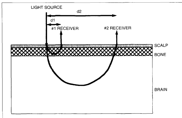
13. Near and far detector approach in estimation of deep layer tissue oxygenation as applied to the head.
