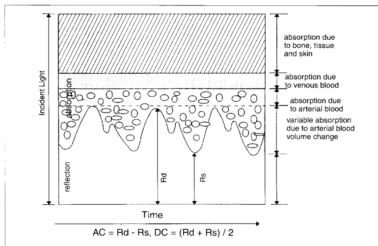
9. Conceptual tissue model for pulse oximetry.
