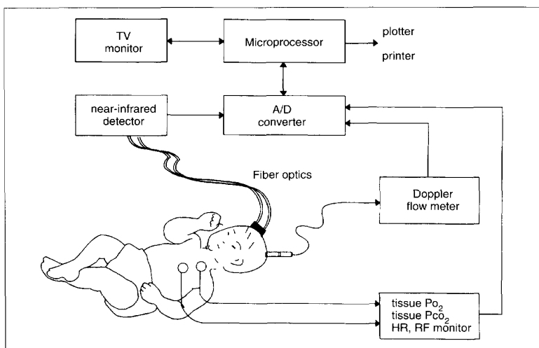
12. Block diagram of the neonatal cerebral monitoring system.
