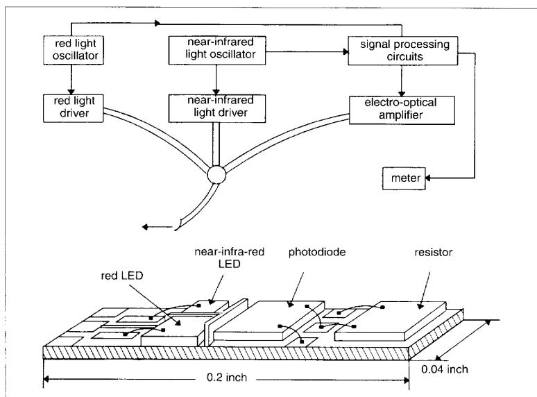
8. Basic illustration of the catheter-tip hybrid circuit oximeter sensor.
