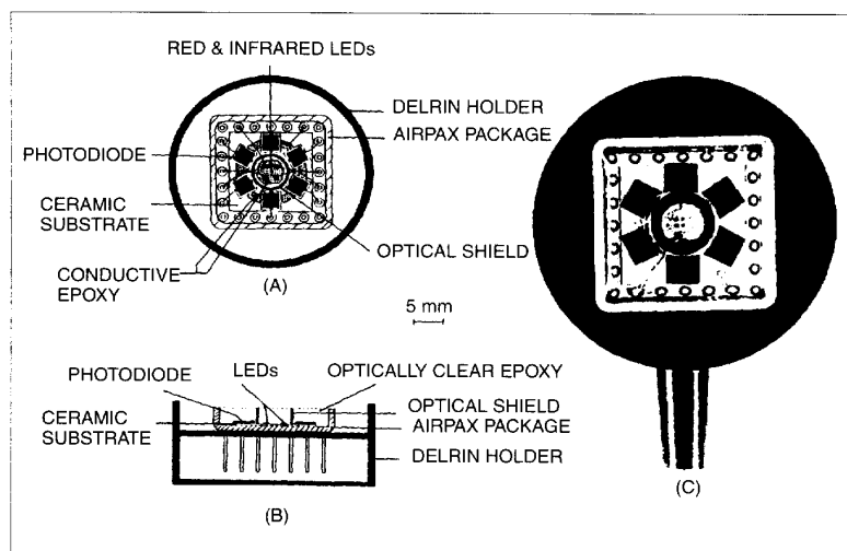
10. Schematic diagram of the reflectance oximeter sensor [68].
