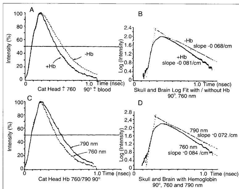
11. Measured pulse waveform of a picosecond light pulse through tissue. (a) Linear scale, (b) logarithmic scale, (c) effect of an alteration of wavelength from 790 to 760 nm in the cat-head model, a point at which the Hb absorbs maximally in this region [33], (d) logarithmic scale.
