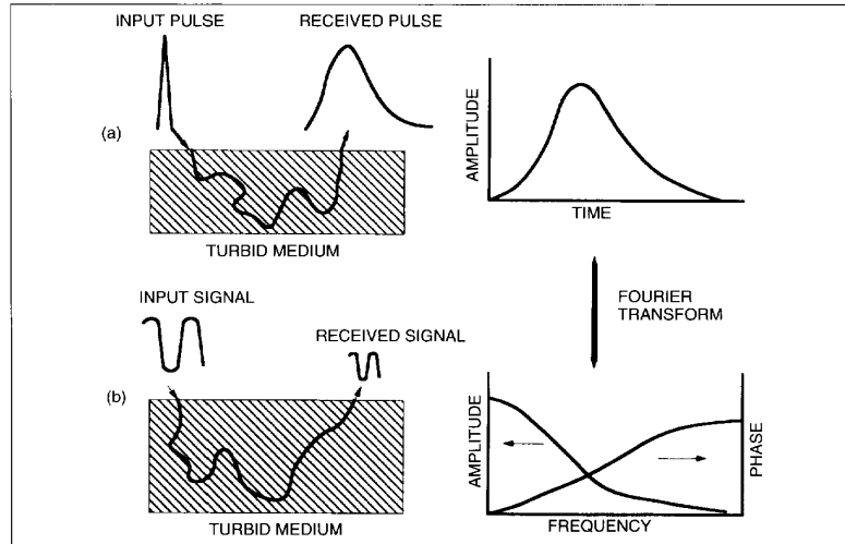
6. (a) Time and (b) frequency domain analysis of picosecond and ultra high frequency spectroscopy.
