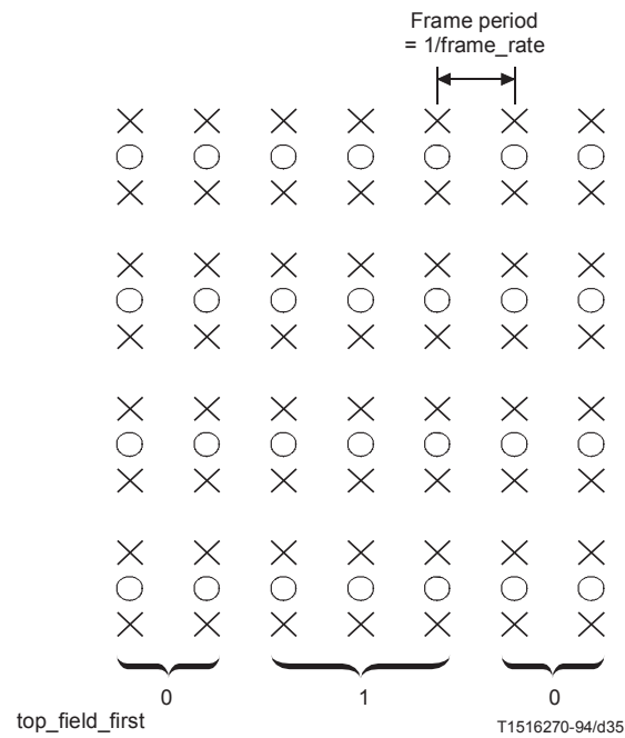
Figure 7-19 – progressive_sequence == '1'; repeat_first_field == '1'
