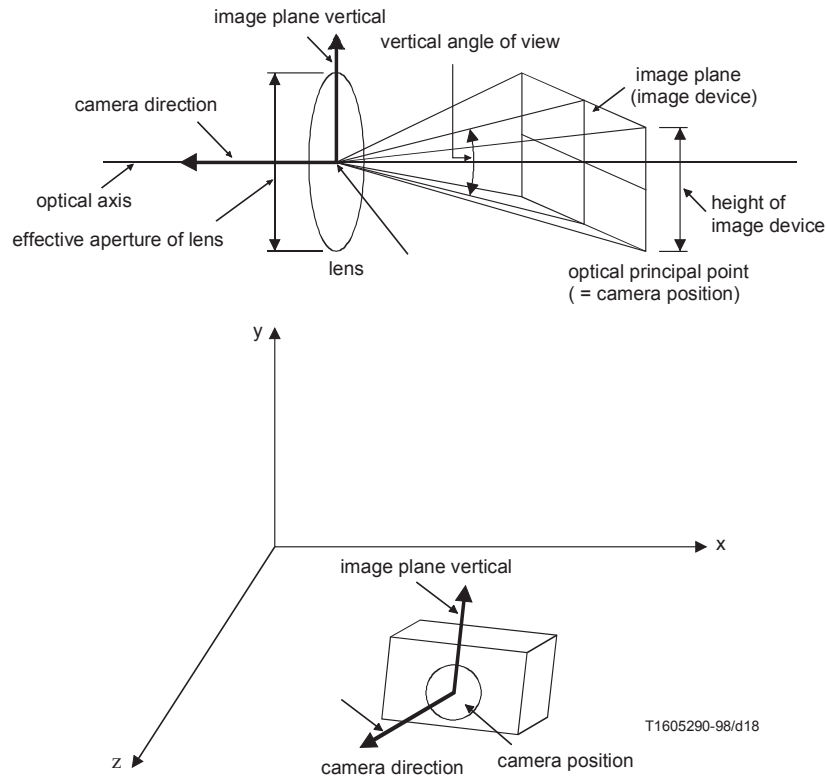
Figure 6-17 -- Camera parameters
