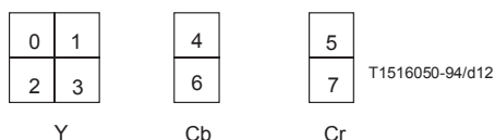
Figure 6-11 – 4:2:2 Macroblock structure
