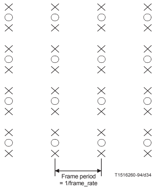
Figure 7-18 – progressive_sequence == 1
