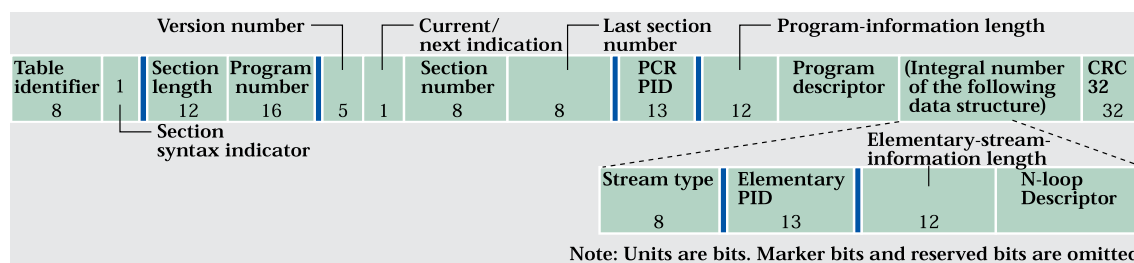
Figure 10: Configuration of TS Program Map Section
