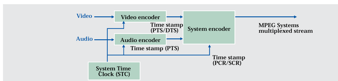
Figure 4: Encoder system example
