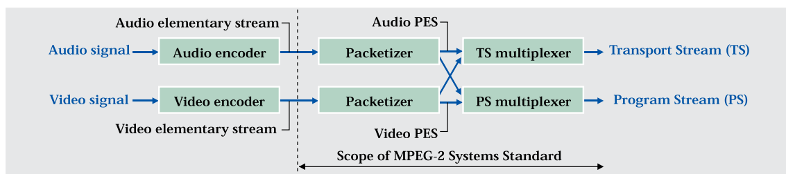
Figure 1: Outline of MPEG-2 Systems Standard
