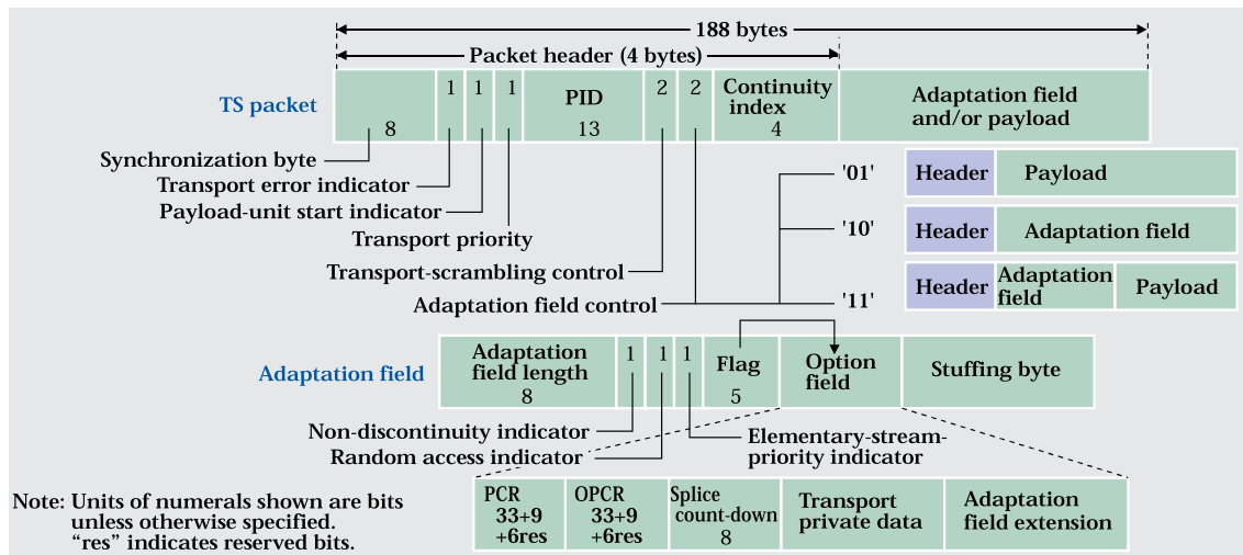
Figure 8: TS packet configuration
