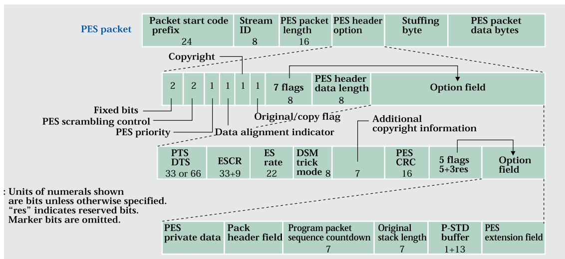
Figure 9: PES packet configuration
