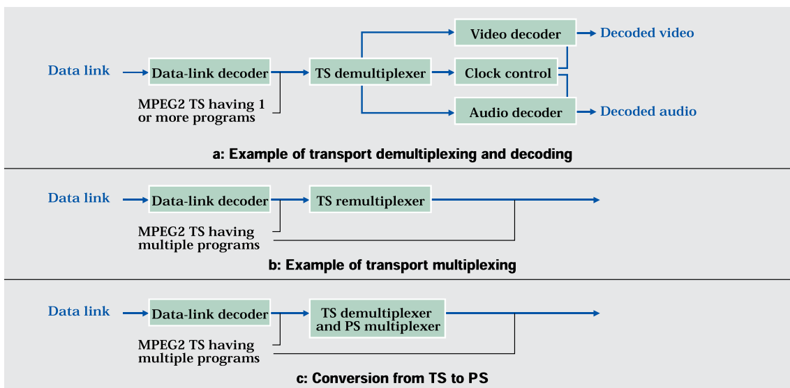
Figure 3: Outline of Transport Stream multiplexing
