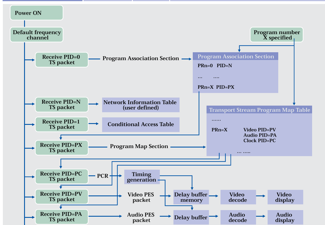
Figure 7: Example of stream selection by PSI in an MPEG2 Transport Stream
