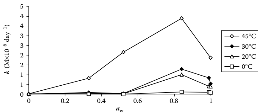
FIGURE 11.6 Apparent zero-order rate constants ( k ) of \text{H}_3\text{O}^+ formation as a function of a_w of coffee samples stored at different temperatures. (From Manzocco L., Nicoli M.C. 2007. Modeling the effect of water activity and storage temperature on chemical stability of coffee brews. Journal of Agricultural and Food Chemistry 55: 6521–6526, with permission.)
