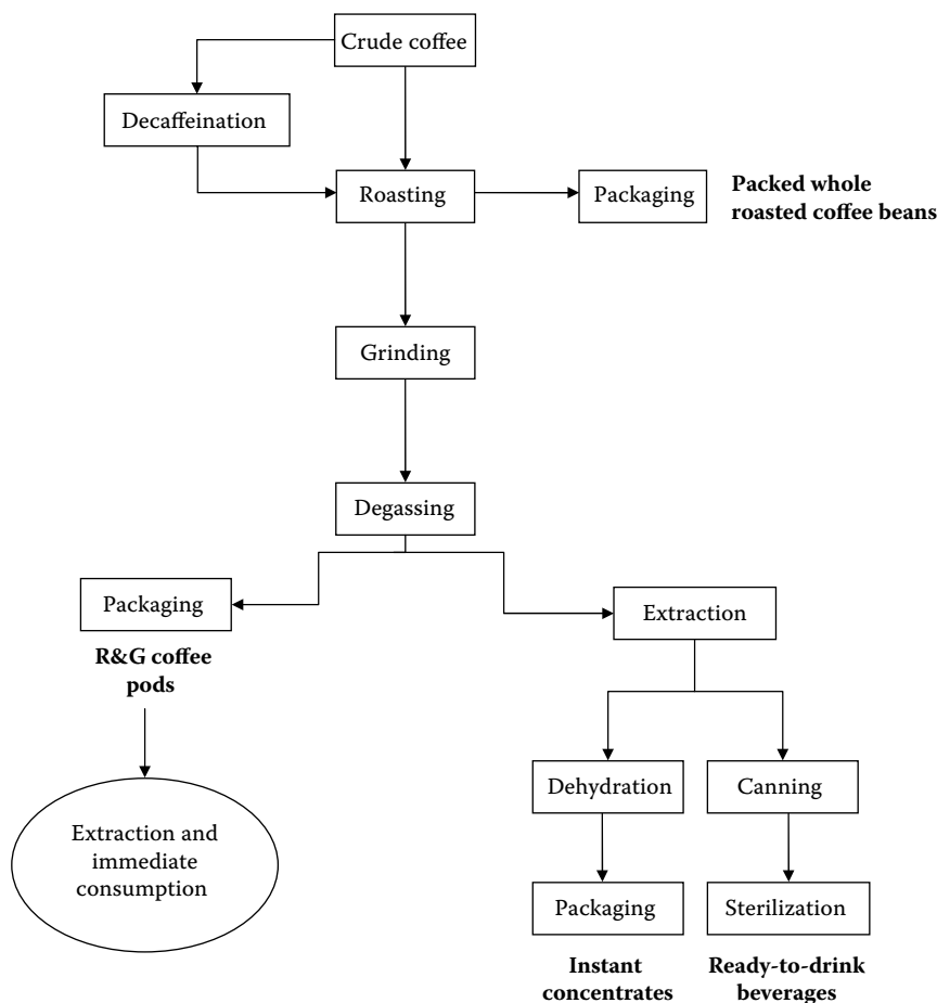
FIGURE 11.1 Key technological steps to obtain the most important coffee products present in the market.
