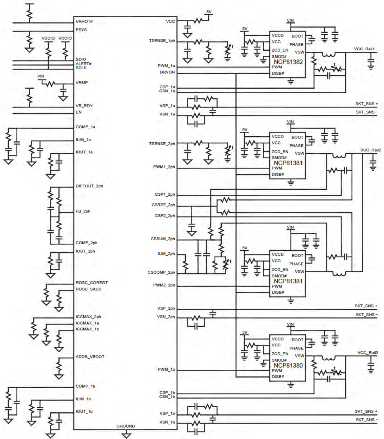
Figure 3. Application Schematic
