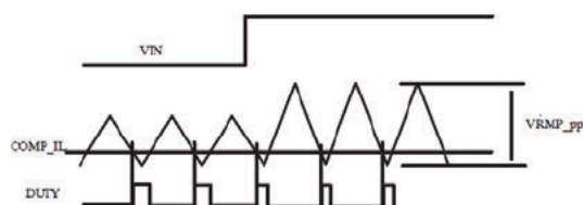
Figure 4. Ramp Feed Forward
