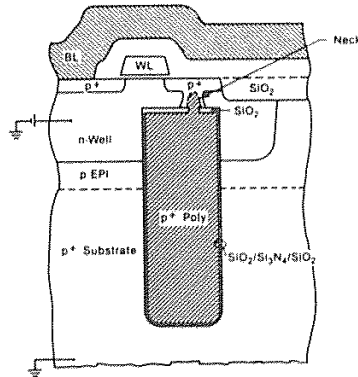
Fig. 8-24 Cross section of the SEOT cell. 71 (© 1988 IEEE).
