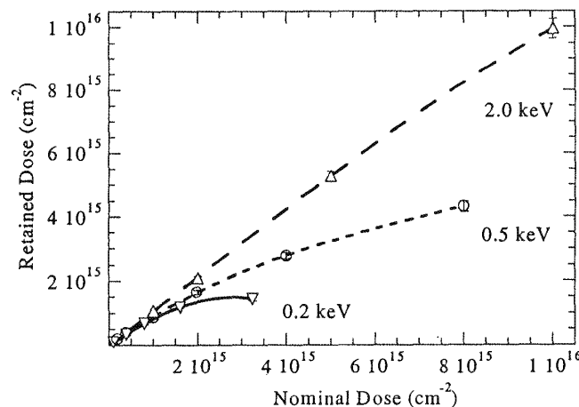
Fig. 5-24 Retained B-dose as a function of nominal B-dose implanted into (100)-silicon wafers with an as-received native oxide. The trend lines are 3 rd order polynomial spline-fits. For a nominal B-dose of 1 \times 10^{15}/\text{cm}^2 , sputtering leads to a reduction of ~10% in the retained dose at 0.5-keV, and a reduction of ~20% at 0.2-keV. 52
