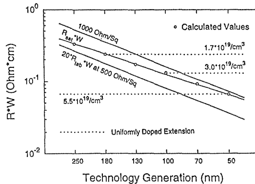
Fig. 5-17 Allowed values of drain (or source) extension resistance considering both bulk extension resistance R_{SDE} and extension spreading resistance R_{sp} . 23
