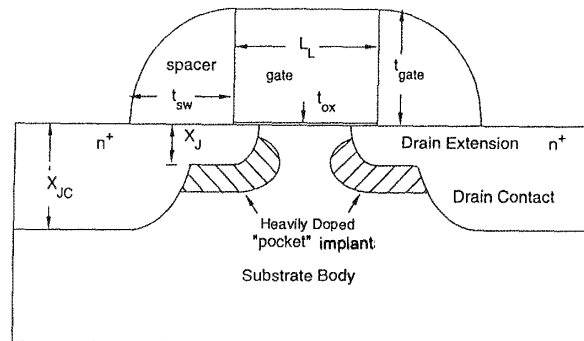
Fig. 5-27 MOSFET with heavily-doped pocket-implants for punchthrough-control.
