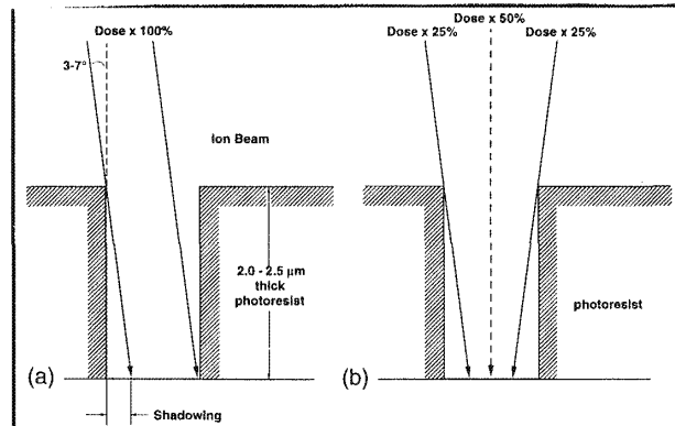
Fig. 5-6 The geometric effects of ion implantation into a narrow active region: a) low-tilt-angle shadowing and well misalignment; b) low-tilt quad implant provides both lateral and vertical (no channeling) uniformity.
