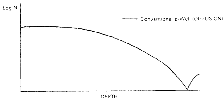
Fig. 5-1 Doping profile in a conventional well formed by a shallow implant and drive-in step. diffused well (in which the doping concentration after drive-in is highest at the surface, and decreases monotonically with depth, as seen in Fig. 5-1), such deeply implanted wells are known as retrograde-wells . * Comparison of the doping profiles in conventional and implanted p -well profiles (obtained by simulation) is shown in Fig. 5-2. 2,3 The retrograde-doping-profile is retained by minimizing the temperature-cycles of later process steps (e.g., by using RTP instead of furnace anneals).
