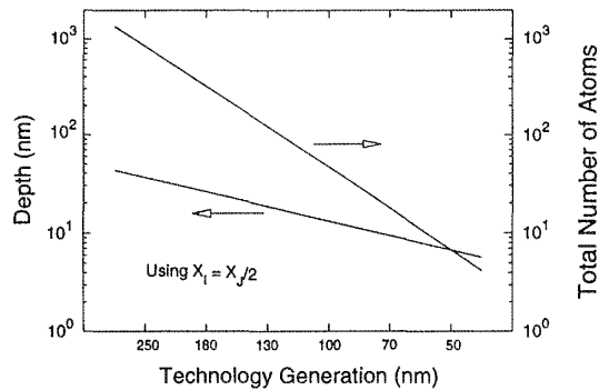
Fig. 5-10 Typical thickness of lighter-doped layer and total number of impurity atoms for 10^{17}/\text{cm}^3 surface doping density. 11
