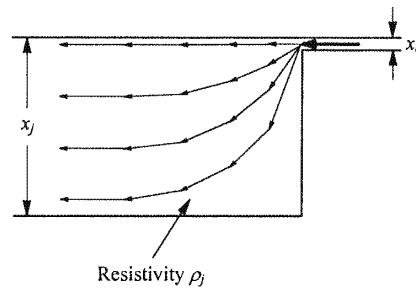
Fig. 5-16 Schematic diagram showing the resistance component associated with the injection region where the current spreads from a thin surface layer into a uniformly doped source or drain region. 22 (© 1983 IEEE)
