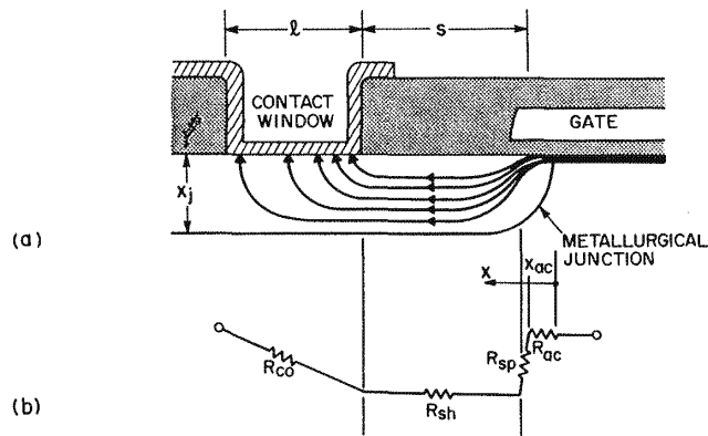
Fig. 5-13 Schematic drawing showing: a) current paths within the source and drain regions, of a planar MOSFET and; b) their corresponding representative series resistance components. 21 (© 1987 IEEE).
