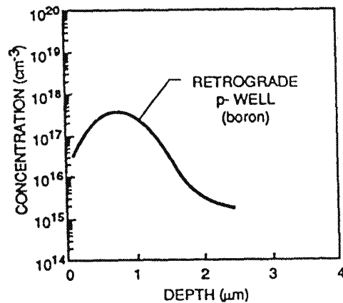
Fig. 5-3 Example of the doping profile of a retrograde p -well (boron) implant (400 keV).
