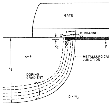
Fig. 5-15 Details of structures near the vicinity of the channel end. The dotted lines are contours of constant concentration. Dark region represents the accumulation layer. 21 (© 1987 IEEE).
