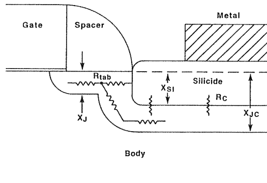
Fig. 5-14 Schematic drawing of the components of source or drain resistance in a deep-submicron MOSFET.
