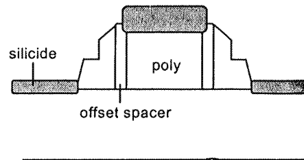
Fig. 5-25 Schematic of a deep-submicron MOSFET with an offset-sidewall spacer. 57
