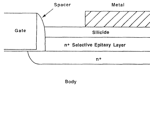
Fig. 5-19 Schematic of elevated-source/drain contacting structure.
