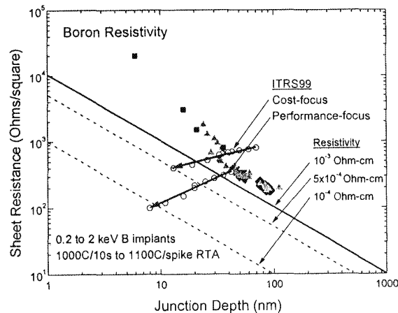
Fig. 5-20 Sheet resistance and source/drain junction depth expectations for CMOS transistors according to the ITRS99 study for cost and performance-focused product and gate sizes from 180 nm towards deeply-scaled devices with gates \sim 20 nm. Also shown are experimental results for sub-keV B^+ implants with "spike" RTA in CZ-Si materials. 59
