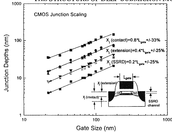
Fig. 5-12 Source/drain junction and undoped-channel depths for planar CMOS on bulk-Si.
