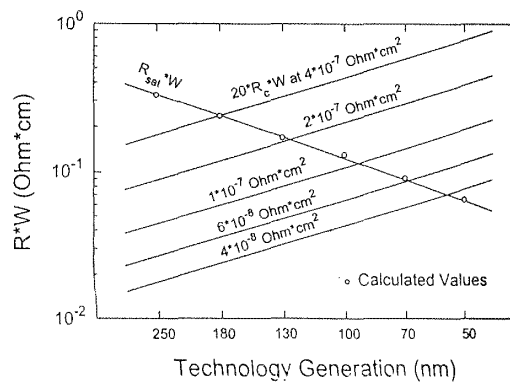
Fig. 5-18 Allowed values of drain (or source) contact-resistance. 23
