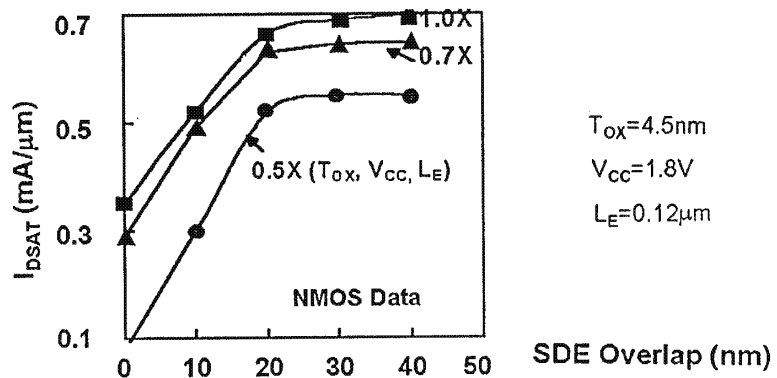
Fig. 5-26 I_{Dsat} versus SDE overlap (NMOS). 42
