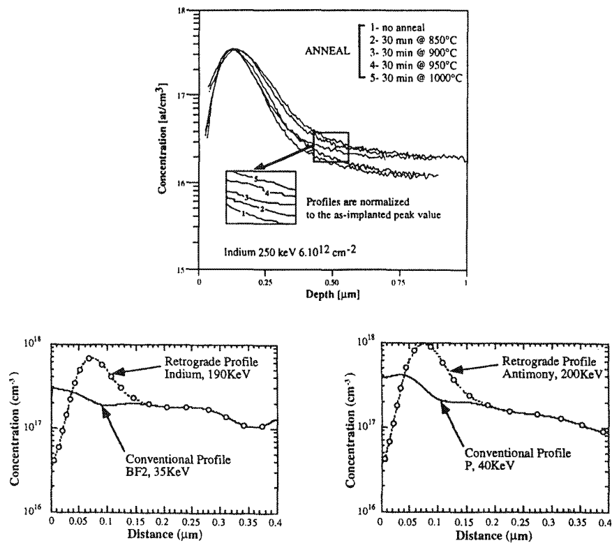
Fig. 5-11 a) SIMS data of indium profiles over a large range of annealing temperatures. Conventional and retrograde doping profiles (simulated) for b) NMOS and c) PMOS. 12
