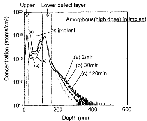
Fig. 5-30 Indium SIMS profiles for 1 \times 10^{14}/\text{cm}^2 implants at 200 keV annealed at 750°C for 2, 30, and 120 min in nitrogen. This figure shows large dose loss for indium. The depth of the defect layer (measured by XTEM) is shown (upper & lower defect layers). 54
