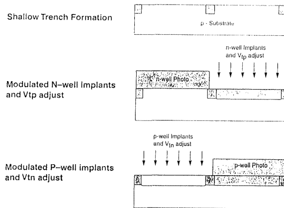
Fig. 5-5 Modulated n -well structure for advanced devices, showing the functions of each implant. 7
