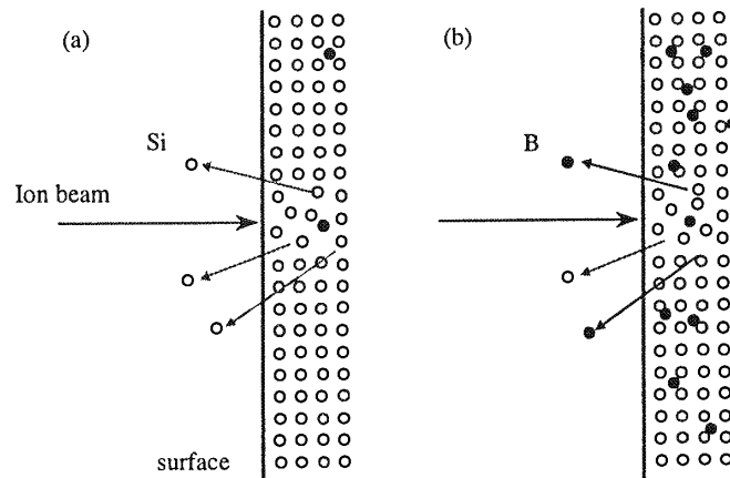
Fig. 5-23 The dose-loss due to self-sputtering depends on how much dopant has already been implanted. (a) At the start of the implant most of the sputtered atoms are silicon. (b) As the composition of the near surface layer becomes altered, with an increasing fraction of them being boron, more boron atoms are sputtered. 59
