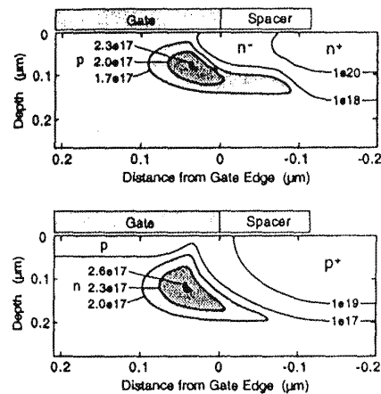
Fig. 5-28 Simulated 2-D impurity profiles of typical LATIPS structures for (a) NMOSFET with n -LDD region and; (b) Buried-channel PMOSFET. 49
