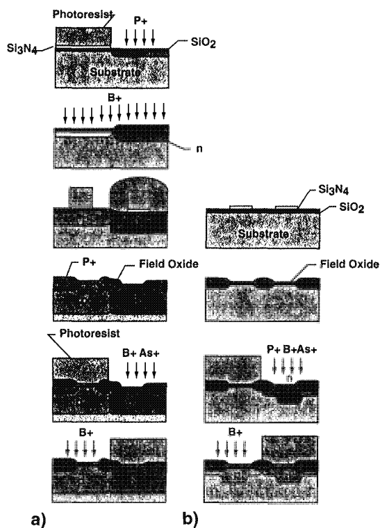
Fig. 5-4 Fabrication sequences for: a) conventional-diffused-well and; b) high-energy-implanted-well processes.
