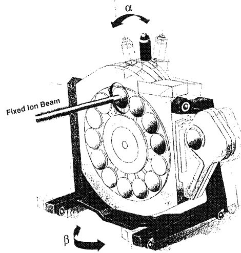
Fig. 5-8 In situ quad implants can be run on a batch end-station with orthogonal tilt axes (designated \alpha and \beta ).
