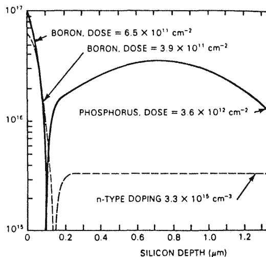
Fig. 5-2 Simulated doping profiles in PMOS channel regions: dashed lines, lightly doped substrate; solid lines, retrograde n -well. 3 (© 1982 IEEE).
