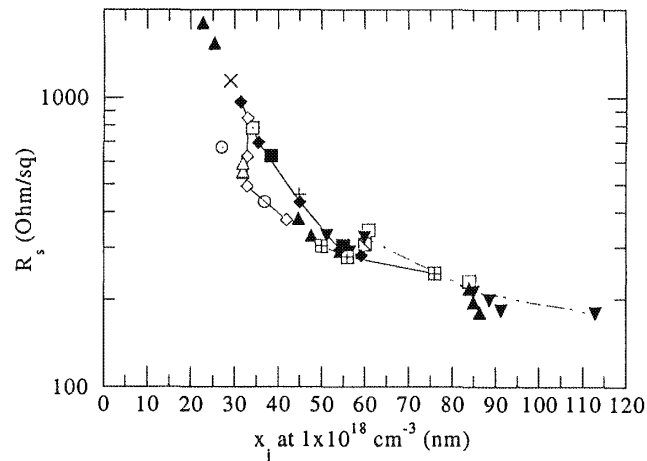
Fig. 5-22 Comparison of p -type sheet-resistance and junction-depth data for spike-anneals using various implant-and-annealing conditions. The data set includes a 400°C/sec ramp-up-rate and 0.2-keV implant-energy. Note that all the data points fall in a rather narrow band. No one has been able to make a 30-nm junction with a 300-Ω/sq sheet-resistance using ion-implantation and conventional rapid-thermal-annealing. 32
