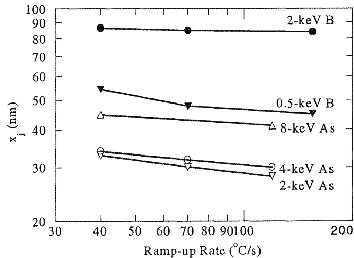
Fig. 5-21 Junction-depth, measured at a concentration of 1 \times 10^{18}/\text{cm}^3 after spike-annealing at various ramp-up-rates. The ramp-down-rate was the same in all cases. For both As and B the advantage from a faster ramp-up is largest for the shallowest implant. This implies that the reduction in TED (known to decrease with implant-depth) is not the dominant mechanism responsible for the larger reduction in junction-depths observed for the shallower-implants with increasing ramp-up-rates. 31
