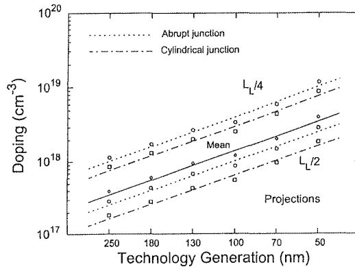
Fig. 5-9 Doping density required for punchthrough control. 11
