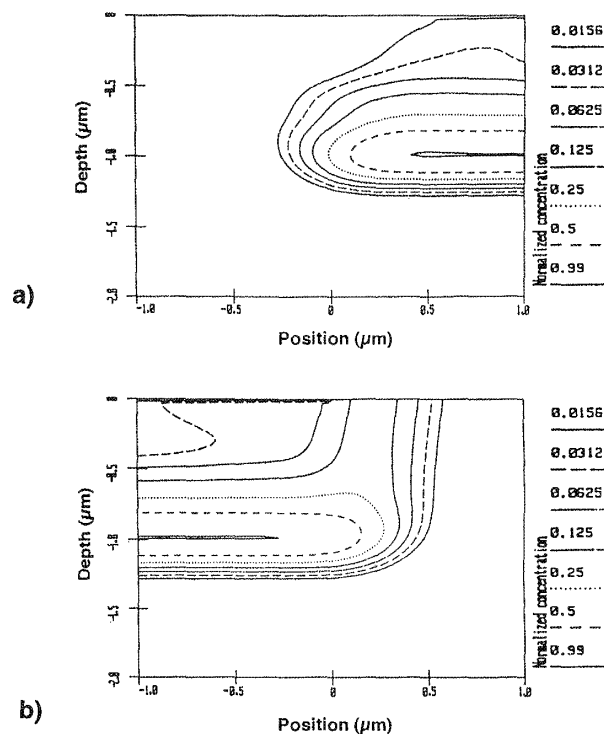
Fig. 5-7 Normalized doping profile of 1 MeV phosphorus implantation. a) On the shadow side (a) a lowly doped bulge is found (according to Monte Carlo simulation). b) On the incoming side, Monte Carlo simulation shows a trunk. 8
