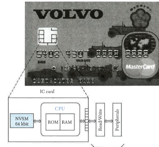
Fig. 22 An integrated-circuit (IC) card. The data stored in the NVSM can be accessed through the bus of the central processing unit (CPU). There are several metal pads connecting to the read/write machine. (Photography courtesy of Retone Information System Co., LTD.)
