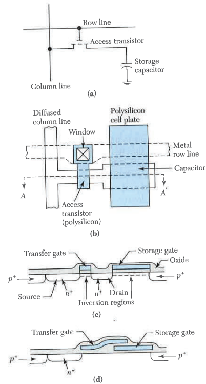
Fig. 18 Single-transistor dynamic random access memory (DRAM) cell with a storage capacitor. 9 (a) Circuit diagram. (b) Cell layout. (c) Cross section through A-A'. (d) Double-level polysilicon.
