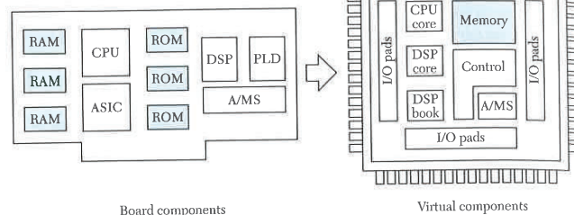
Fig. 37 System-on-a-chip of a conventional personal computer mother-board. 21
