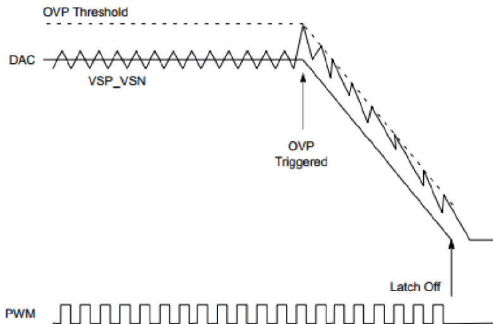
Figure 13. OVP During Normal Operation Mode
