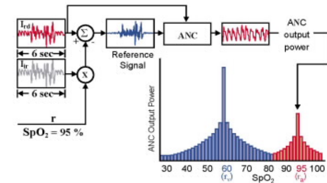
Figure C: "During Motion" DST plot at SpO_2 of 95%
