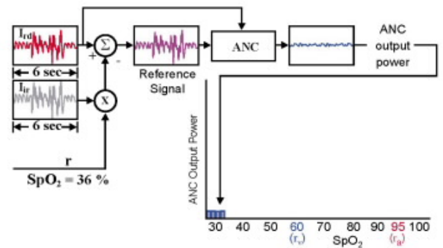
Figure A: "During Motion" DST plot at SpO_2 of 36%
