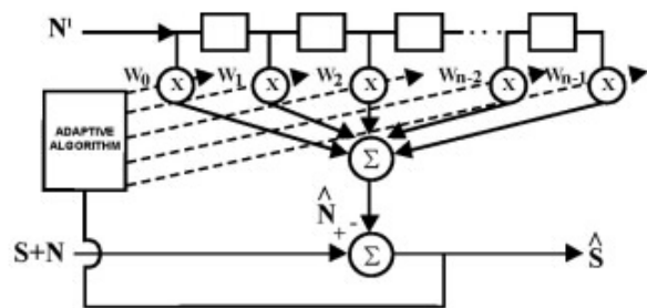
Adaptive Noise Canceller (ANC) block diagram
