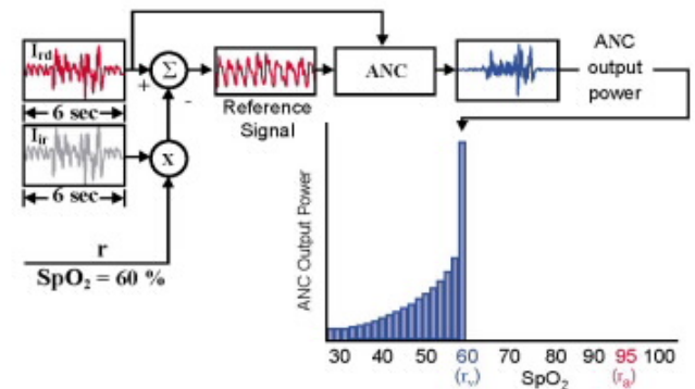
Figure B: "During Motion" DST plot at SpO_2 of 60%
