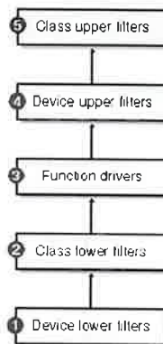
Figure 2-7. Order of AddDevice calls
