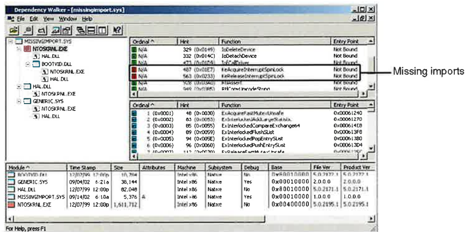
Figure A-3. DEPENDS shows missing imports.
