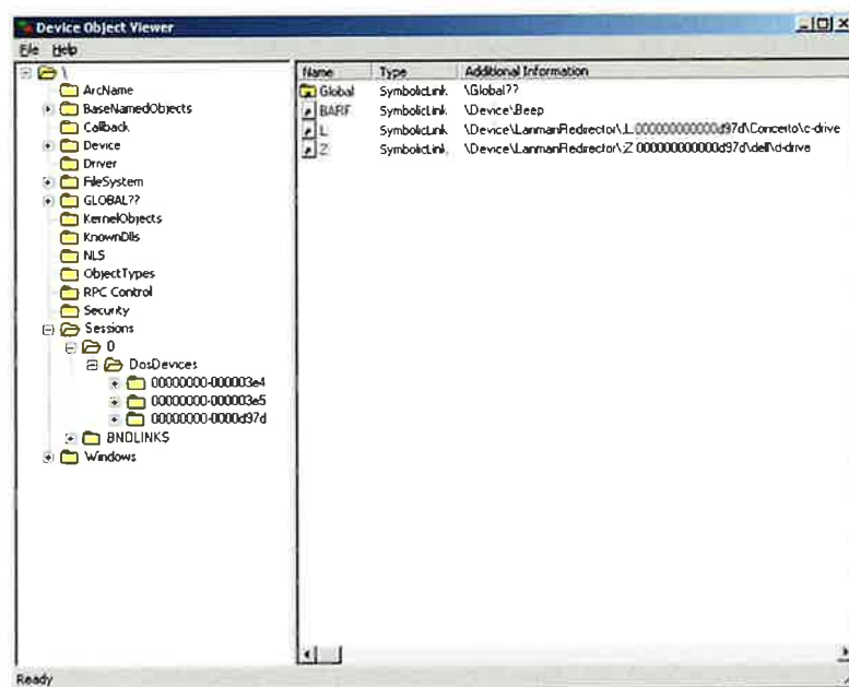
Figure 2-18. Symbolic link created by DefineDosDevice
