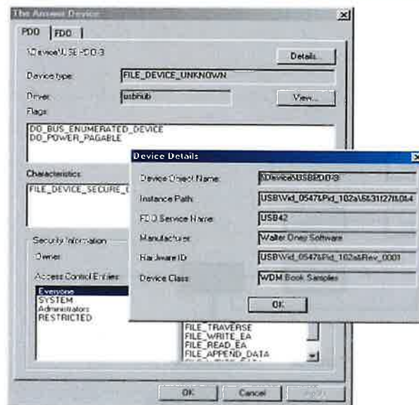
Figure 2-11. DEVVIEW information about USB42's PDO.
