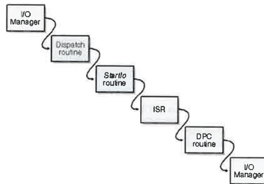
Figure 5-5. The “standard model” for IRP processing.
