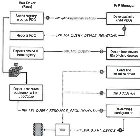
Figure 2-5. Loading a legacy driver.
