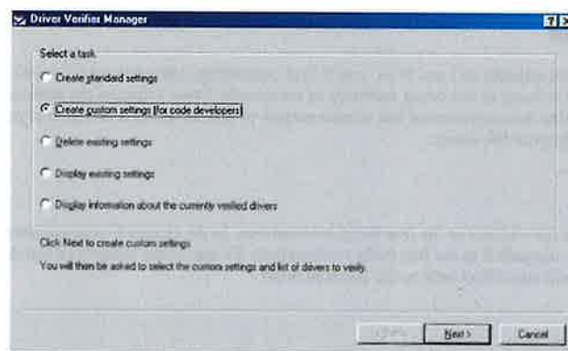
Figure 3-14. Initial Driver Verifier wizard page
