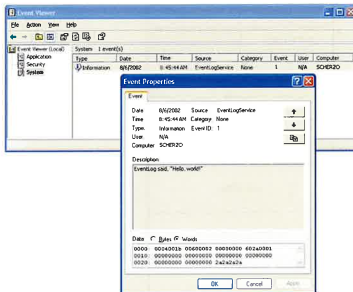
Figure 14-1. The Windows XP Event Viewer.
