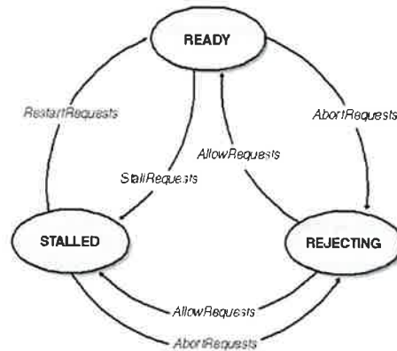
Figure 6-3. States of a DEVQUEUE object.
