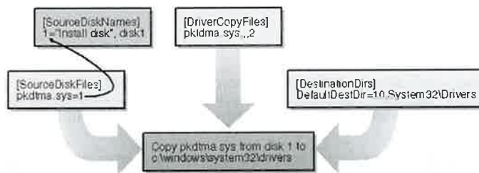
Figure 15-10. Source and destination information for file copies.
