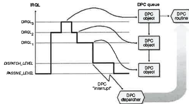
Figure 7-5. Processing DPC requests.
