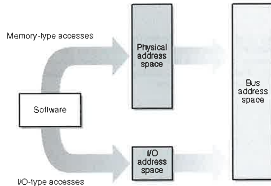
Figure 7-4. Accessing ports and registers.
