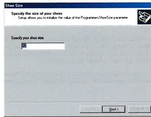
Figure 15-13. Wizard page presented by a co-installer DLL.
