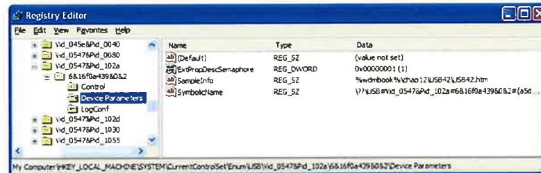
Figure 15-4. A device parameters key in the registry.
