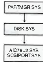
Figure 16-1. Driver stack for a hard drive.
