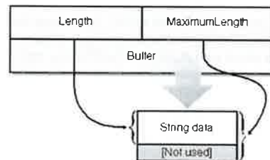
Figure 3-13. The UNICODE_STRING and ANSI_STRING structures.
