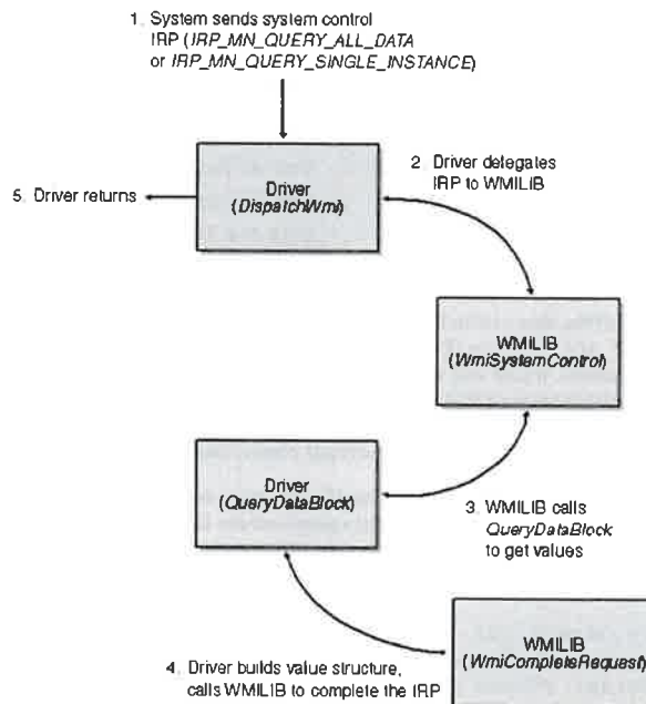
Figure 10-4. Control flow for data queries.
