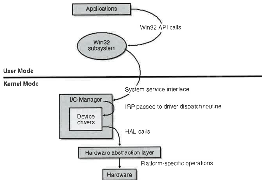
Figure 1-1. Windows XP architecture.
