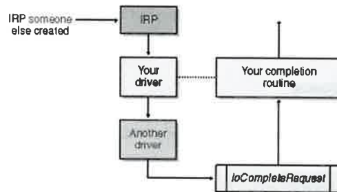
Figure 5-11. Pass down with completion routine.
