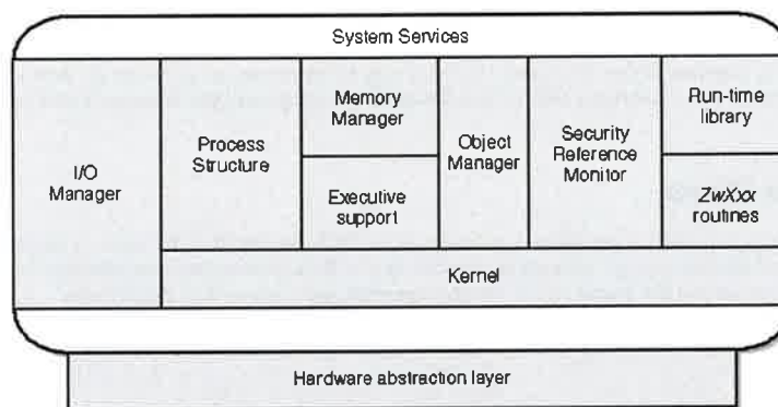
Figure 3-1. Overview of kernel-mode support routines
