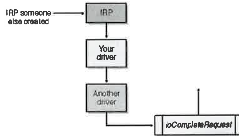
Figure 5-12. Pass down without completion routine.
