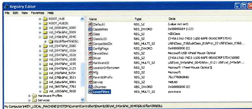
Figure 16-7. Preparing to use POWTRACE.
