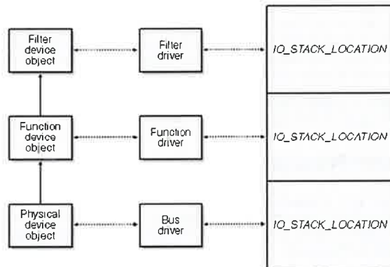
Figure 5-3. Parallelism between driver and I/O stacks.
