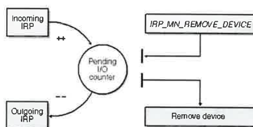
Figure 6-5. Operation of an IO_REMOVE_LOCK .
