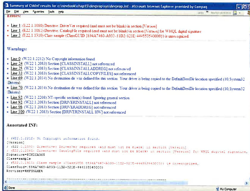
Figure 15-11. Output from CHKINF utility.
