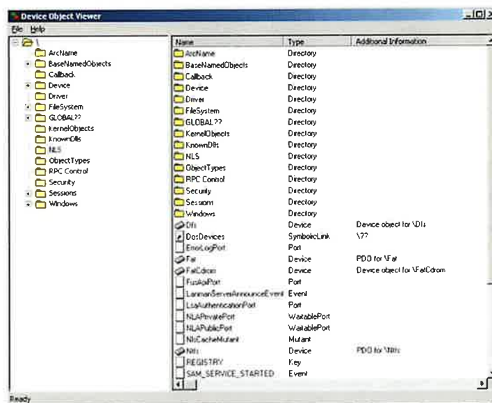
Figure 2-16. Using DEVVIEW to view the namespace.
