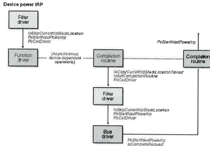
Figure 8-10. IRP flow when decreasing device power.
