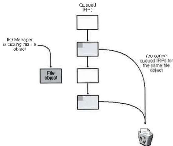
Figure 5-10. Driver responsibility for IRP_MJ_CLEANUP .
