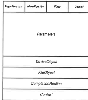
Figure 5-4. I/O stack location data structure.
