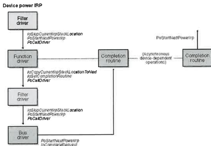
Figure 8-9. IRP flow when increasing device power.
