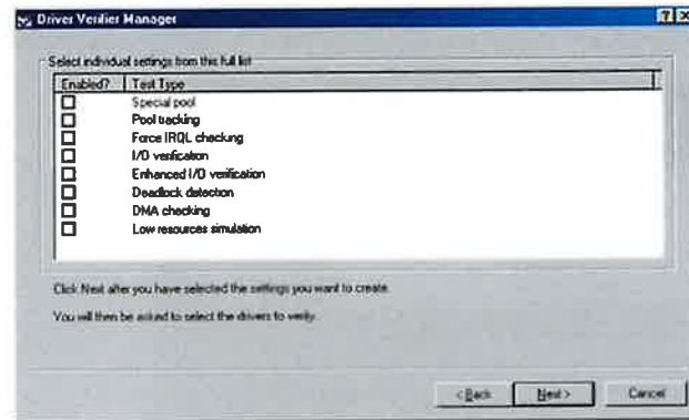
Figure 3-16. Driver Verifier's custom settings wizard page
