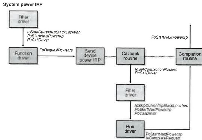
Figure 8-7. IRP flow when decreasing system power.
