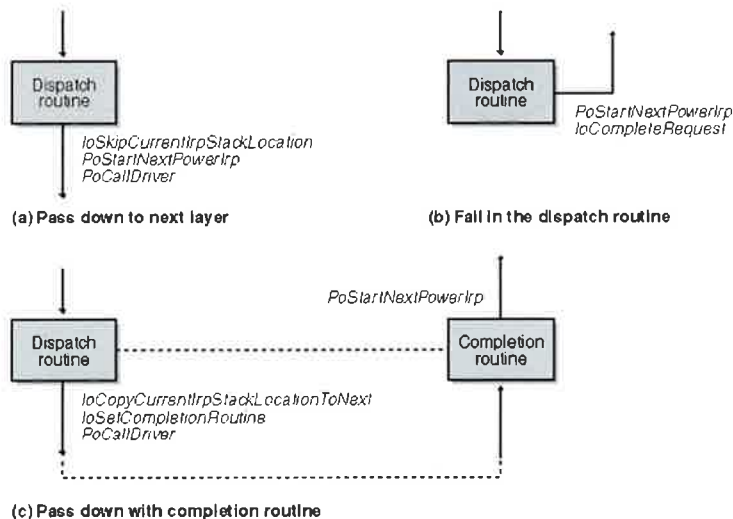
Figure 8-3. Handling IRP_MJ_POWER requests.
