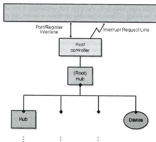
Figure 12-1. Hierarchy of USB devices.
