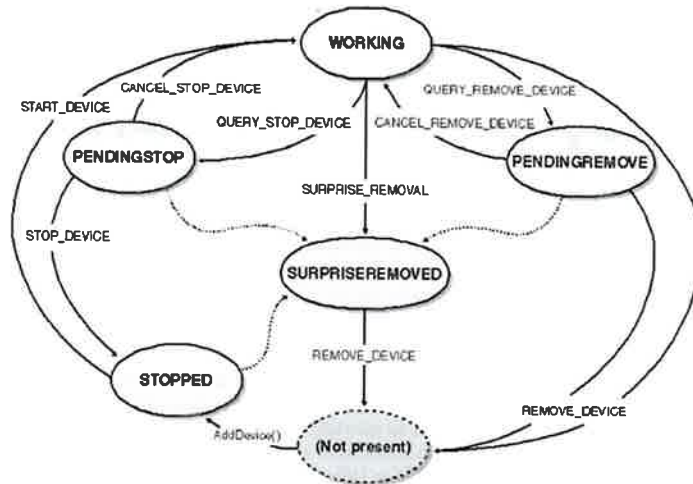
Figure 6-1. State diagram for a device.
