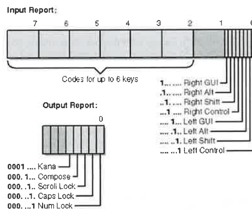
Figure 13-2. Layout of keyboard input and output reports.
