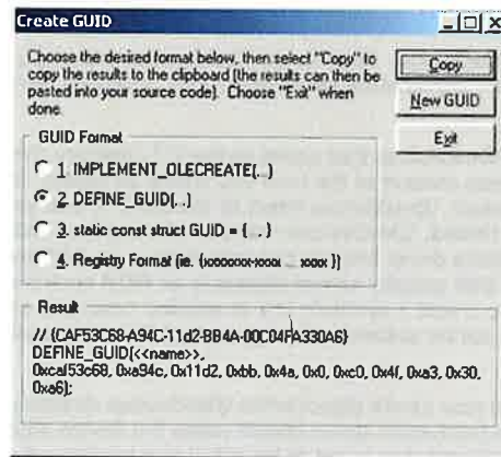
Figure 2-19. Using GUIDGEN to generate a GUID
