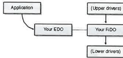
Figure 16-9. An Extra Device Object for a filter driver.
