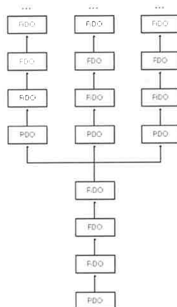
Figure 2-6. Layering of recursively enumerated devices.
