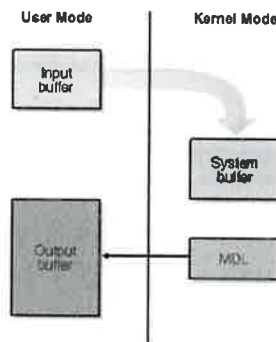
Figure 9-4. Buffer management with METHOD_XXX_DIRECT .
