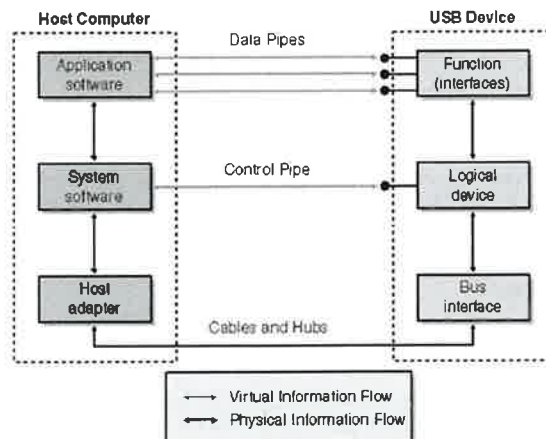
Figure 12-3. Layered model for USB communication.
