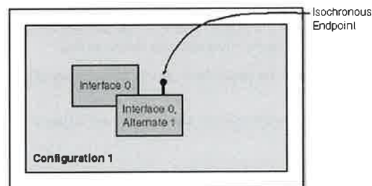
Figure 12-18. Descriptor structure for the USBISO device.
