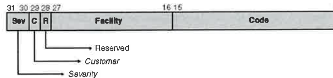
Figure 3-2. Format of an NTSTATUS code.
