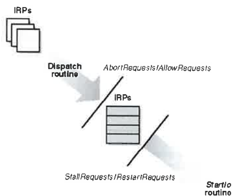
Figure 6-4. Flow of IRPs through a DEVQUEUE .
