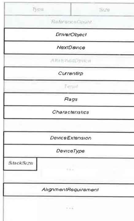
Figure 2-15. The DEVICE_OBJECT data structure.
