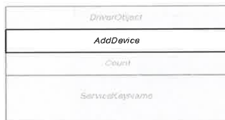
Figure 2-14. The DRIVER_EXTENSION data structure.
