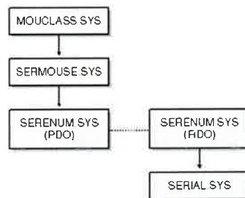
Figure 16-5. Driver stack for a serial mouse.
