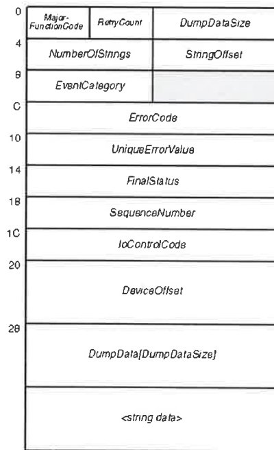
Figure 14-3. The IO_ERROR_LOG_PACKET structure.
