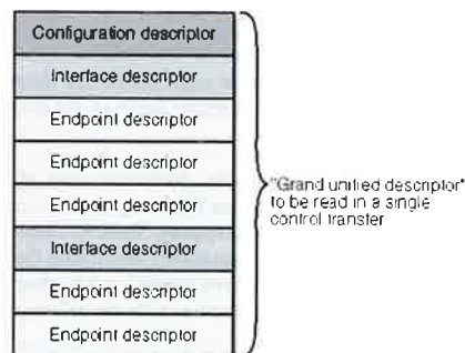
Figure 12-14. Structure of a configuration descriptor.
