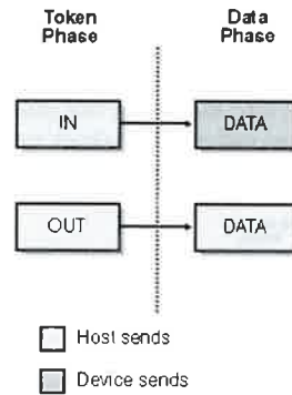
Figure 12-10. Phases of an isochronous transfer.
