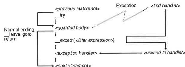
Figure 3-4. Flow of control in a try-except block.
