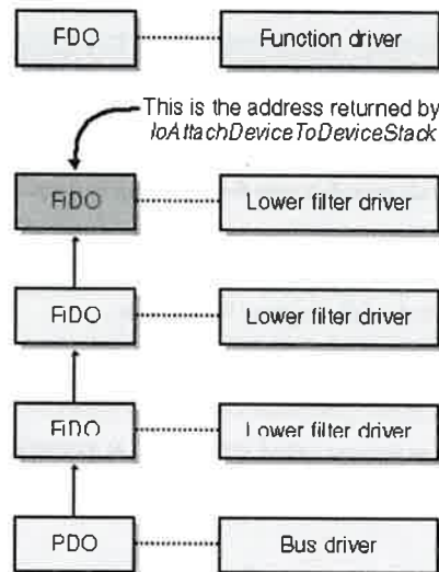
Figure 2-21. What IoAttachDeviceToDeviceStack returns.
