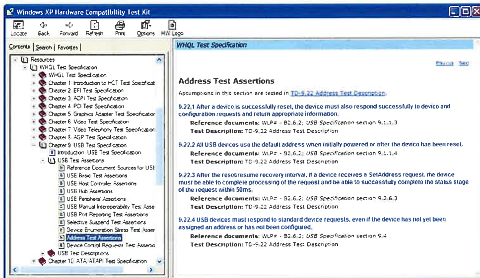
Figure 15-21. Documentation for test assertions.
