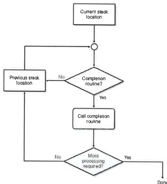
Figure 5-7. Logic of IoCompleteRequest .
