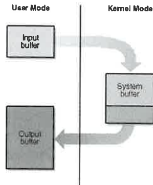
Figure 9-3. Buffer management with METHOD_BUFFERED .
