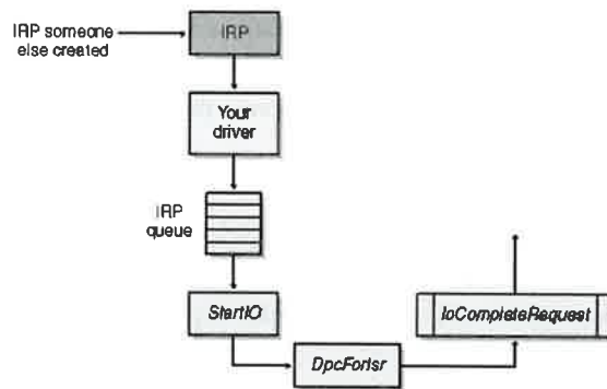
Figure 5-14. Queue for later processing.
