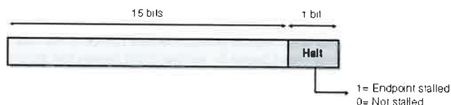
Figure 12-16. Bits in endpoint status.
