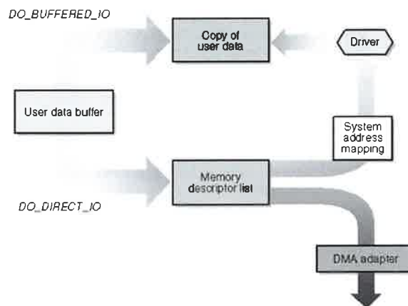
Figure 7-2. Accessing user-mode data buffers.
