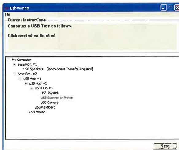
Figure 15-17. Required hardware topology for the USB Manual Interoperability test.
