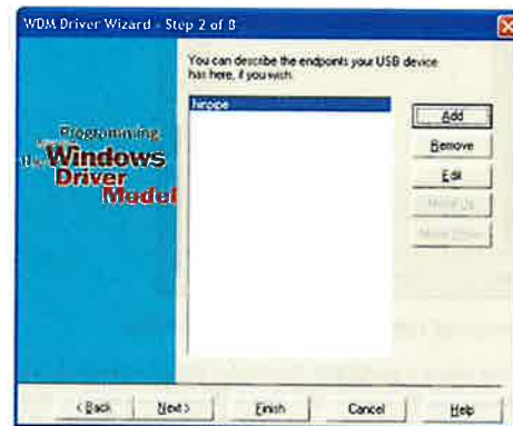
Figure B-6. Page for defining USB endpoints.
