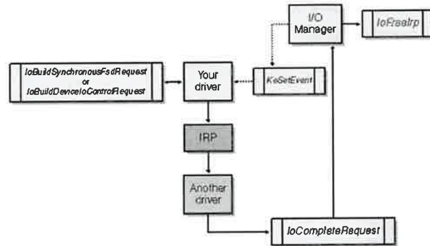
Figure 5-16. Your own synchronous IRP.
