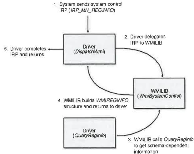
Figure 10-3. Control flow for IRP_MN_REGINFO.
