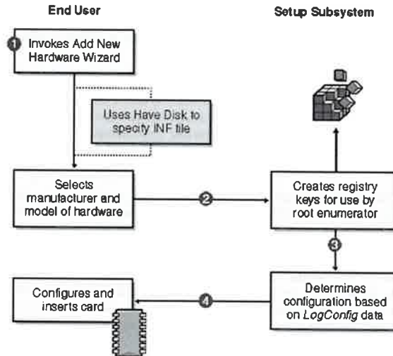
Figure 2-4. The detection process for a legacy device.
