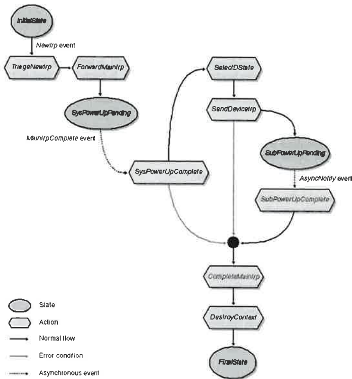
Figure 8-6. State transitions when increasing system power.
