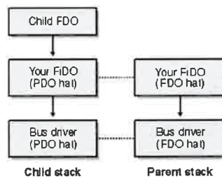
Figure 16-10. Bus filter topology.
