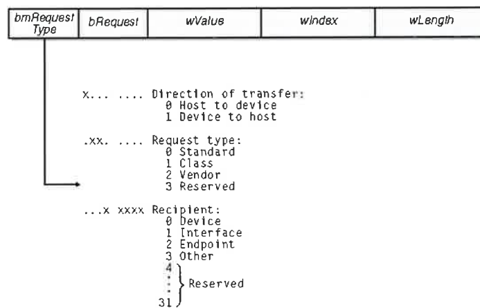
Figure 12-8. Contents of a SETUP token.
