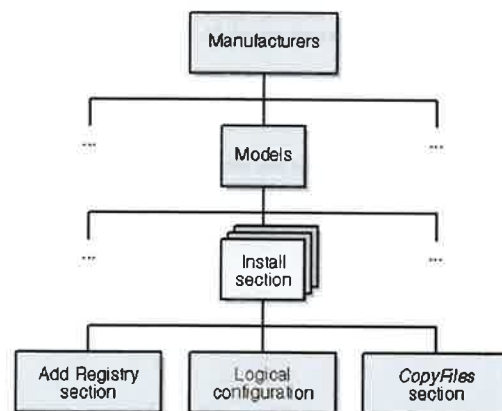
Figure 15-8. Tree structure of an INF file.
