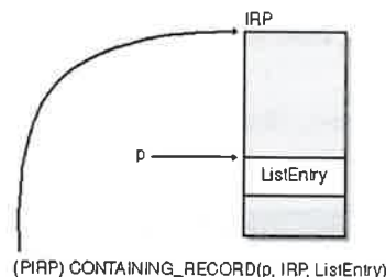
Figure 3-7. The CONTAINING_RECORD macro.
