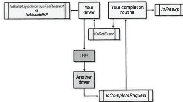
Figure 5-18. Asynchronous IRP handled synchronously.
