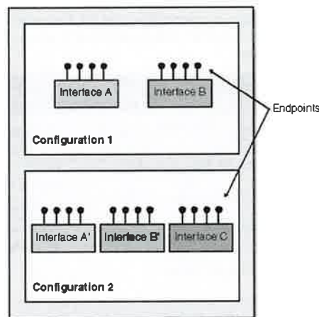
Figure 12-2. Device configurations, interfaces, and endpoints.
