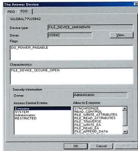
Figure 2-12. DEVVIEW information about USB42's FDO.
