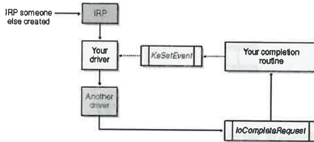
Figure 5-17. Synchronous pass down.
