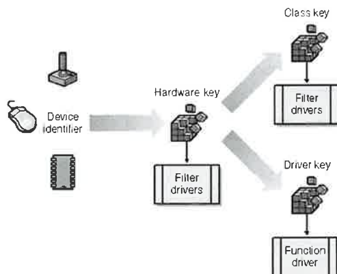
Figure 15-1. Meaningful registry keys for a device.
