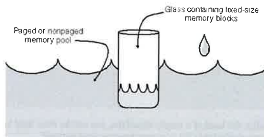
Figure 3-12. Lookaside lists.
