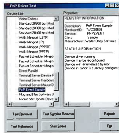
Figure 6-8. PNPDriverTest window.
