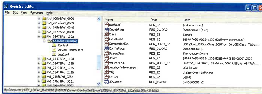
Figure 15-2. A hardware key in the registry.
