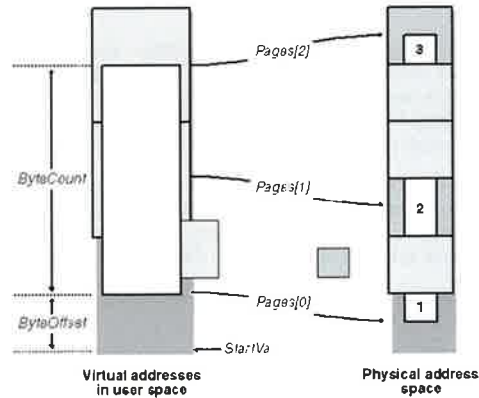
Figure 7-3. The memory descriptor list structure.
