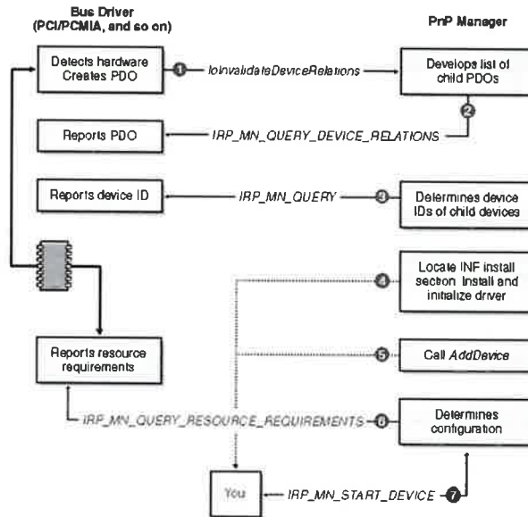
Figure 2-3. Installing a Plug and Play device.
