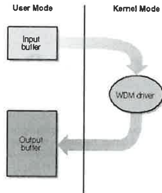
Figure 9-1. Input and output buffers for DeviceIoControl .
