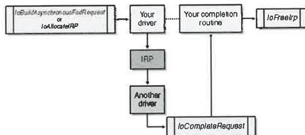
Figure 5-15. Your own asynchronous IRP.
