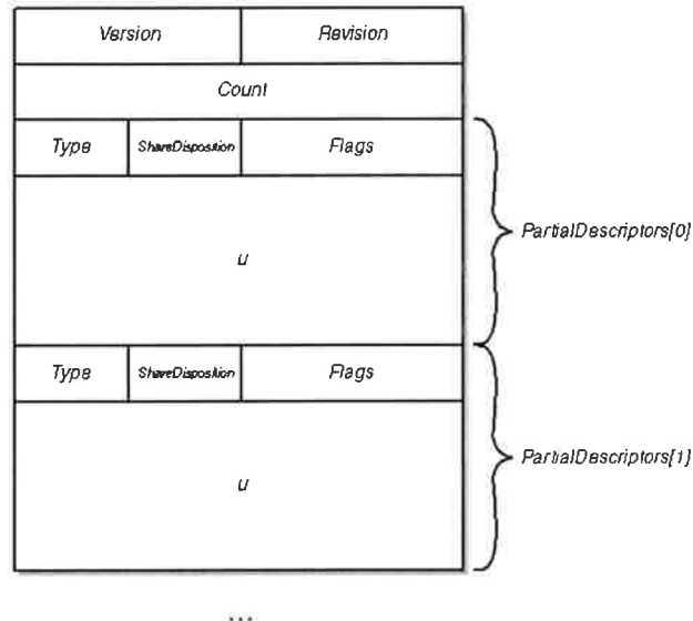
Figure 7-1. Structure of a partial resource list.
