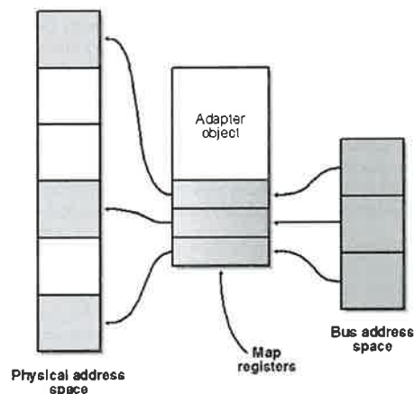
Figure 7-6. Abstract computer model for DMA transfers.
