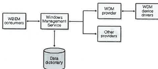
Figure 10-2. The world of WMI.
