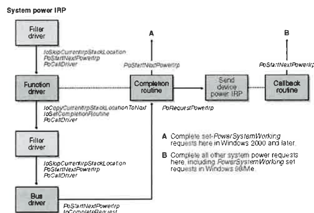
Figure 8-5. IRP flow when increasing system power.
