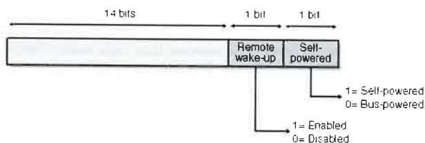
Figure 12-15. Bits in device status.
