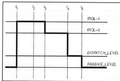
Figure 4-2. Interrupt priority in action.
