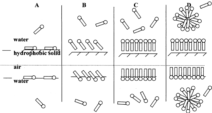
Figure 2. Simplified models of the interfacial behavior of a nonionic surfactant at several concentrations in water. Circles—polar head groups (e.g., polyoxyethlenes). Rectangles—hydrophobic tails (e.g., hydrocarbon chains). Models above the dotted line is for the hydrophobic solid (ice)/water interface and those below are for the air/water interface. (A) Surfactant concentration is well below the CMC (B) Surfactant concentration is greater than in A, but still below the CMC. (C) Surfactant concentration is at the CMC. (D) The surfactant concentration is above the CMC. (This model is adapted from Figures 4.4 and 4.8 of Porter (Porter, 1994)).
