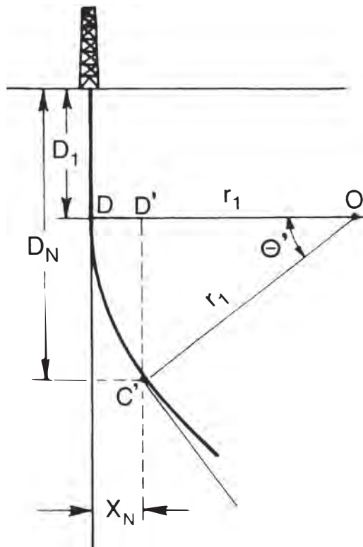
Fig. 8.10—Geometry for the build section.
