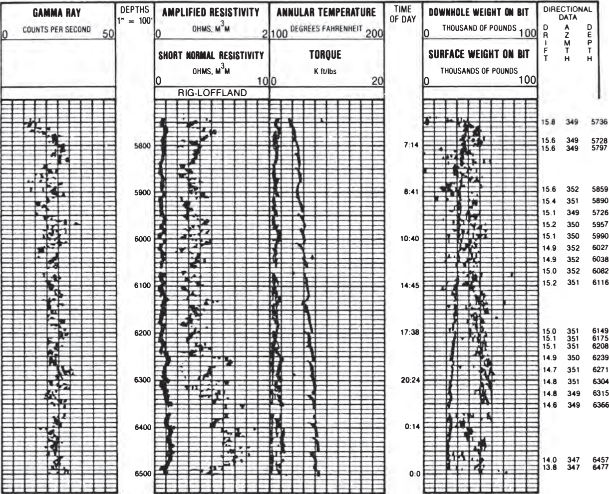
Fig. 8.61A—Typical multisensor MWD output.
