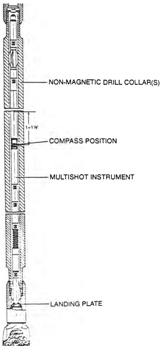
Fig. 8.48—Typical arrangement for landing a multishot instrument (after Eikelberg et al. 6 ).
