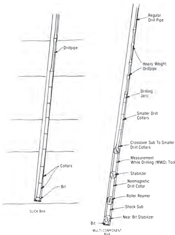
Fig. 8.120—Bottomhole assemblies.
