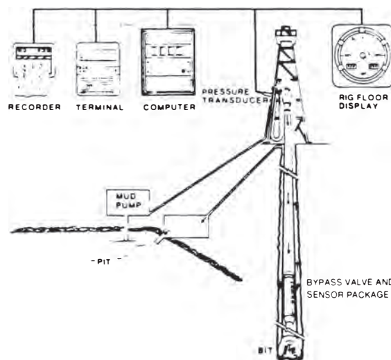
Fig. 8.59—Typical MWD system (after Gearhart et al. 9 ).
