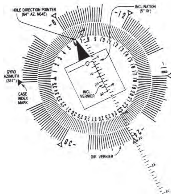
Fig. 8.71—Gyroscope face.
