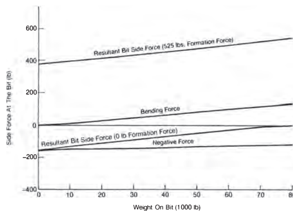
Fig. 8.127—Results of BHA calculation for slick BHA.
