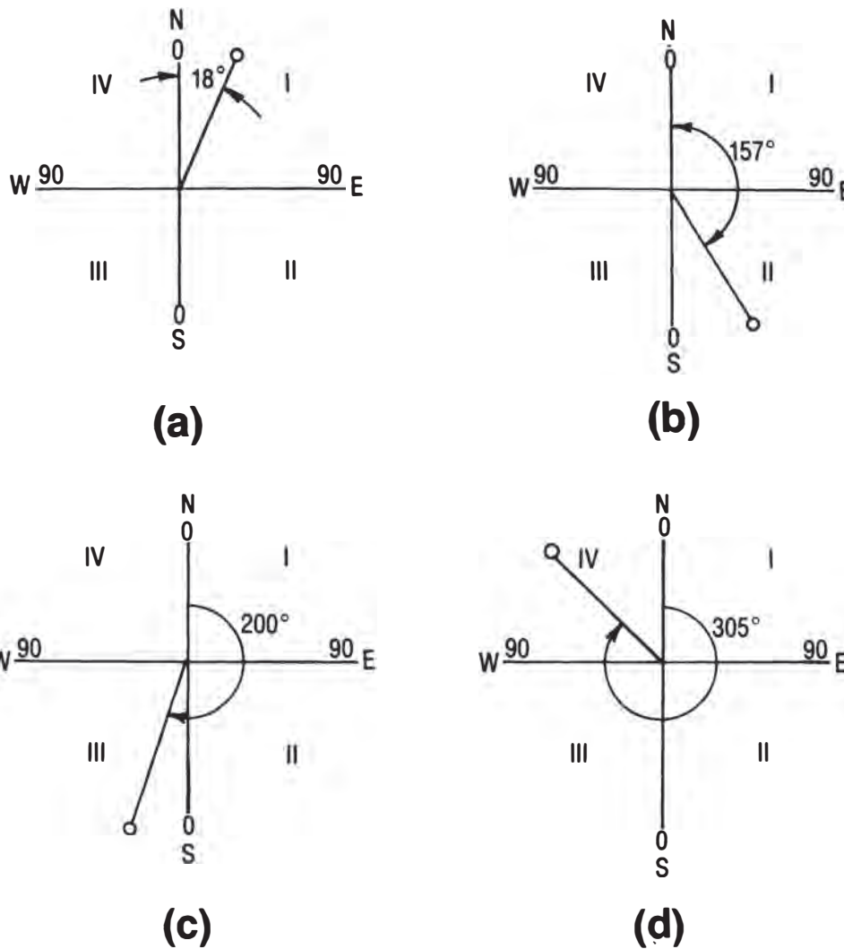
Fig. 8.15—Directional quadrants and compass measurements.
