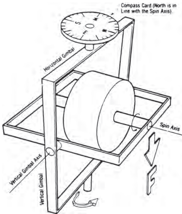
Fig. 8.68—Typical gyroscope.
