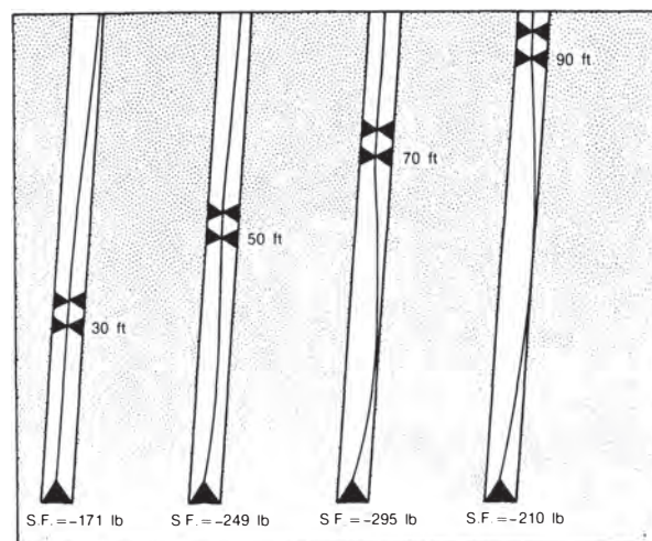
Fig. 8.133A—Tangency between bit and stabilizer resulting from pendulum length and inclination; 9\frac{7}{8} -in. hole, 6\frac{3}{4} -in. collars, 8^\circ inclination, 30,000-lbf WOB.
