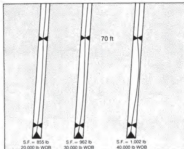
Fig. 8.133C—Tangency resulting from increasing WOB; 8\frac{1}{2} -in. hole, 6-in. collars, 10^\circ inclination, 70-ft tangency length.
