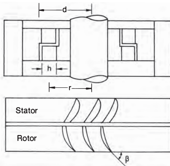
Fig. 8.105—Side view of a single-stage turbine. (after Jürgens 13 ).
