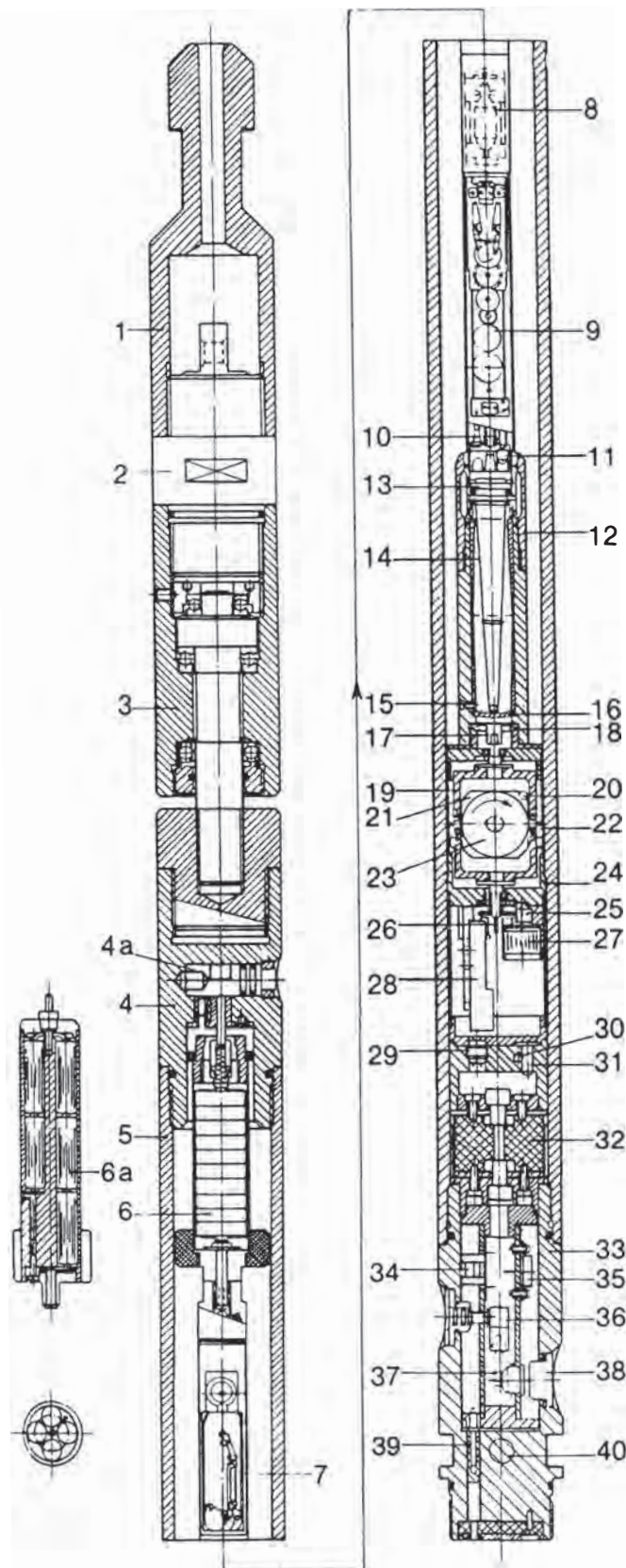
Fig. 8.69—Components of a gyroscope compass instrument (after Eikelberg et al. 8 ).
