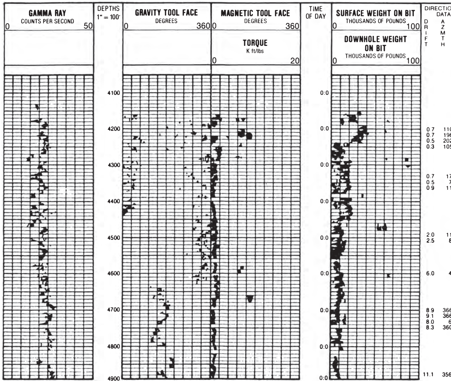
Fig. 8.61B—Typical multisensor MWD output.
