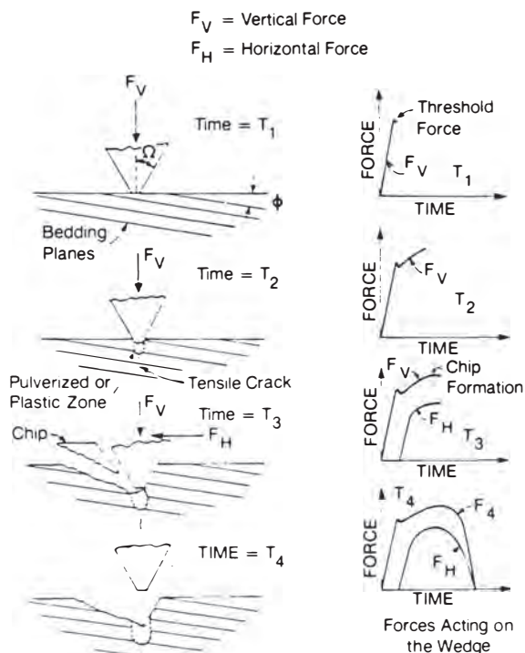
Fig. 8.159—Preferred chip formation model (after McLamore 30 ).
