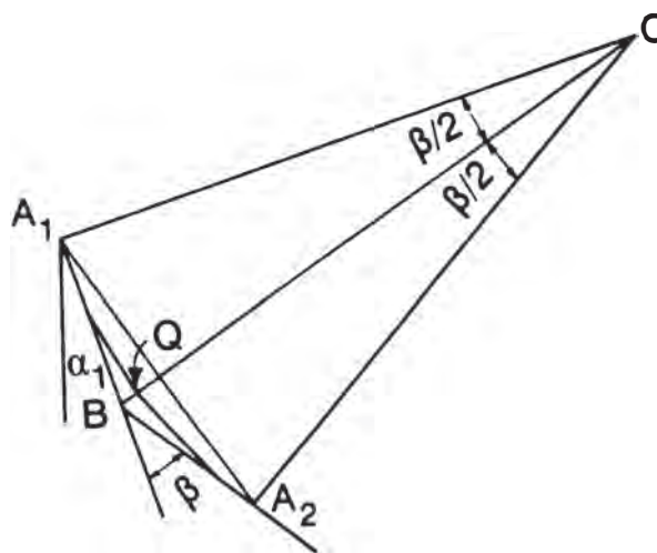
Fig. 8.21—Representation of minimum curvature ratio factor, F .
