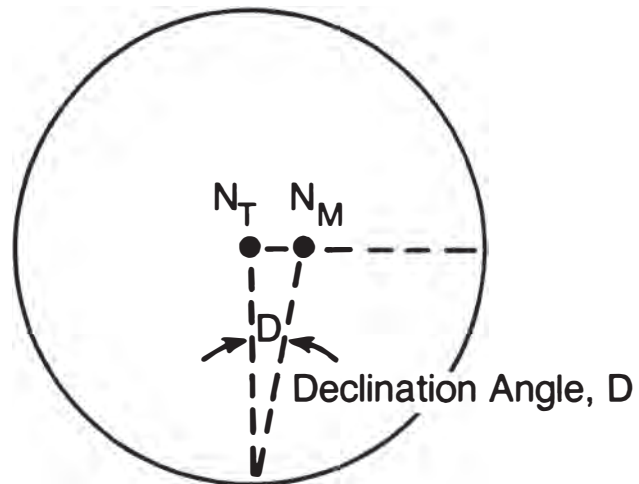
Fig. 8.63—Declination.
