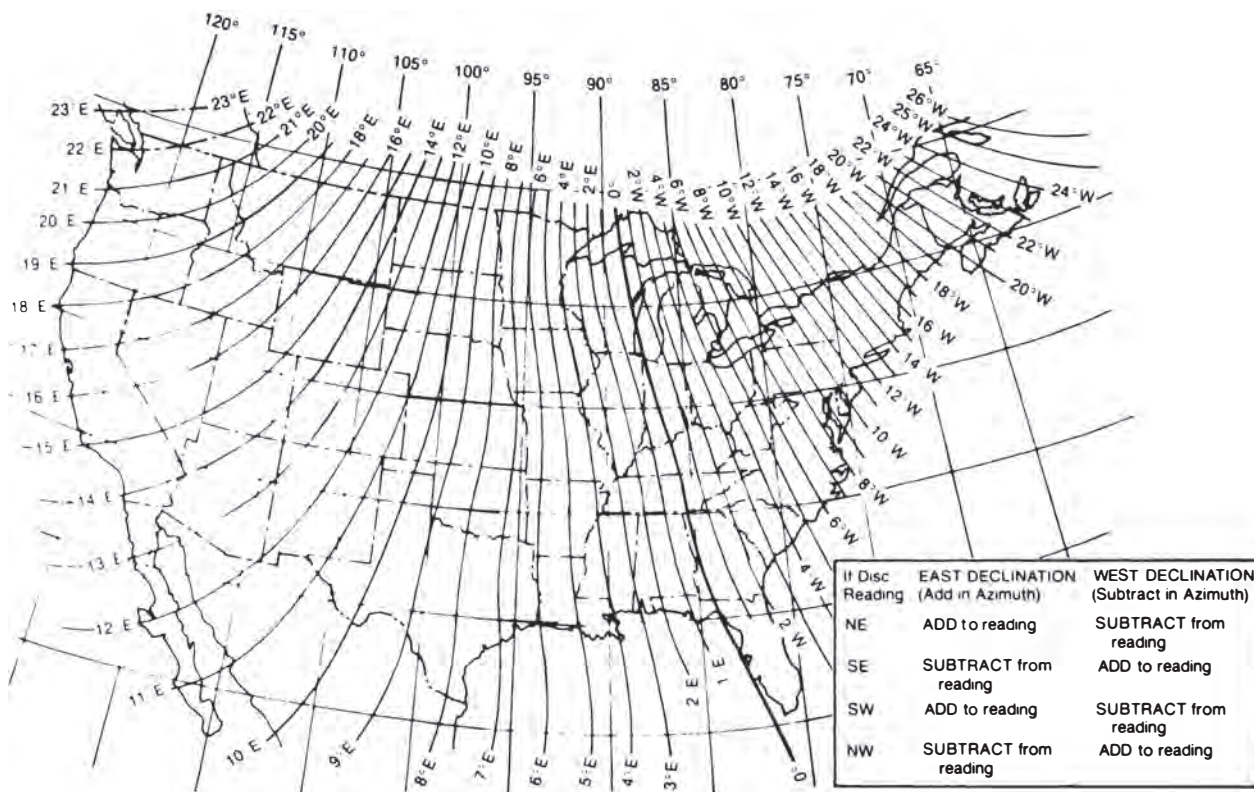
Fig. 8.64—Isogonic chart for the U.S.
