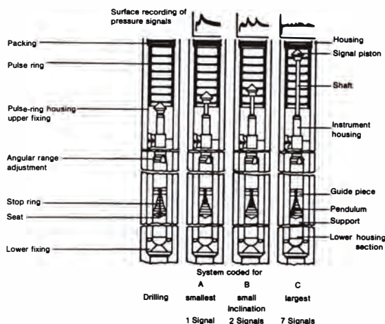
Fig. 8.58—Operation of a teledrift tool (after Eikelberg et al. 8 ).
