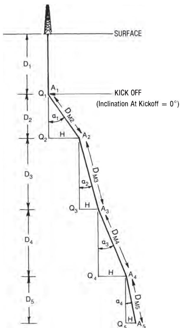
Fig. 8.17—Vertical calculation.
