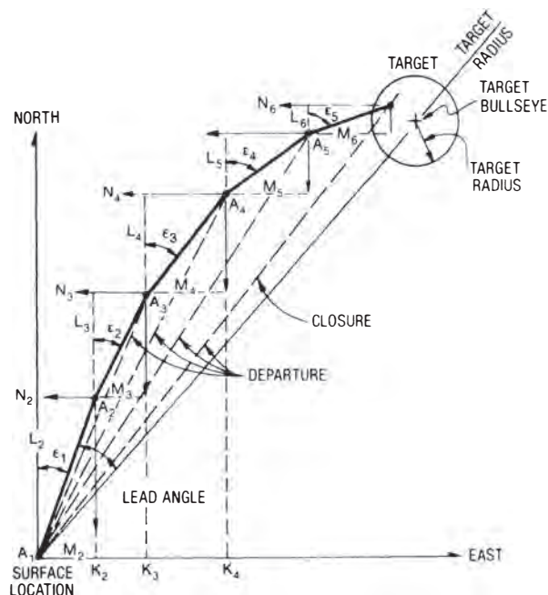
Fig. 8.18—Horizontal calculation.
