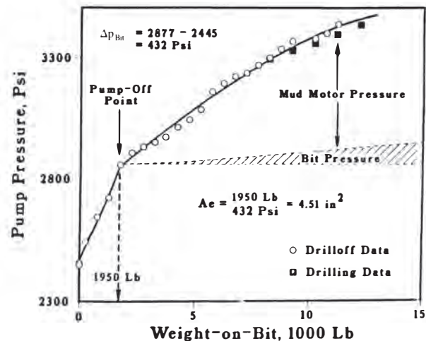
Fig. 8.111B—Point of pump-off (after Winters and Warren 16 ).
