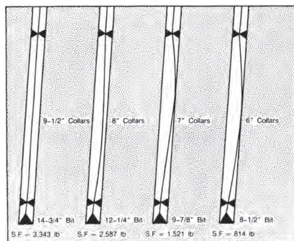
Fig. 8.133B—Tangency between bit and stabilizer; 90-ft building assembly, 10^\circ inclination, 30,000-lbf WOB.
