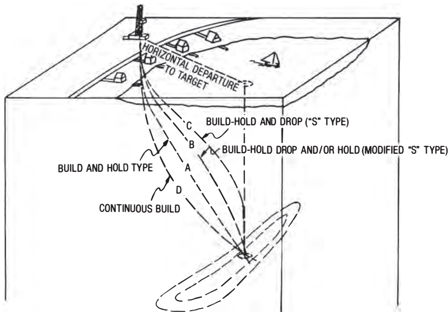
Fig. 8.8—Major types of wellbore trajectories.
