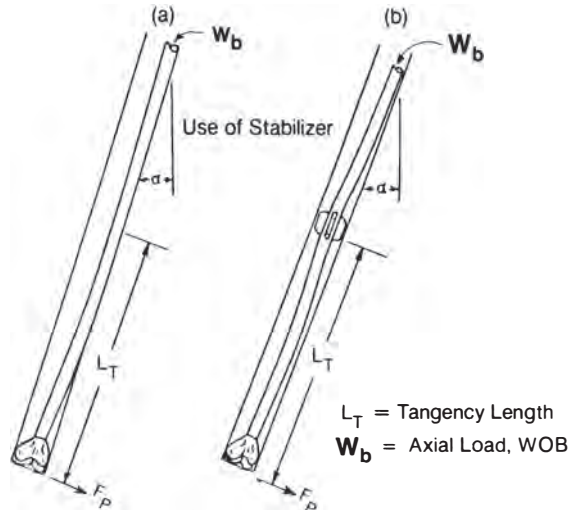
Fig. 8.125—Tangencies for slick and pendulum BHA's.
