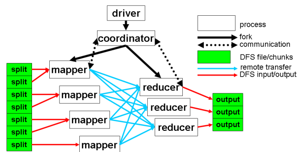
Figure 1: Data and control flow for Google’s Map-Reduce framework. A driver program initiates a coordinator process. It remotely forks many mappers, then reducers. Each mapper reads file splits from GFS, applies user-defined logic, and creates several output partitions, one for each reducer. A reducer reads remotely from every mapper, sorts, groups the data, applies user-defined logic, and sends outputs to GFS.
