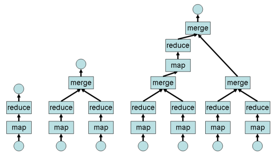
Figure 5: Map-Reduce-Merge workflows. The left is a typical 2-pass Map-Reduce workflow. The middle one is a typical 3-pass Map-Reduce-Merge workflow. The right is a multi-pass hierarchical workflow built with several Map, Reduce, and Merge modules.
