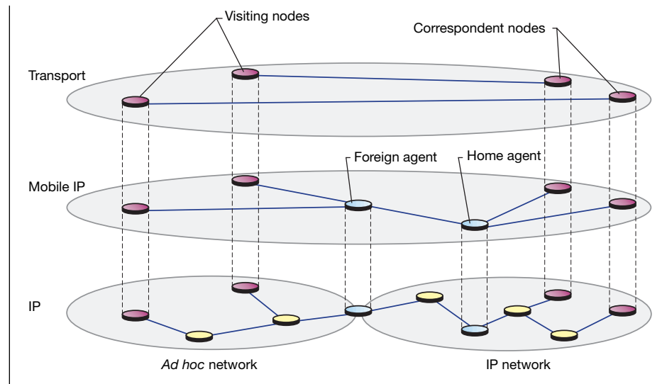
Figure 8 An overview of the MIPMANET architecture.
