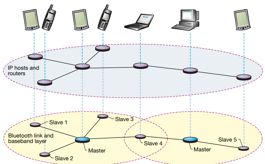
Figure 14 A Bluetooth scatternet where the networking functionality is handled within the IP layer (that is, by IP routing).
