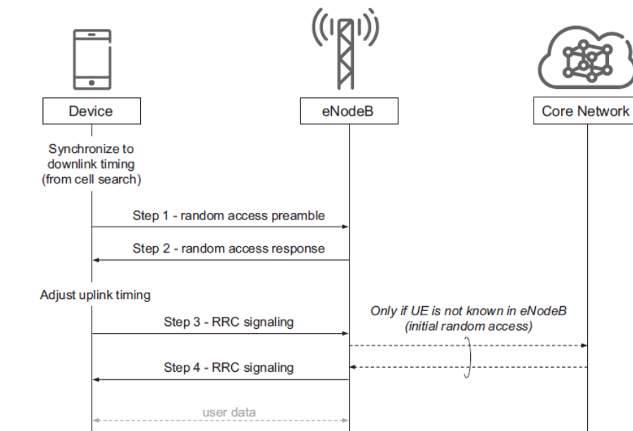
FIGURE 11.8 Overview of the random-access procedure.
