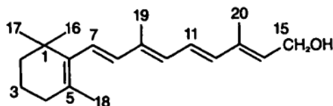
Scheme 1. Numbering system for retinol (vitamin A alcohol).
