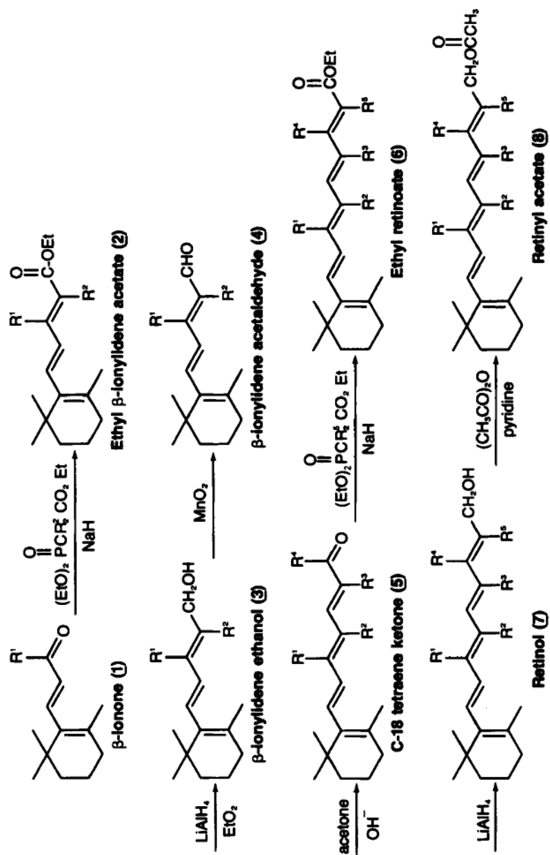
Scheme 2. Synthesis of deuterated forms of vitamin A.
