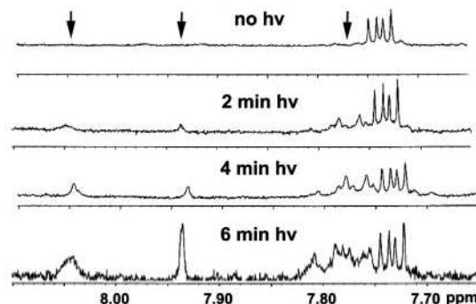
Fig. 9. ^1\text{H} NMR analysis of irradiated ATR dimer. ATR dimer was either unirradiated (no hv) or irradiated for 2, 4, or 6 min (430 nm, 0.19 mW/mm ^2 ). The presence of aromatic protons (arrows) upon blue-light exposure suggests aromatization of the central hexadiene core.
