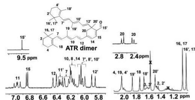
Fig. 2. ^1H NMR spectrum (400 MHz; CDCl_3 ) of the pigment in ATR-treated ROS that was isolated by using reverse-phase HPLC at a retention time of 6.95 min. Two sets of gem -dimethyl peaks on C1 and C1' were immediately suggestive of a dimerized retinal product and verified the structure as that of ATR dimer. The peaks are assigned based on the numbering shown with the structure. X, solvent impurities.
