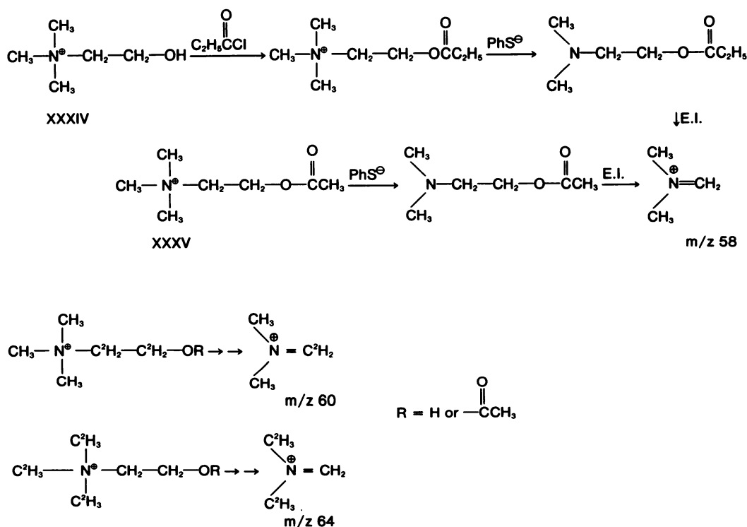
FIG. 2. A. Basis of the analytical method for the determination of choline (XXXIV) and acetylcholine (XXXV) by GC-MS. The structure of the ion with m/z 58, which represents the base peak in the EI mass spectrum of each compound, is as indicated. B. The consequence of deuterium substitution at specific sites in choline and acetylcholine on the m/z value of the fragment ion used in selected ion monitoring analyses.
