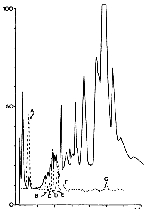
FIG. 8. Detection of ^{13}\text{C} -labelled metabolites in urine after administration of [ ^{13}\text{C} ]aspirin to a human subject. The effluent from the gas chromatograph is combusted to \text{CO}_2 and the ratio of ^{13}\text{CO}_2 : ^{12}\text{CO}_2 is determined by mass spectrometry. Solid trace: Gas chromatogram of methylated urinary extract. Broken trace: Ratio of m/z 45 ( ^{13}\text{CO}_2 ): 44 ( ^{12}\text{CO}_2 ) obtained from GC-MS analysis of the same sample. Reproduced with permission from M. Sano, Y. Yotsui, H. Abe, and S. Sasaki, Biomed. Mass Spectrom. 3: 1-3, 1976.
