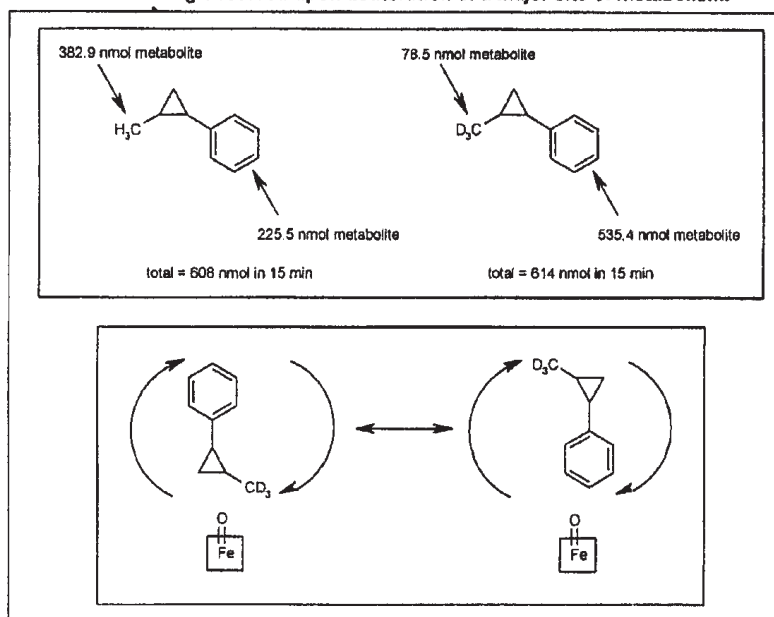
Figure 1. Schematic of metabolic switching observed upon deuteration of a major site of metabolism.
