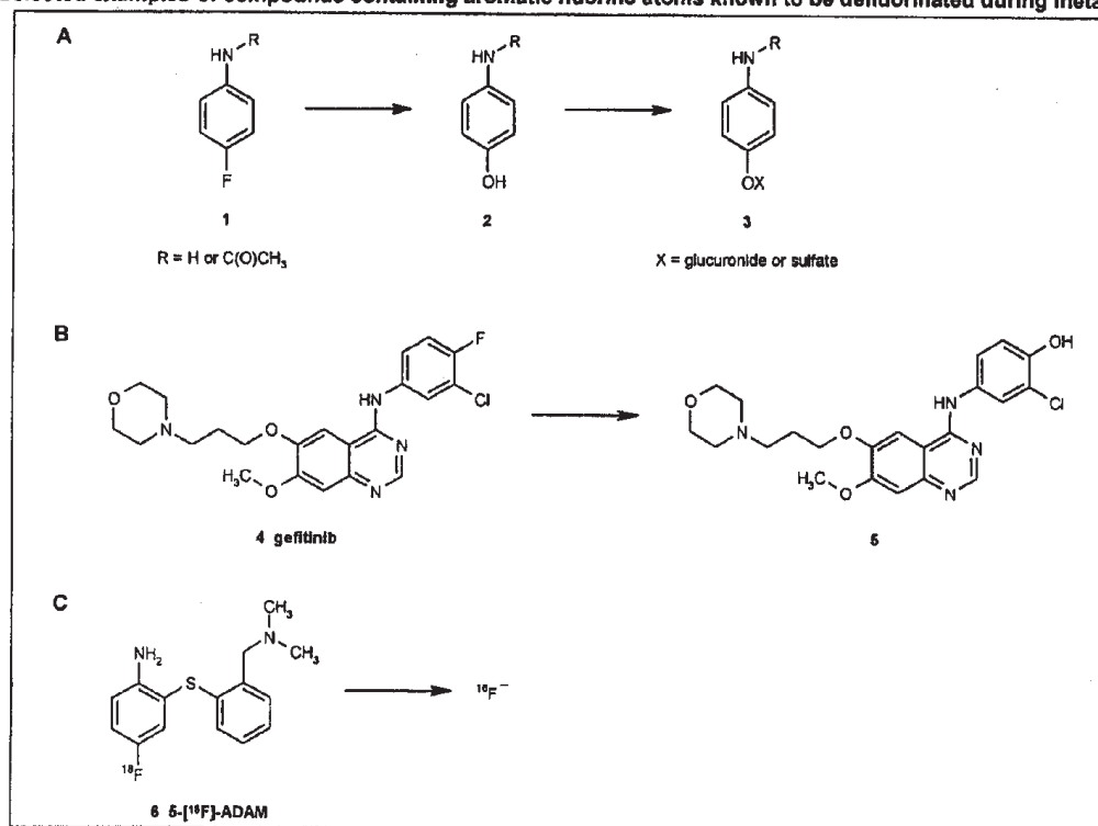
Figure 2. Selected examples of compounds containing aromatic fluorine atoms known to be defluorinated during metabolism.
