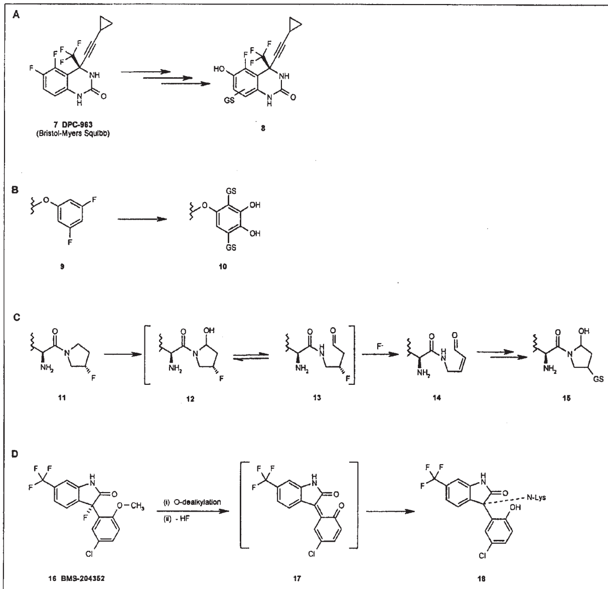
Figure 3. Selected examples of compounds containing aromatic and aliphatic fluorine atoms known to be defluorinated and conjugated with GSH.
