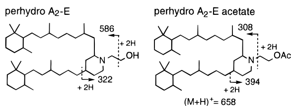
Figure 2. Major fragments observed 14a in FAB-CAD MS/MS of perhydro endogenous orange fluorophore and its acetate.
