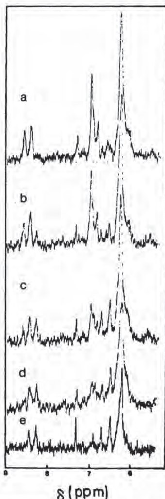
Figure 1. Vinyl proton NMR spectra of 0.14 M retinyl imines at 37 °C in chloroform- d containing 1% Me 4 Si (ppm from Me 4 Si): (a) 13- cis -retinylidene- n -butylimine; after (b) 37 min, (c) 3 h, (d) 6 h, (e) freshly prepared all- trans imine.
