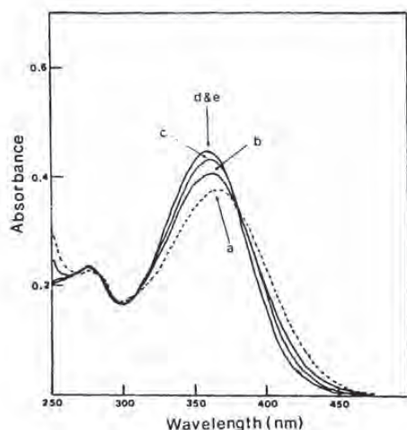
Figure 4. Electronic spectra showing the reaction between 9- cis -retinal (9.7 \mu M) and n -butylamine (100 mM) at 25 ^{\circ} C in chloroform: (a) 9- cis -retinal; formation of 9- cis imine. Hours after adding amine: (b) 0.5; (c) 1.0; (d) 6.0; (e) 30.
