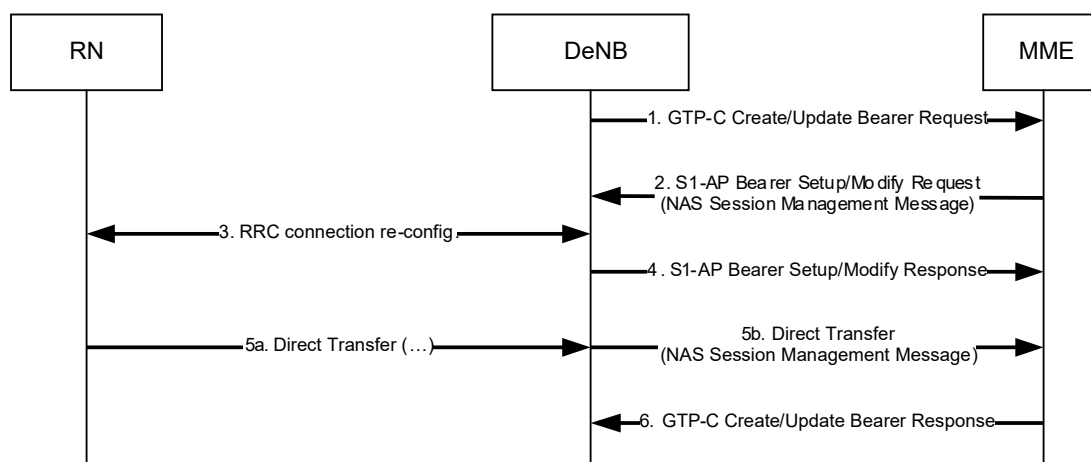
Figure 4.3.20.4-1: DeNB-initiated bearer activation/modification procedure
