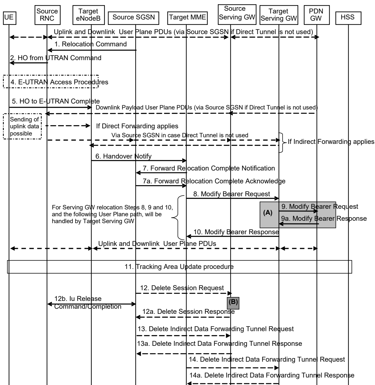
Figure 5.5.2.2.3-1: UTRAN Iu mode to E-UTRAN Inter RAT HO, execution phase
