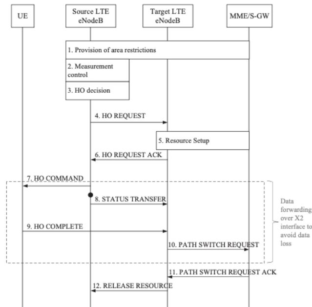
Figure 2.19: X2-based handover procedure.
