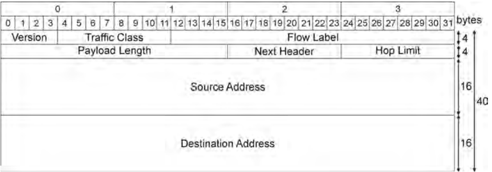
Figure 1.81 IPv6 header format.
