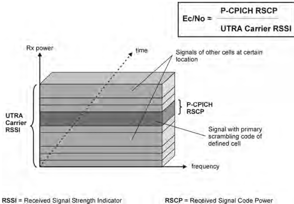
Figure 4.11 CPICH E_c/N_0 measurement in 3G FDD UMTS.
