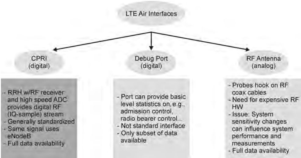
Figure 4.2 Strategies to monitor the air interface.
