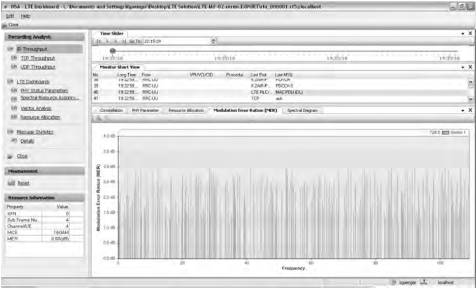
Figure 4.28 Modulation error ratio for LTE spectrum.
