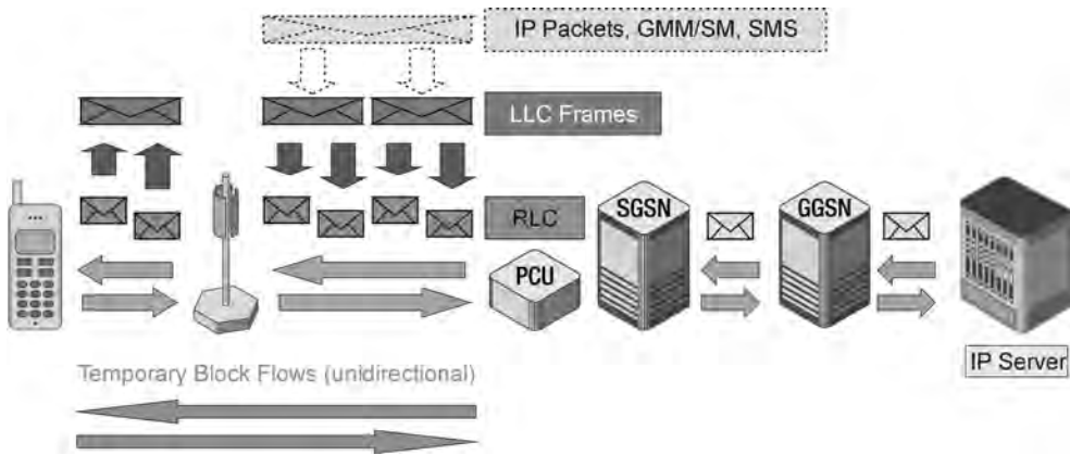
Figure 1.2 Packet data transfer in 2.5G GPRS across Radio and Abis interfaces.
