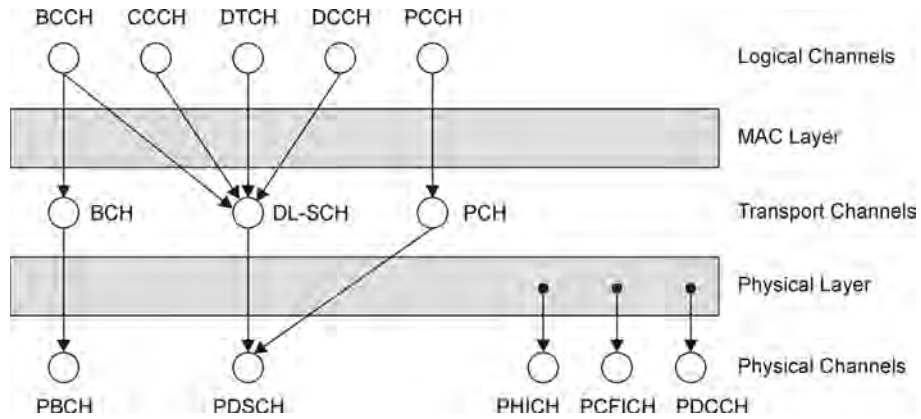
Figure 1.64 Downlink channel mapping and multiplexing from logical channels via transport channels to physical channels.
