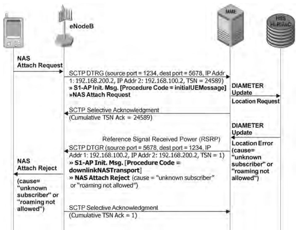
Figure 4.32 Failed attach due to failed update location in HSS.
