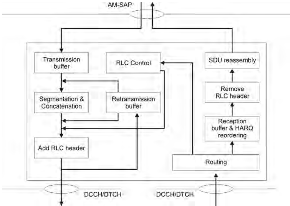
Figure 1.92 Model of an Acknowledged Mode entity. Reproduced with permission from © 3GPP™.
