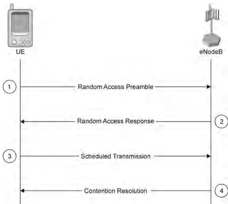
Figure 1.67 Contention-based random access procedure (TS36.300). Reproduced with permission from © 3GPP™.
