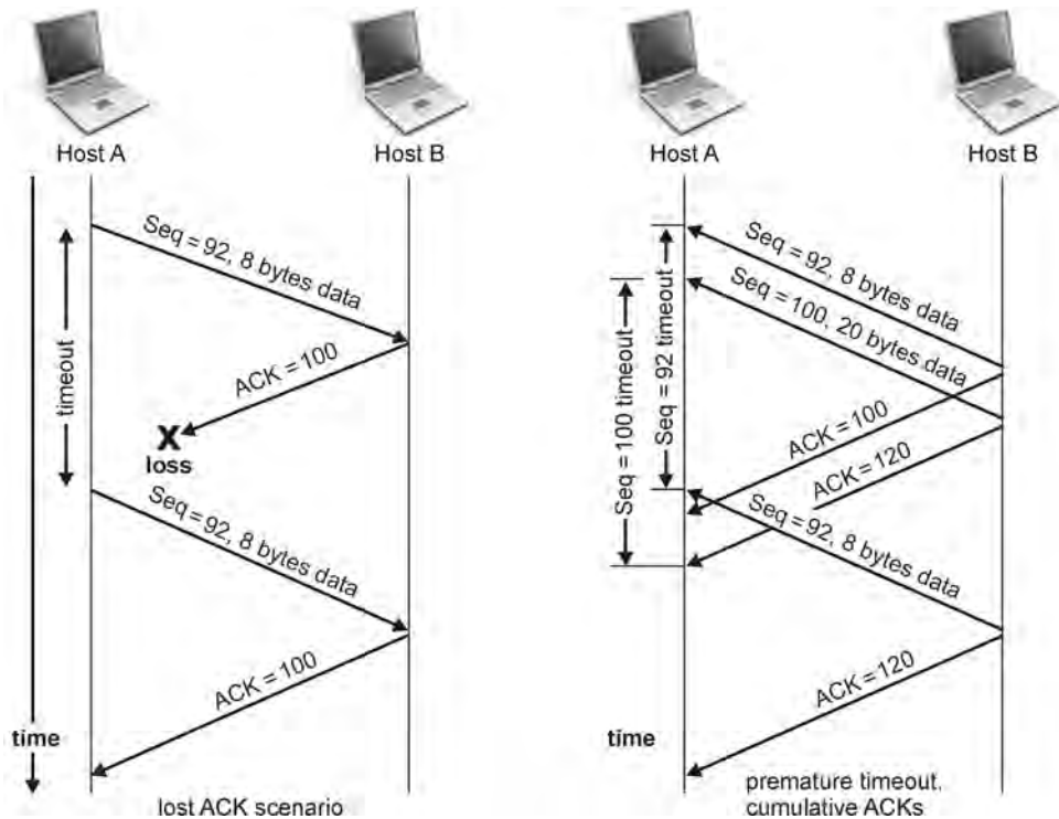
Figure 1.105 TCP retransmission scenarios.
