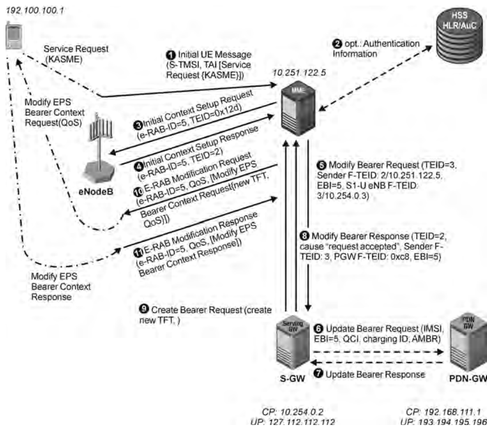
Figure 2.7 Service request after UE context release. (Tektronix Communications).
