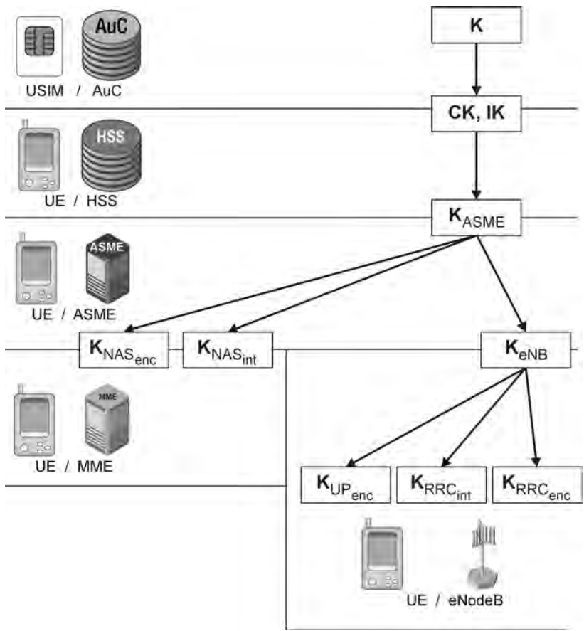
Figure 1.25 LTE security key hierarchy (according to 3GPP 33.401). Reproduced with permission from © 3GPP™.
