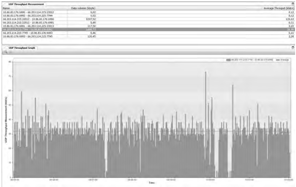
Figure 4.43 UDP throughput of a connection between two terminal endpoints as measured on S1-U interface.
