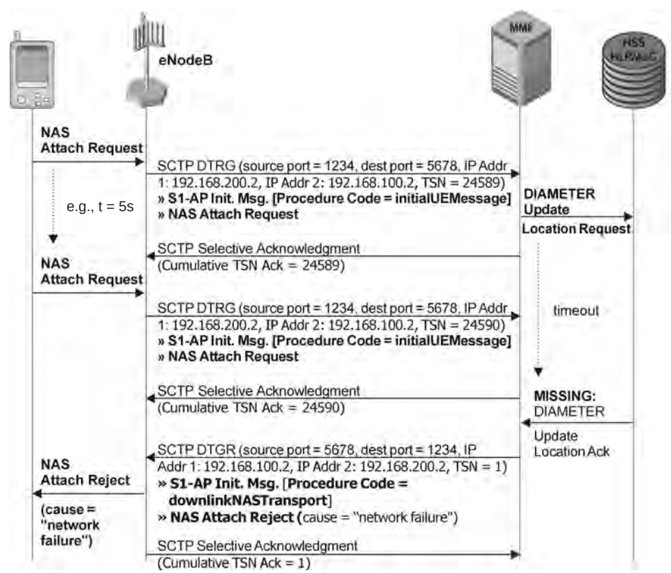
Figure 4.33 Network failure in attach procedure due to EPC latency.
