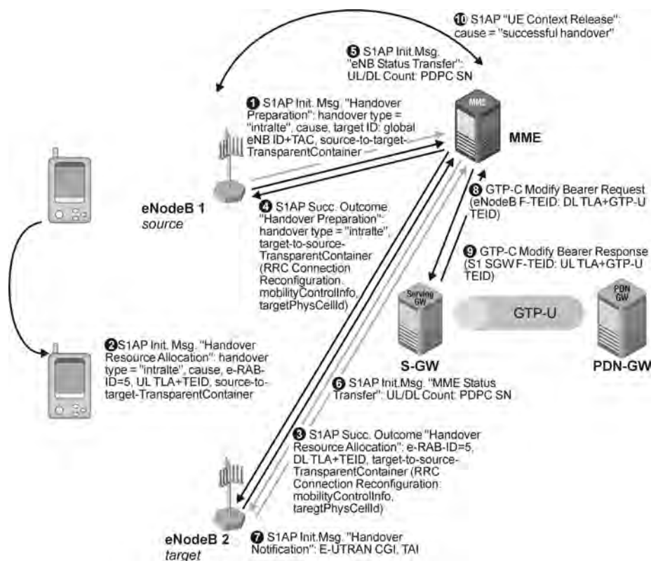
Figure 2.12 S1 handover message flow. (Tektronix Communications).
