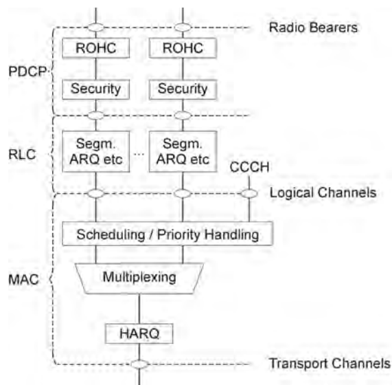
Figure 1.85 Layer 2 structure for UL (TS36.300). Reproduced with permission from © 3GPP™.
