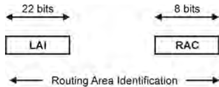
Figure 1.19 Structure of routing area identification (according to 3GPP 23.303). Reproduced with permission from © 3GPP™.
