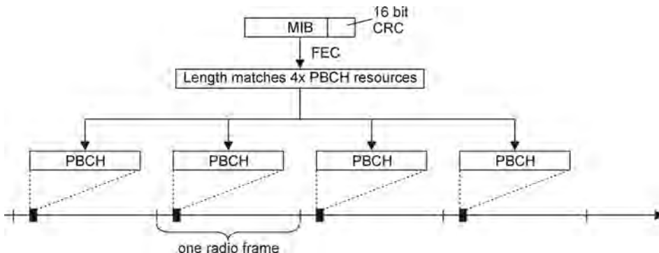
Figure 1.57 Master information block encoding and mapping to four DL radio frames.
