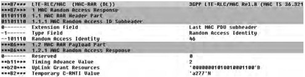
Figure 1.68 Example RAR message.
