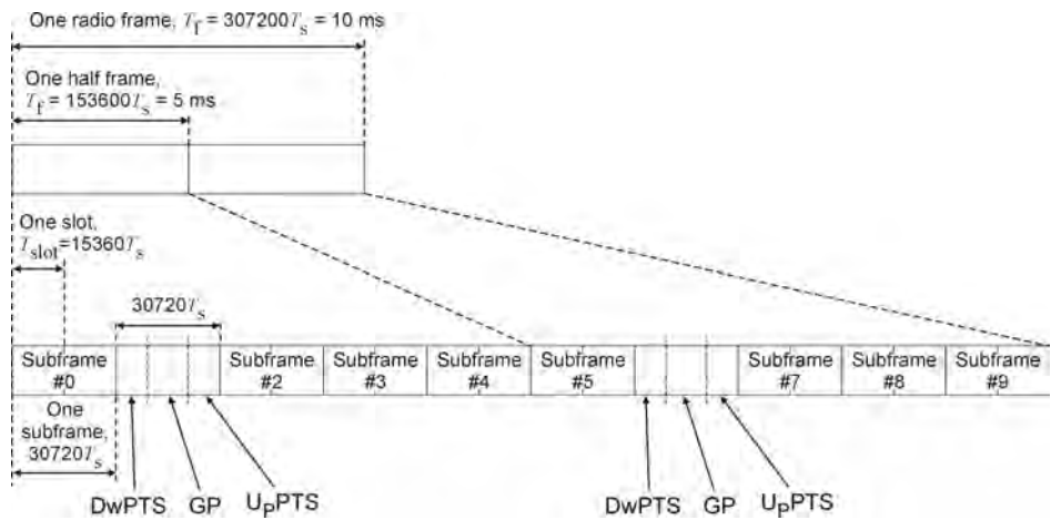
Figure 1.45 Frame structure type 2 used with TDD (for 5 ms switch-point periodicity) (TS36.211). Reproduced with permission from © 3GPP™.
