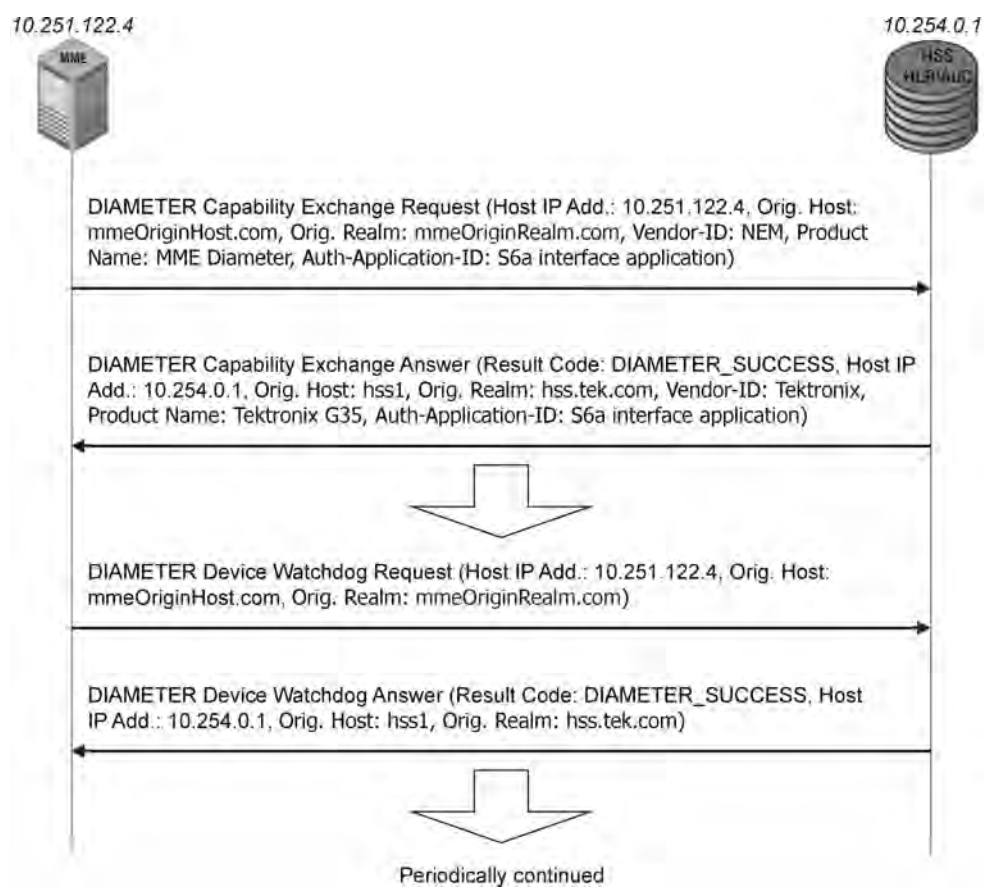
Figure 1.107 MME startup and activity check on S6a reference point.
