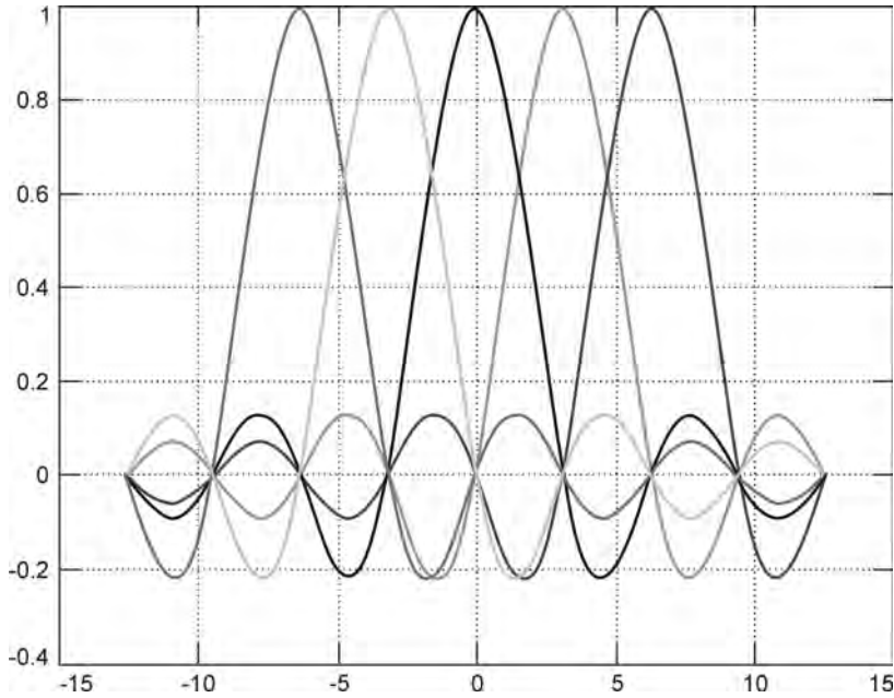
Figure 1.37 OFDM signal of orthogonal Si functions (subcarriers); subcarriers do not interfere because at each subcarrier the signals from other subcarriers are zero.
