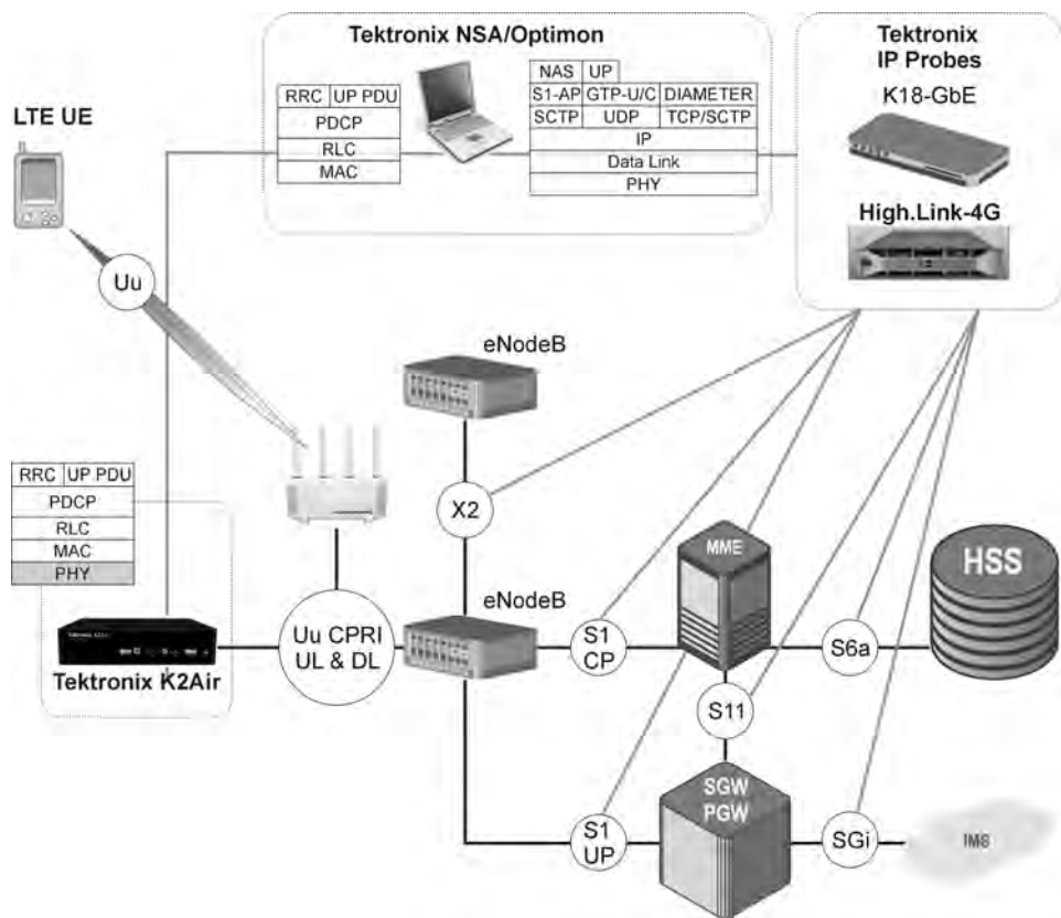
Figure 4.1 Monitoring architecture of a LTE network with fixed line interfaces (subset) and air interface.
