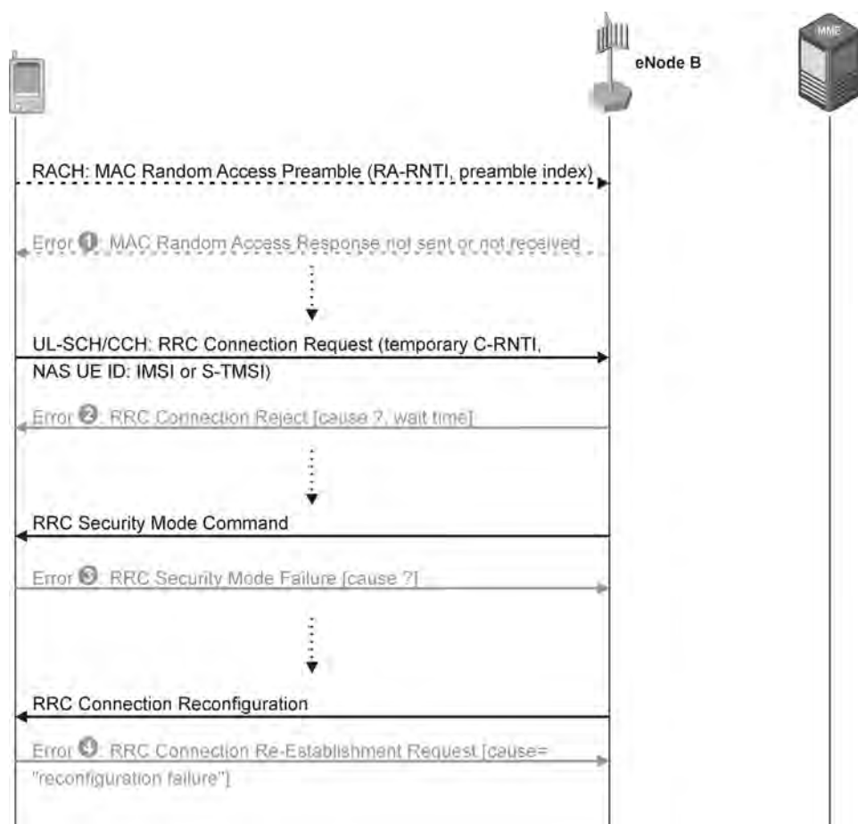
Figure 3.6 Errors during RRC connection setup and default radio bearer setup. (Tektronix Communications).
