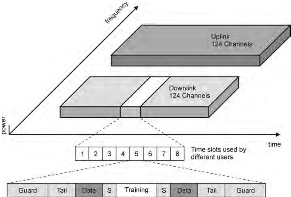
Figure 1.33 Schematic example of a Time Division Multiple Access (TDMA) system.
