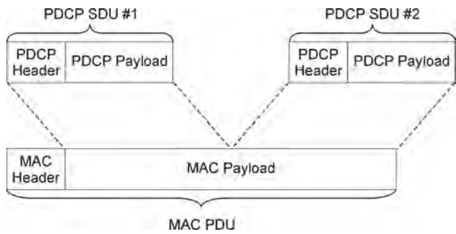
Figure 1.90 Example of RLC concatenation of several PDCP SDUs into one MAC PDU.
