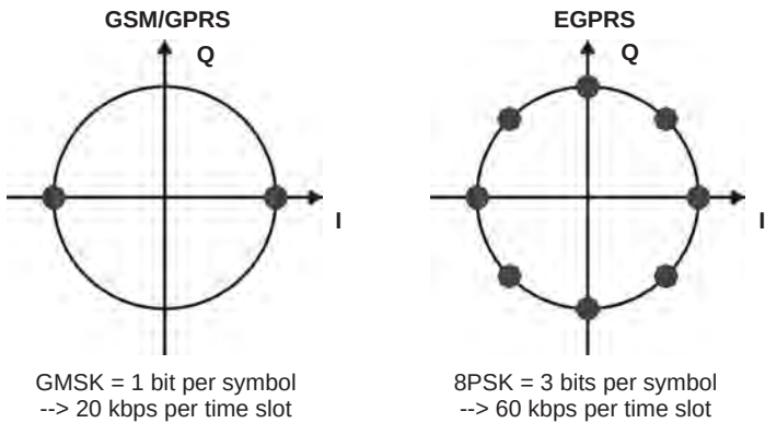
Figure 1.4 GSM/GPRS vs. EGPRS modulation.
