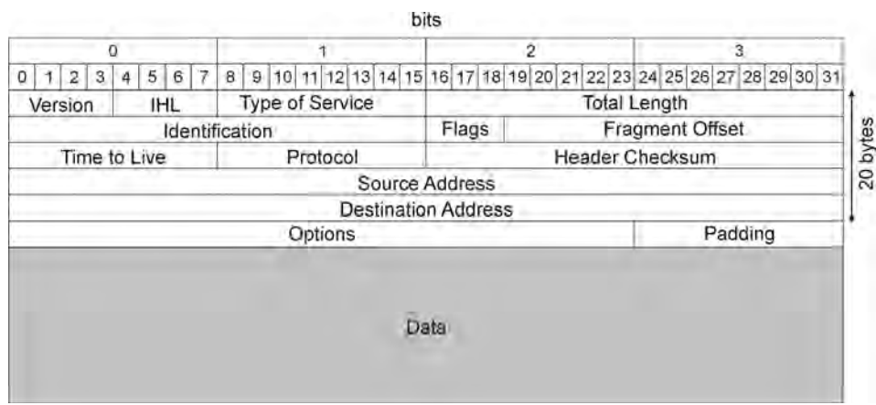
Figure 1.78 IP datagram structure.
