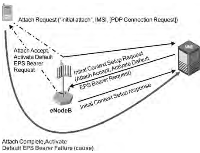
Figure 4.35 Activate Default EPS Bearer Failure.
