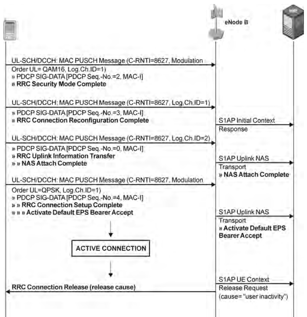
Figure 3.5 RRC connection setup 3/3 and RRC connection release. (Tektronix Communications).
