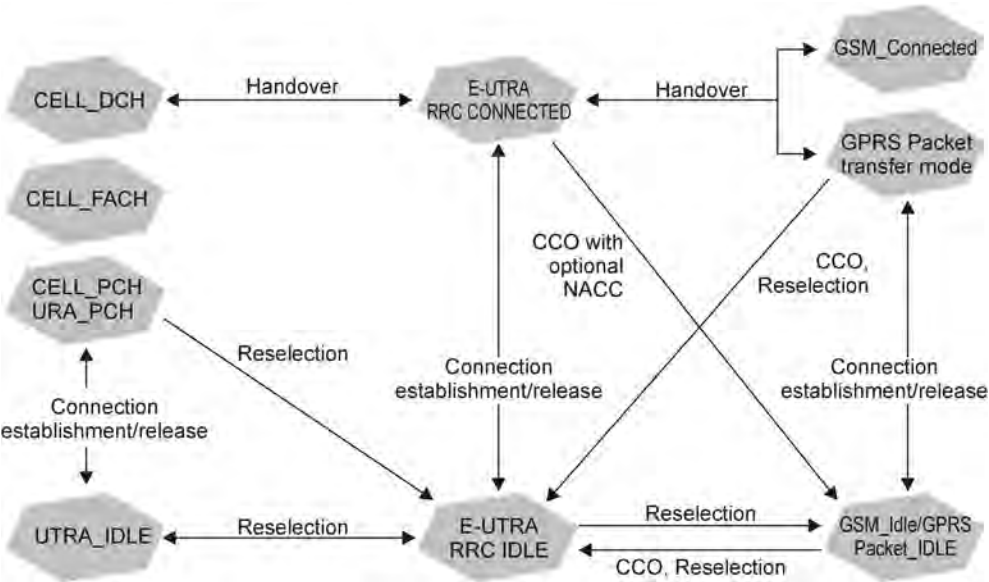
Figure 1.96 RRC state transitions in case of inter-RAT mobility. Reproduced with permission from © 3GPP™.
