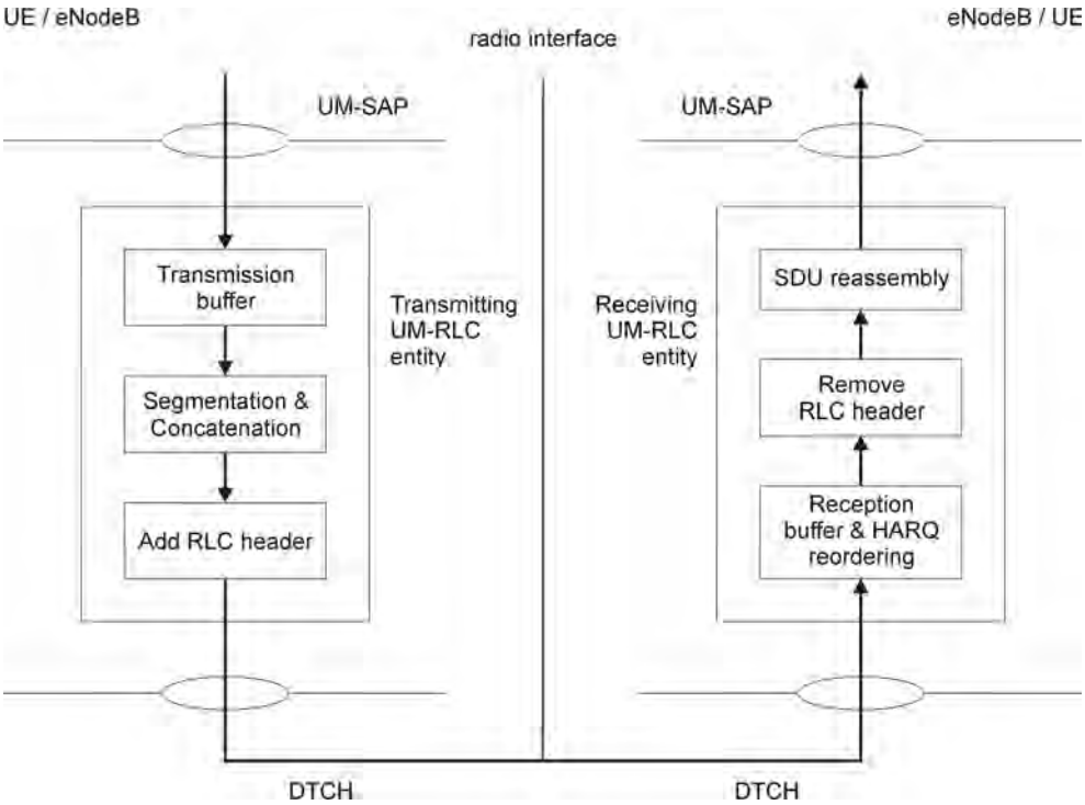
Figure 1.91 Model of two Unacknowledged Mode peer entities. Reproduced with permission from © 3GPP™.
