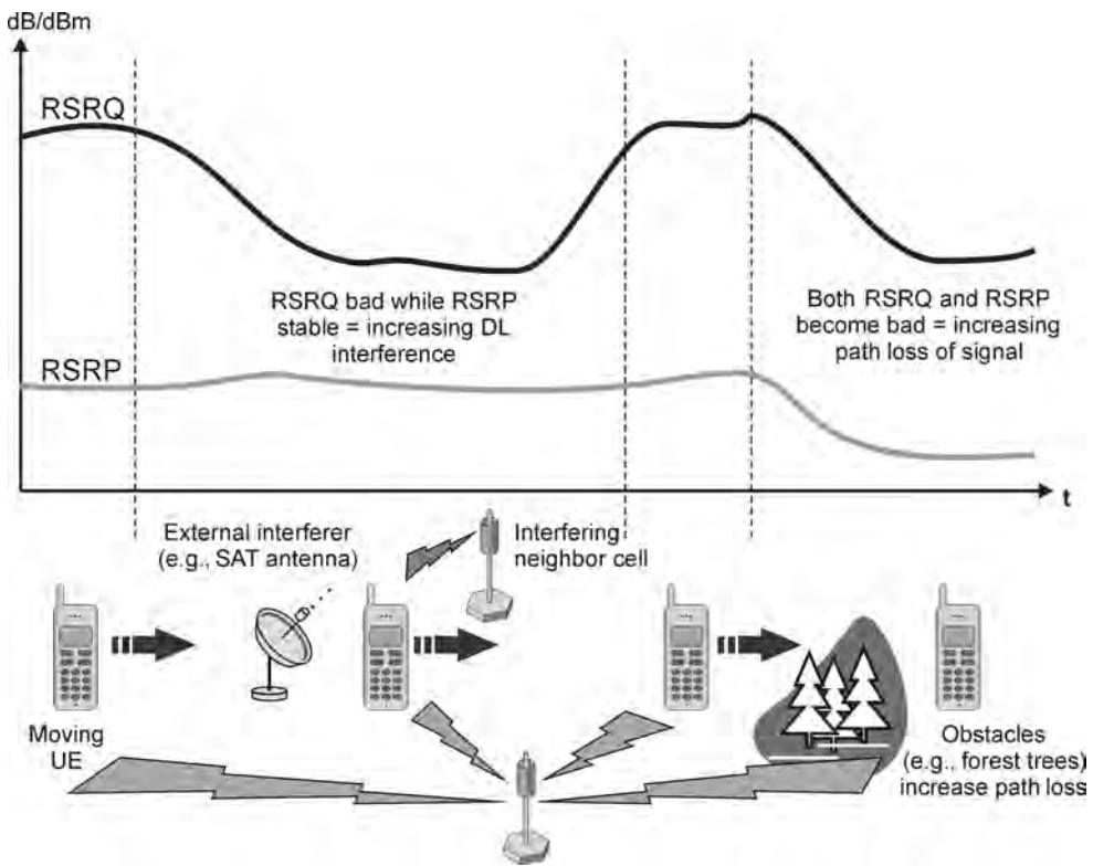
Figure 4.18 LTE coverage and interference problems.
