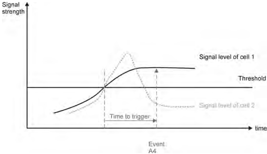
Figure 1.99 Time-to-trigger parameter for RRC measurements.
