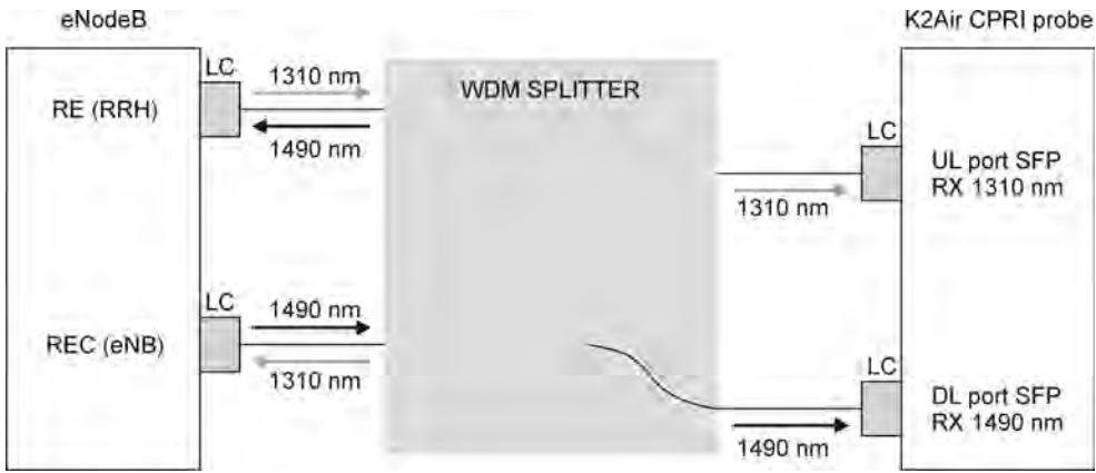
Figure 4.7 WDM CPRI architecture with one fiber for uplink and downlink. LC = Lucent or Local Connector; SFP = Small Form-Factor Pluggable (fiber optic module).
