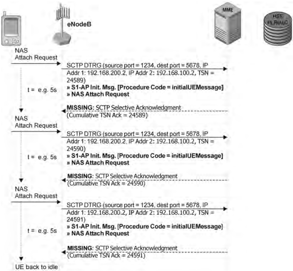
Figure 1.83 Failure in SCTP signaling transport.
