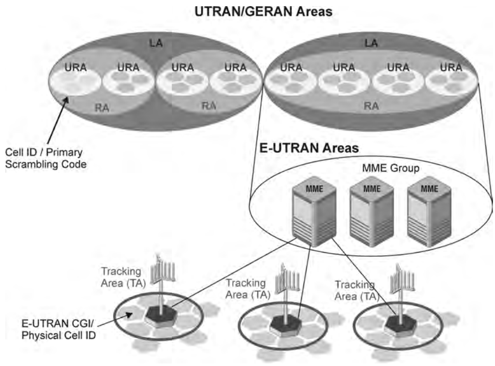
Figure 1.20 Areas in UTRAN/GERAN and E-UTRAN.
