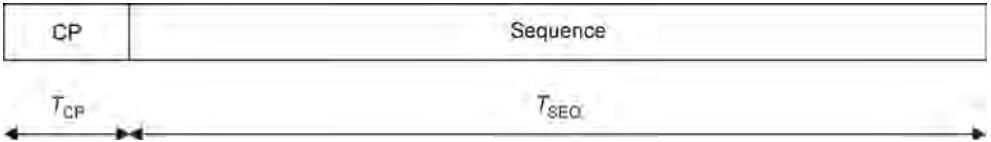
Figure 1.63 Random access preamble format (TS36.211). Reproduced with permission from © 3GPP™.
