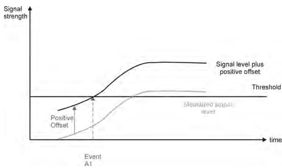
Figure 1.98 Offset parameter for RRC measurements.
