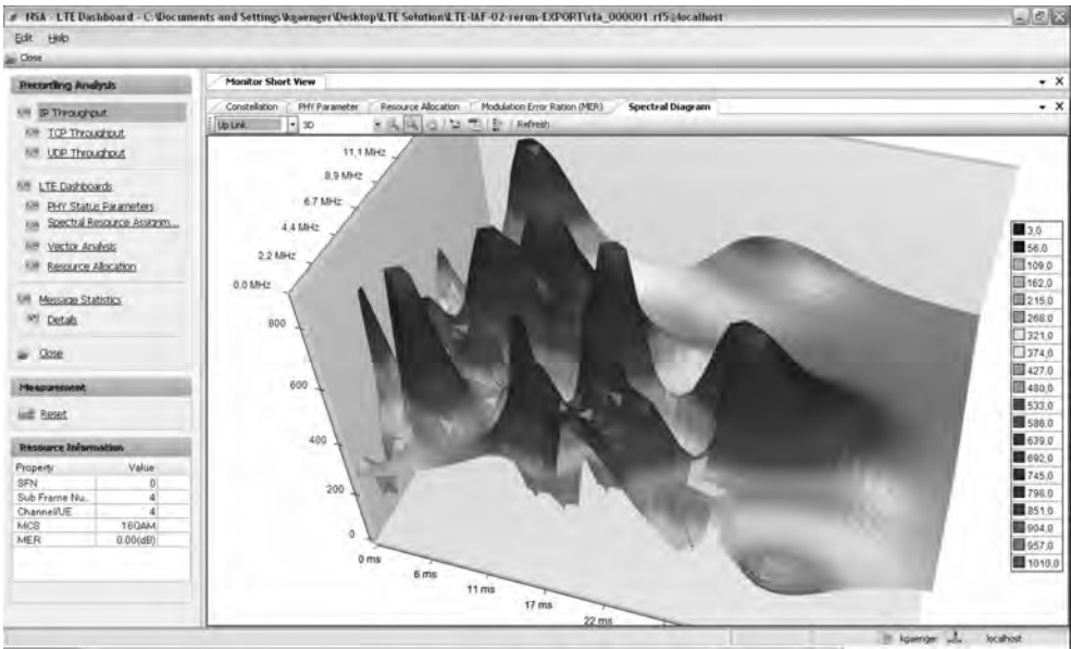
Figure 4.24 Channel baseband power measurement graph.
