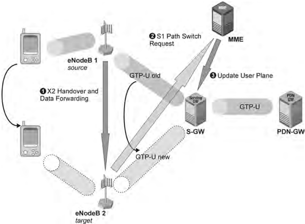
Figure 2.9 Inter-eNodeB handover over X2 – overview. (Tektronix Communications).
