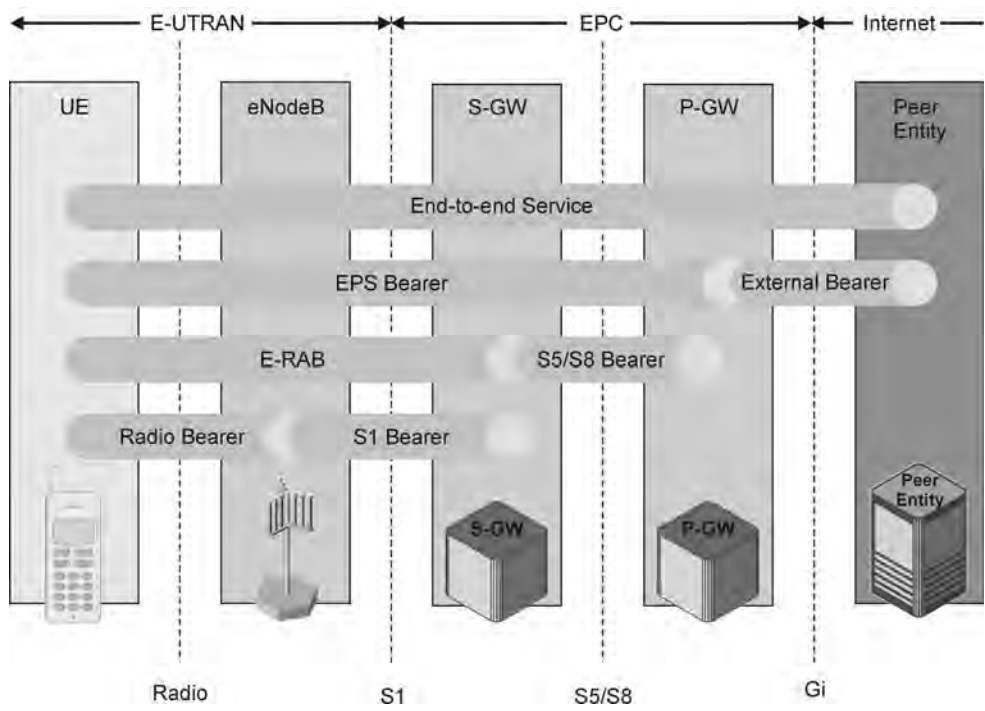
Figure 1.24 LTE QoS architecture (according to 3GPP 23.401). Reproduced with permission from © 3GPP™.
