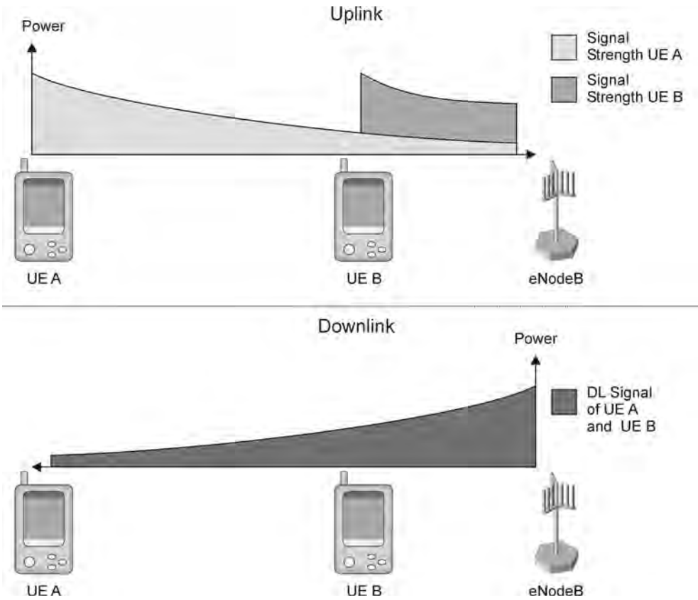
Figure 1.55 Near-far effect occurring in uplink direction, compared to equal signal strength reception in downlink.
