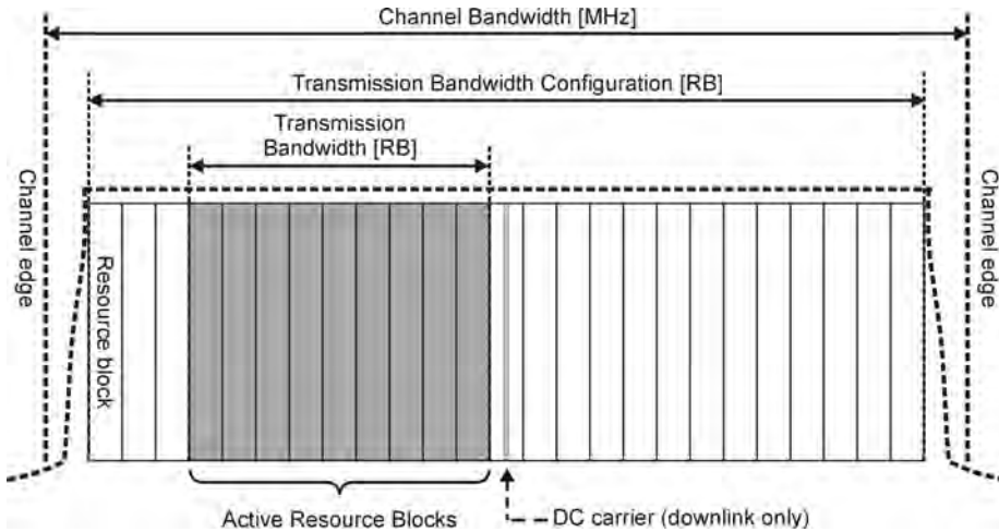
Figure 3.4 Transmission bandwidth (3GPP 36.104).
