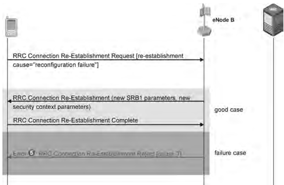
Figure 3.7 Successful/unsuccessful RRC connection re-establishment. (Tektronix Communications).
