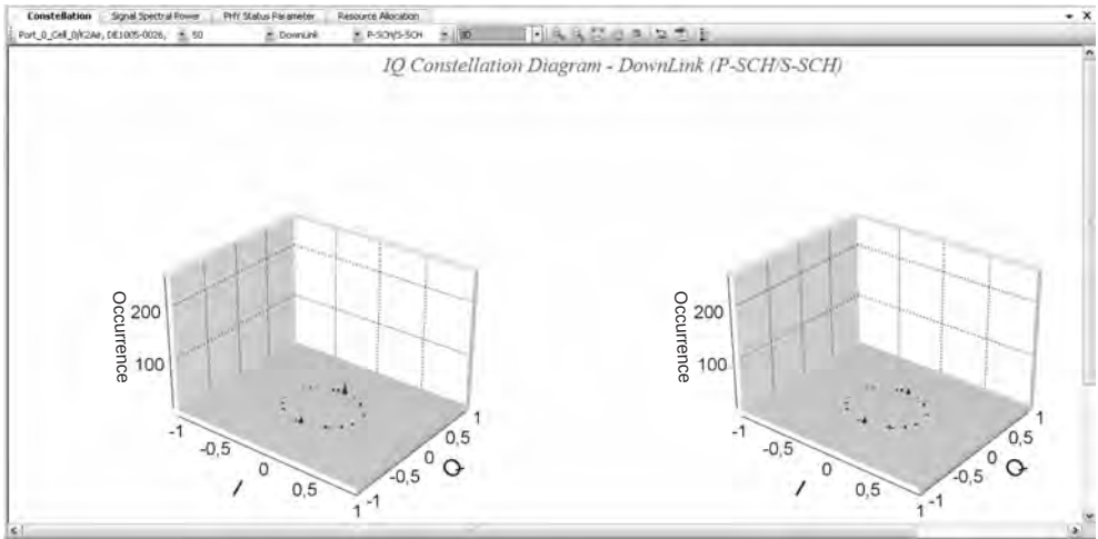
Figure 1.62 Vector IQ analysis of a primary and secondary synchronization signal on two transmit antennas.
