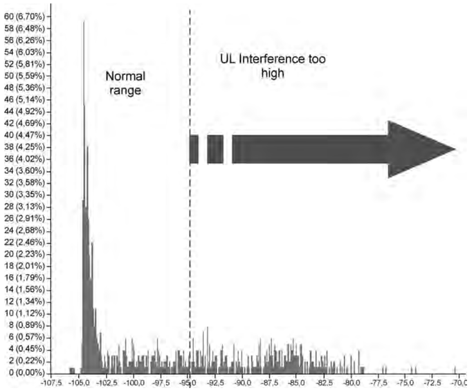
Figure 4.13 Statistical outliers in a histogram for received total wideband power.
