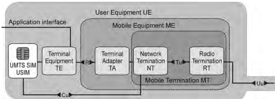
Figure 1.23 Modular architecture of a UE.
