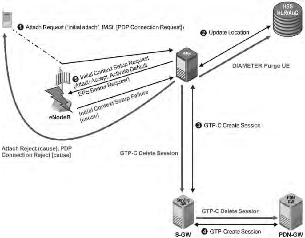
Figure 4.34 Initial context setup failure during initial attach.
