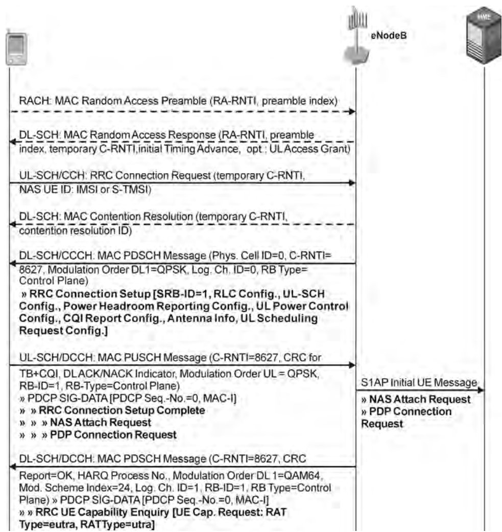
Figure 3.2 RRC connection setup procedure 1/3. (Tektronix Communications).
