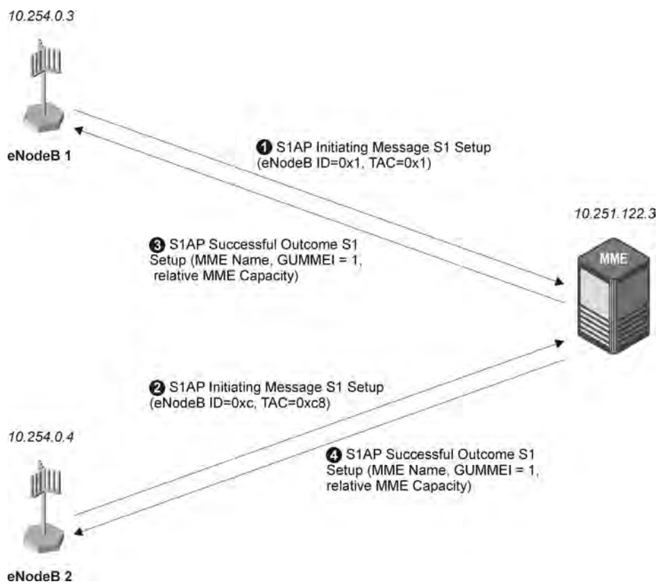
Figure 2.2 S1 Setup for two different eNodeBs. (Tektronix Communications).
