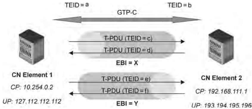
Figure 1.102 GTP tunnel management.
