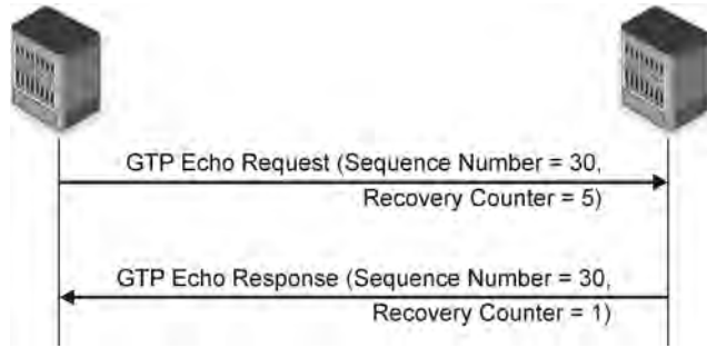
Figure 1.101 GTP path management.
