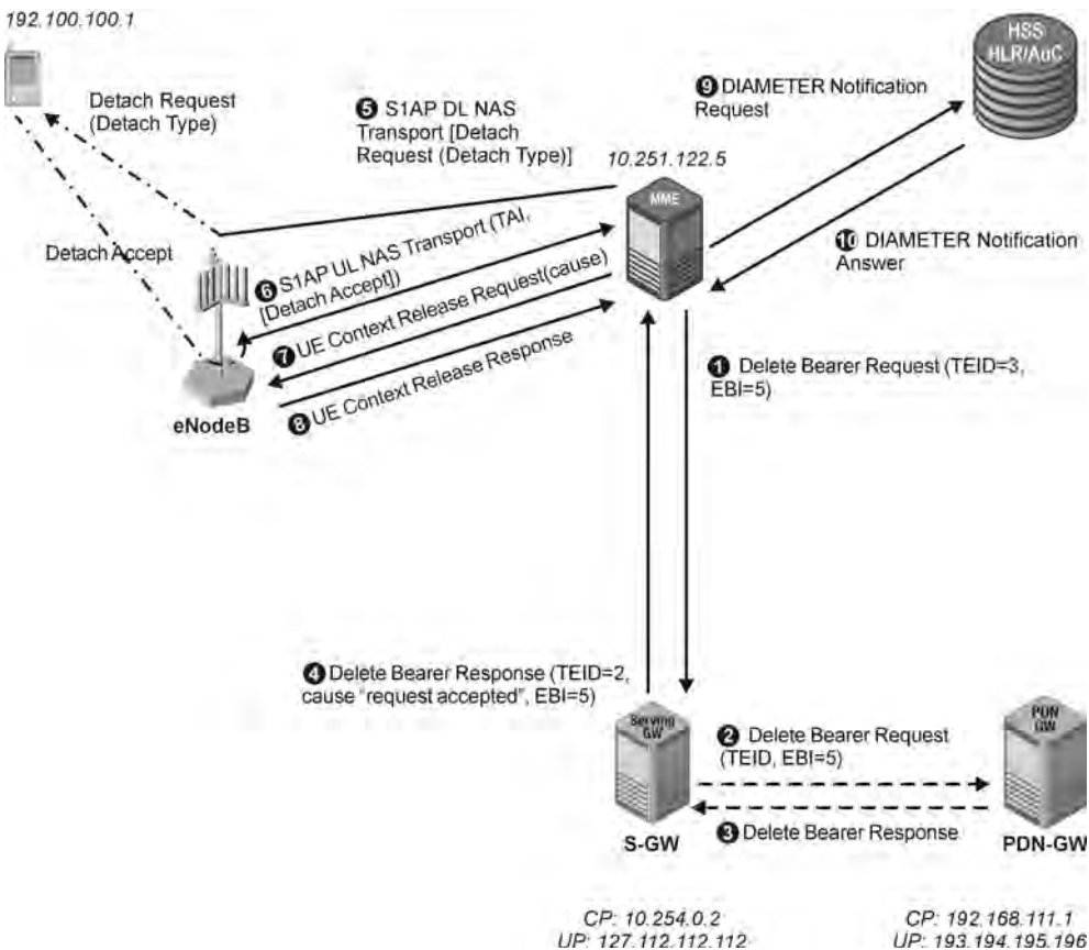
Figure 2.14 Detach (network initiated). (Tektronix Communications).
