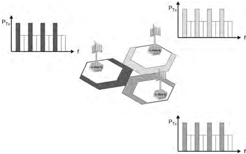
Figure 4.12 Partial frequency reuse to provide better signal quality for users at the cell edge on the downlink.
