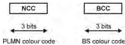
Figure 1.22 Structure of BSIC (according to 3GPP 23.303). Reproduced with permission from © 3GPP™.
