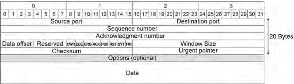
Figure 1.103 TCP header format.
