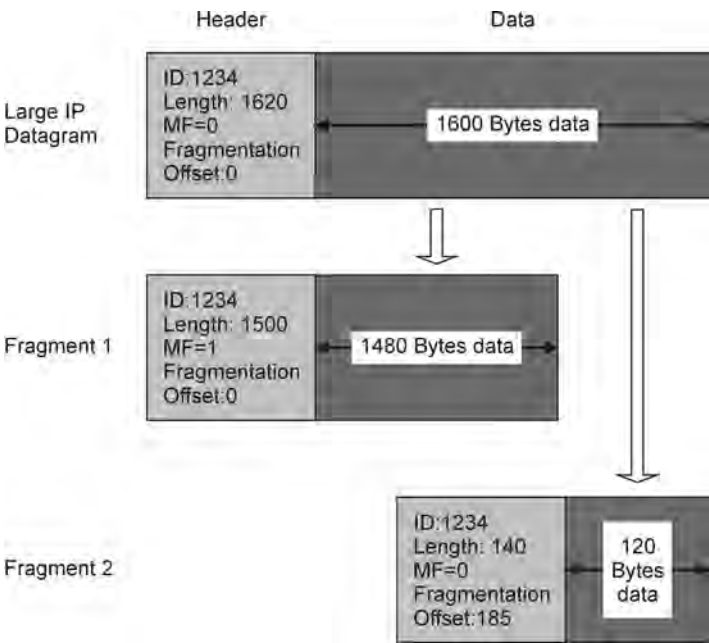
Figure 1.79 IP fragmentation.
