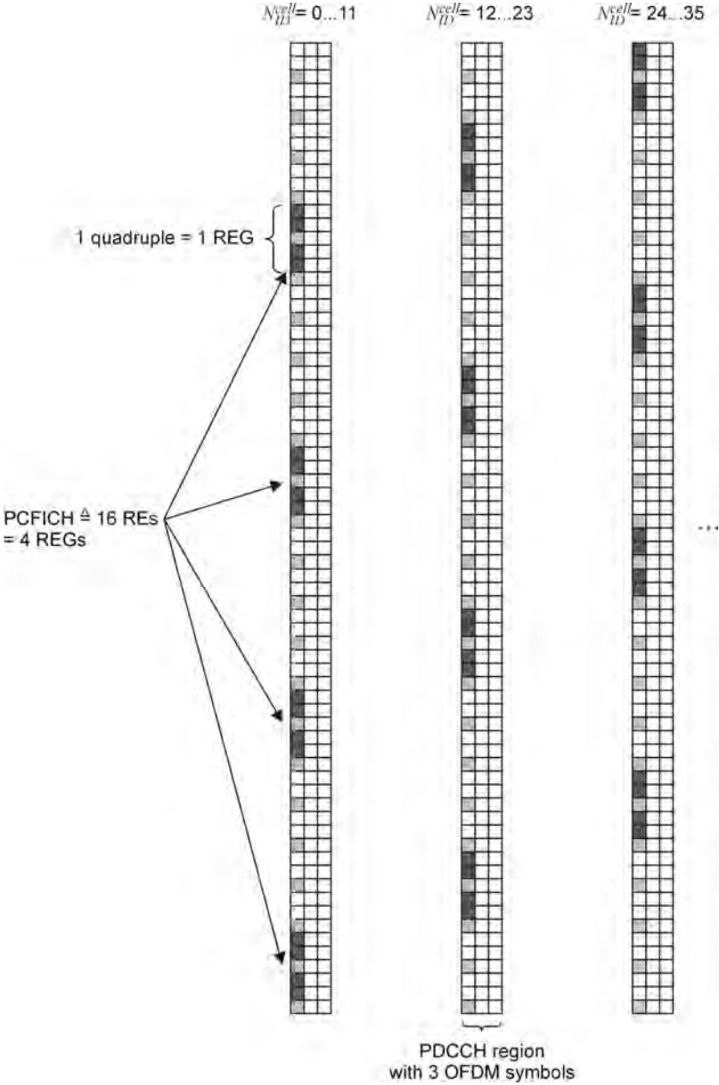
Figure 1.59 Mapping examples of PCFICH into resource element groups (always within the first OFDM symbol of a subframe) within the PDCCH area. Reproduced with permission from Nomor.
