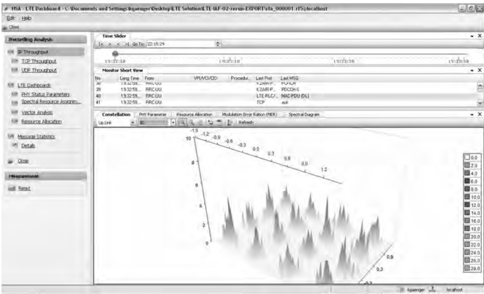
Figure 4.26 Three-dimensional I/Q constellation diagram.
