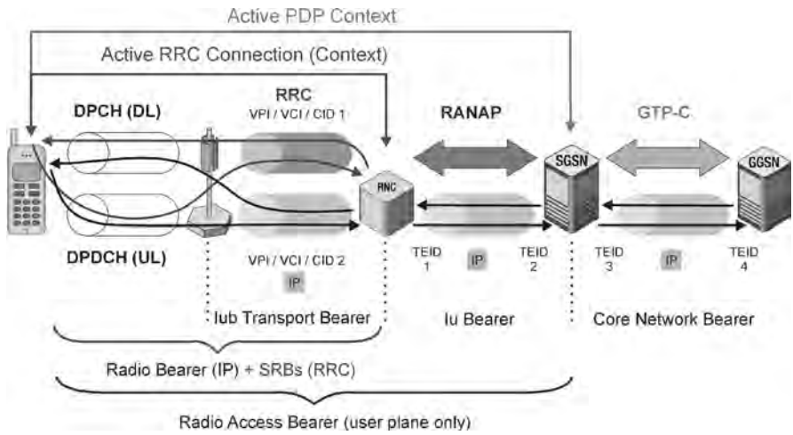
Figure 1.7 IP payload transmission using Release 99 bearers with UE in CELL_DCH state.
