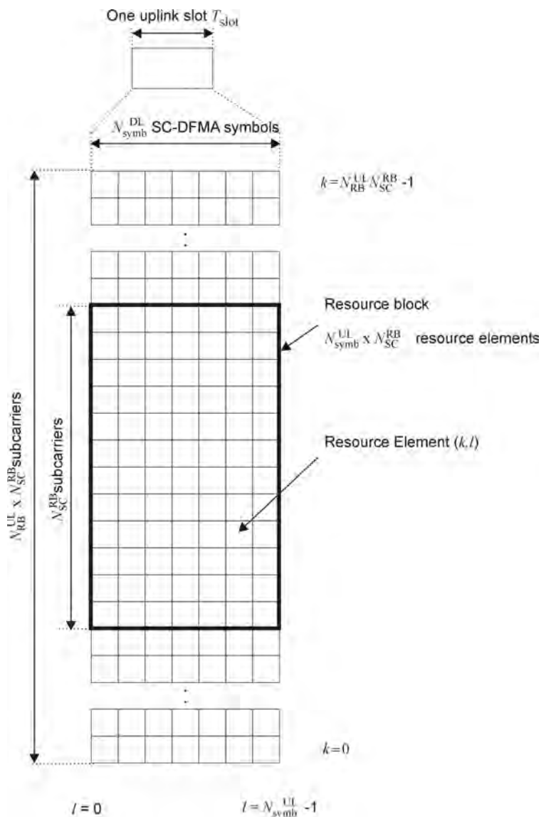
Figure 1.53 Uplink resource grid showing on UL RB. Reproduced with permission from © 3GPP™.
