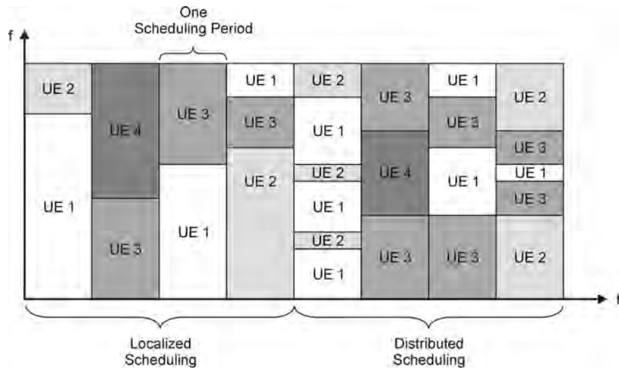
Figure 1.40 Localized vs. distributed shared channel scheduling.
