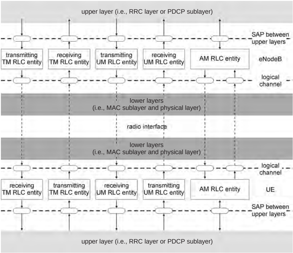
Figure 1.87 RLC layer overview with TM, UM, and AM RLC entities. Reproduced with permission from © 3GPP™.
