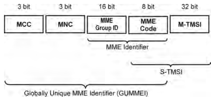
Figure 1.16 Format of GUTI and S-TMSI.
