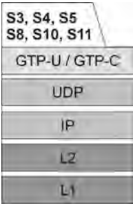
Figure 1.75 Protocol stack S3S4/S5/S8/S10/S11.
