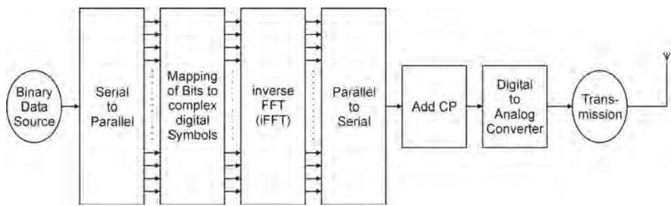
Figure 1.36 Block diagram of OFDM signal generation.
