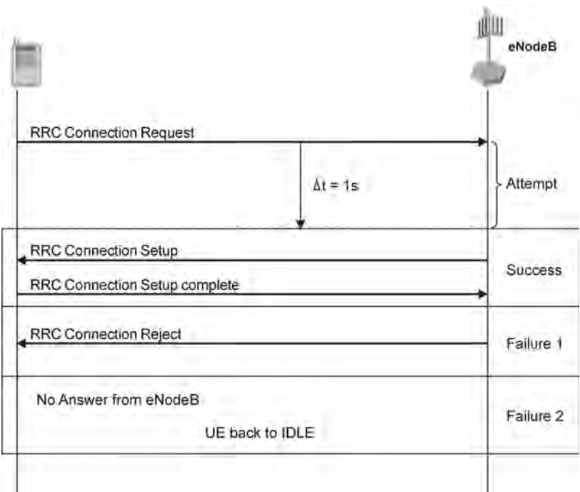
Figure 4.29 RRC connection setup procedure.
