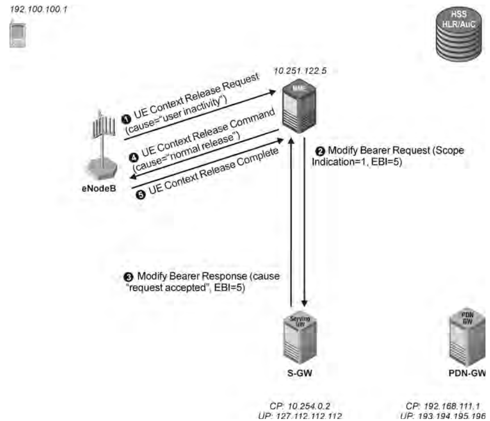
Figure 2.6 UE context release due to user inactivity. (Tektronix Communications).
