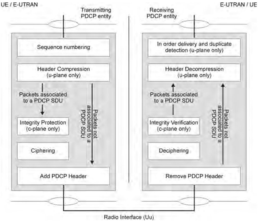
Figure 1.93 Functional overview of the PDCP layer (TS36.323). Reproduced with permission from © 3GPP™.
