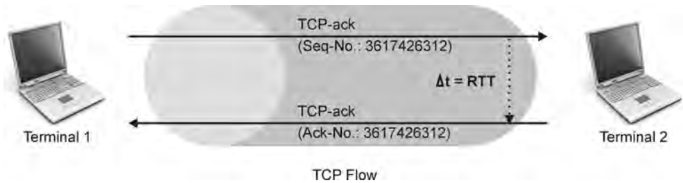
Figure 4.45 TCP round-trip time measurement principle.
