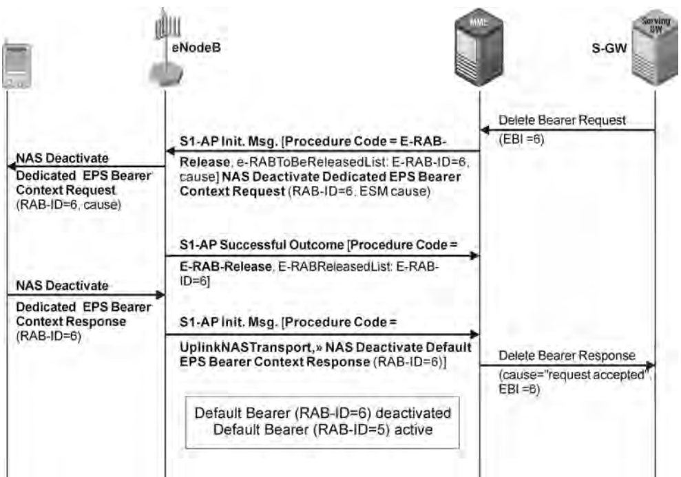
Figure 2.13 Dedicated bearer release. (Tektronix Communications).
