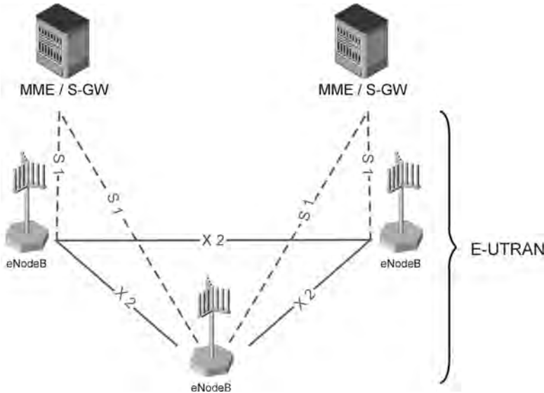
Figure 1.10 E-UTRAN network architecture (according to 3GPP 36.300). Reproduced with permission from © 2008 3GPP™.
