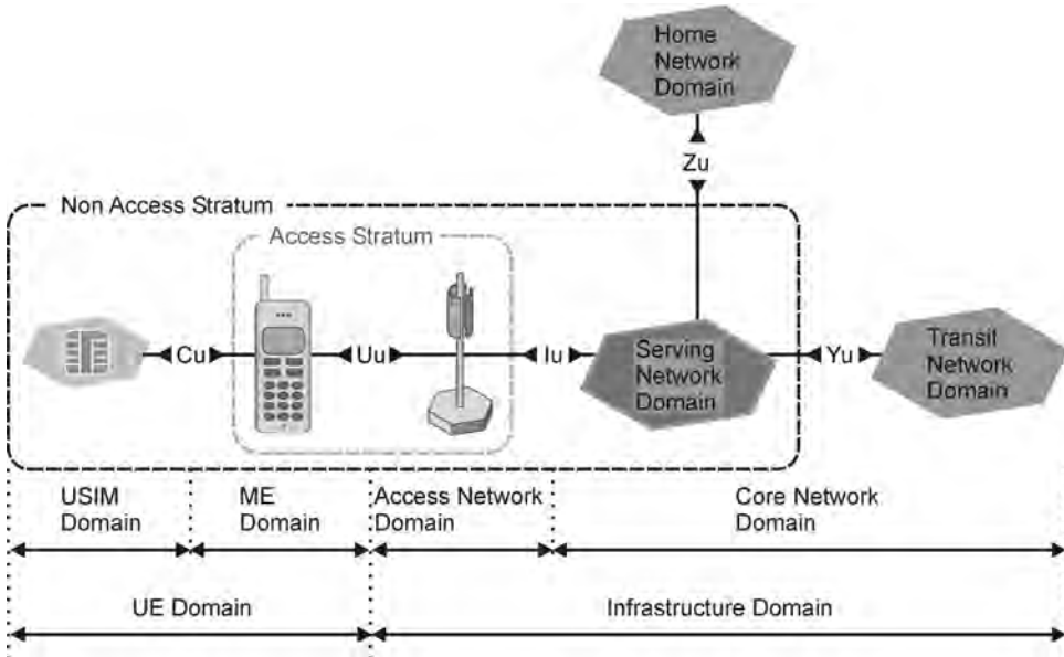
Figure 1.14 Domains and strata in E-UTRAN and EPC.
