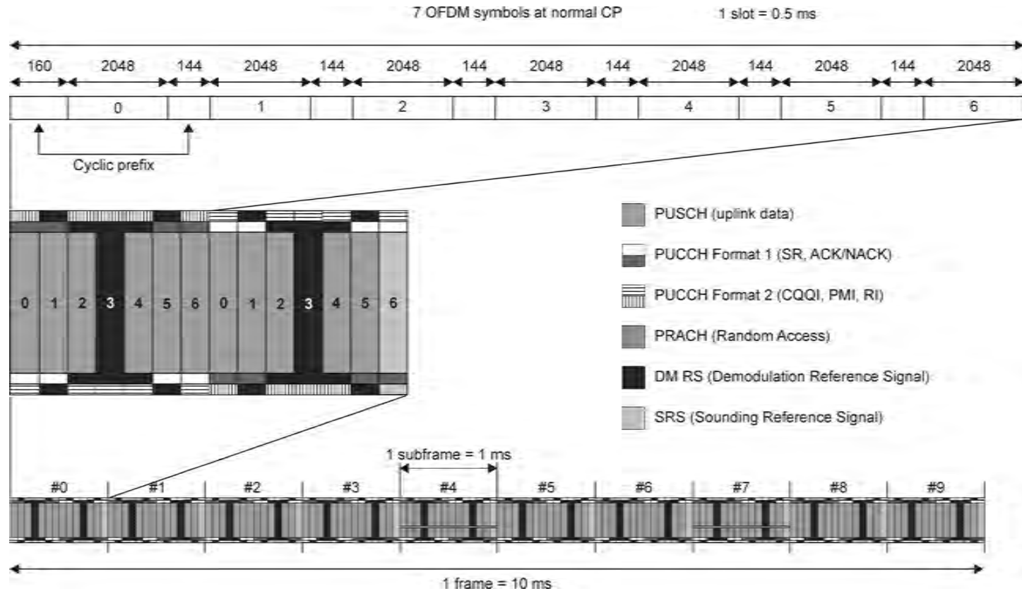
Figure 1.52 Uplink radio frame and subframe with two slots including PUSCH, PUCCH, PRACH, DMRS, and SRS. Reproduced with permission from Nomor.
