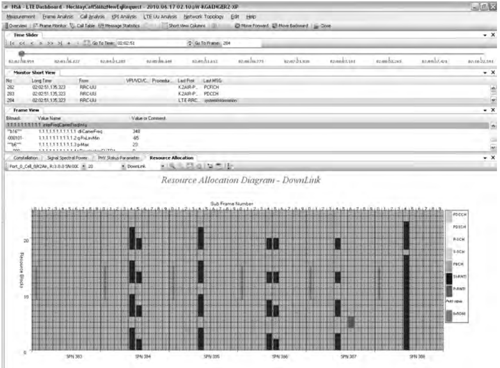
Figure 1.46 Scheduling and cell resource allocation analysis.
