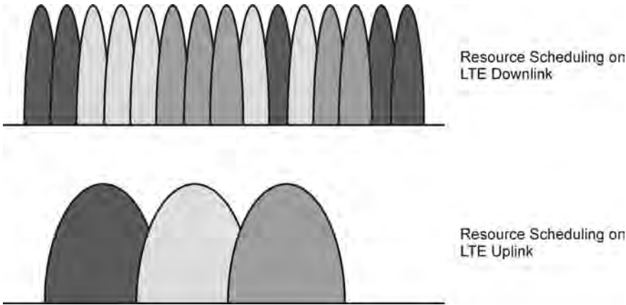
Figure 4.10 Resource scheduling for three different subscribers in same cell for downlink and uplink.
