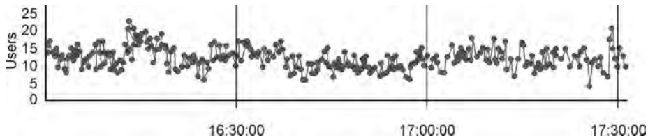
Figure 4.15 Number of active UEs (“users”) over time.
