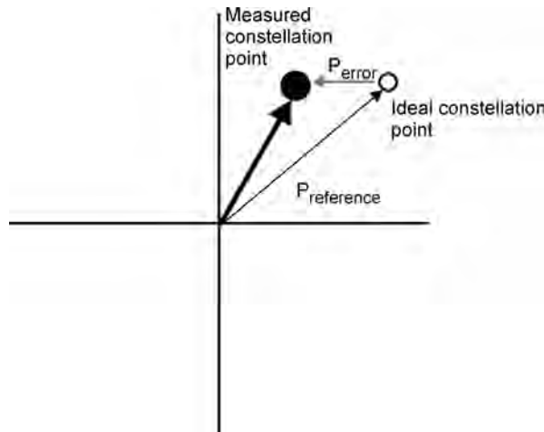
Figure 4.27 Measurements to compute EVM/MER.
