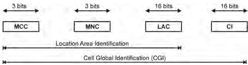
Figure 1.21 Structure of cell global identification (according to 3GPP 23.303). Reproduced with permission from © 3GPP™.
