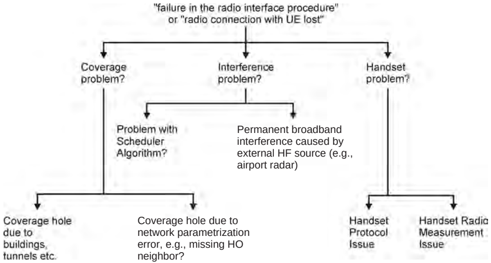
Figure 4.38 Possible root causes for an E-UTRAN call drop.
