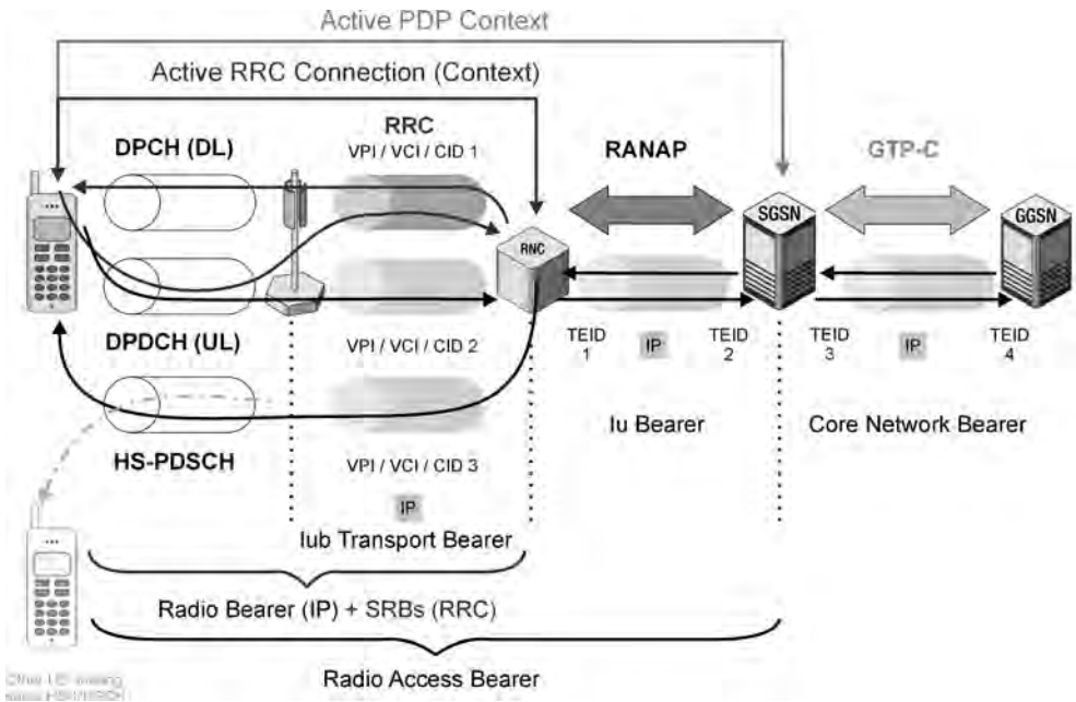
Figure 1.8 IP data transfer using HSDPA.
