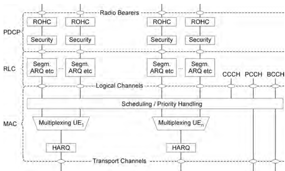
Figure 1.84 Layer 2 structure for DL (TS36.300). Reproduced with permission from © 3GPP™.
