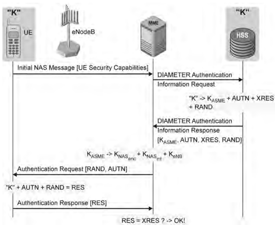
Figure 1.26 Subscriber authentication.
