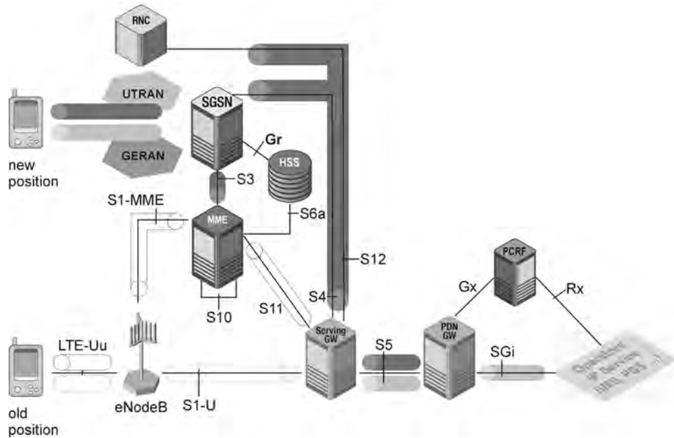
Figure 1.12 Connection after inter-RAT handover from E-UTRAN to UTRAN/GERAN.
