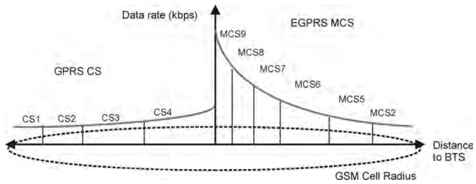
Figure 1.6 Cell footprint of maximum bit rate as function of MCS in (E)GPRS.
