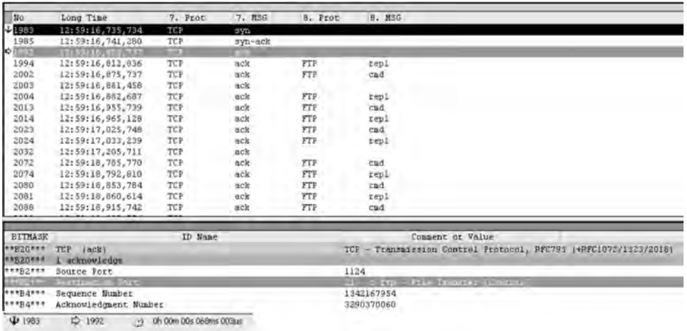
Figure 4.44 FTP (IP) service setup time.
