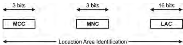
Figure 1.18 Structure of location area identification (according to 3GPP 23.303). Reproduced with permission from © 3GPP™.
