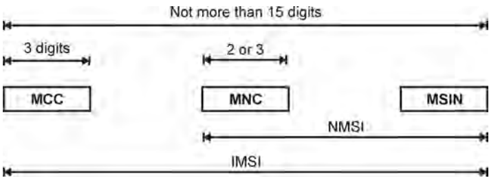
Figure 1.15 Structure of IMSI (according to 3GPP 23.303). Reproduced with permission from © 3GPP™.
