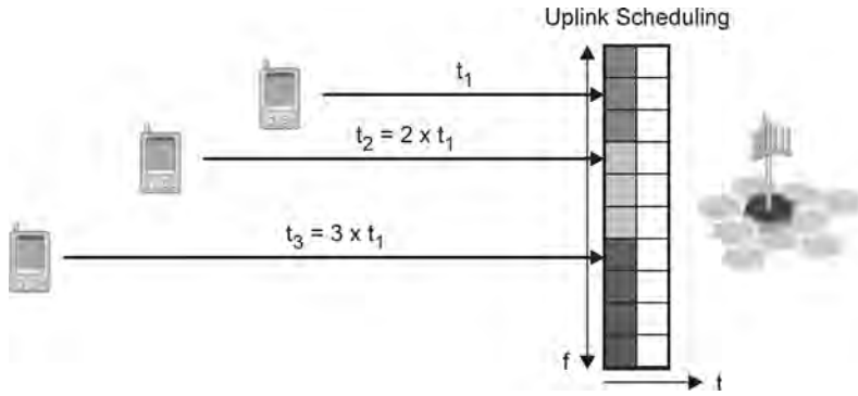
Figure 4.23 Timing advance principle.
