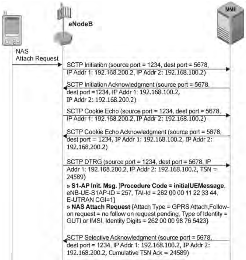
Figure 1.82 Sctp example.
