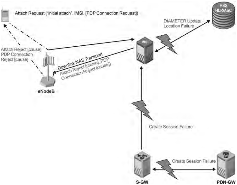
Figure 4.31 Attach failure due to failures in EPC.
