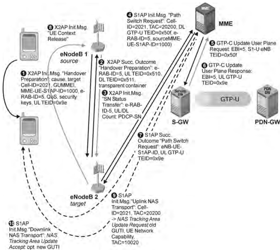
Figure 2.10 Inter-eNodeB handover over X2 – message flow. (Tektronix Communications).
