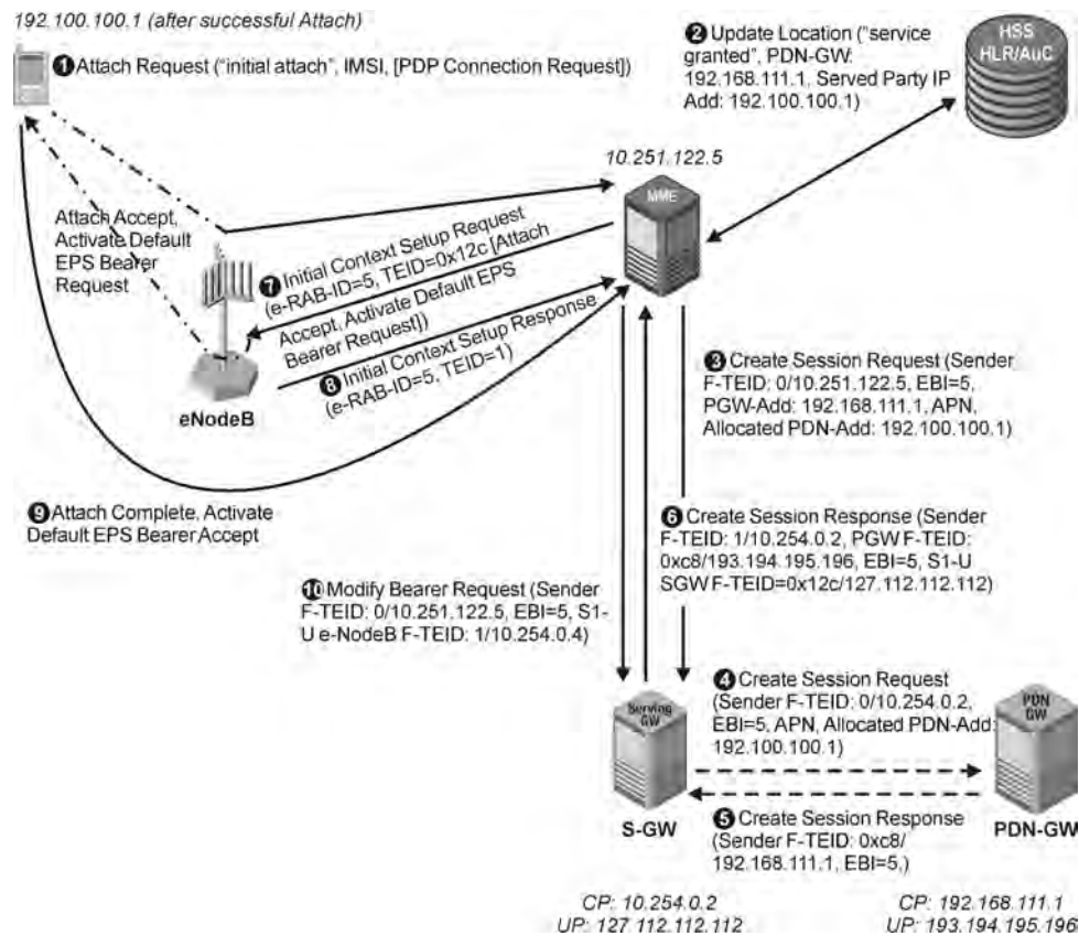
Figure 2.4 E-UTRAN attach procedure. (Tektronix Communications).
