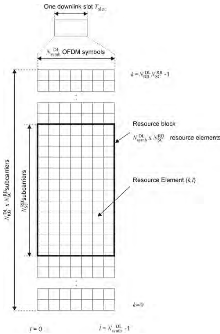
Figure 1.41 Downlink resource grid. Reproduced with permission from © 3GPP™.
