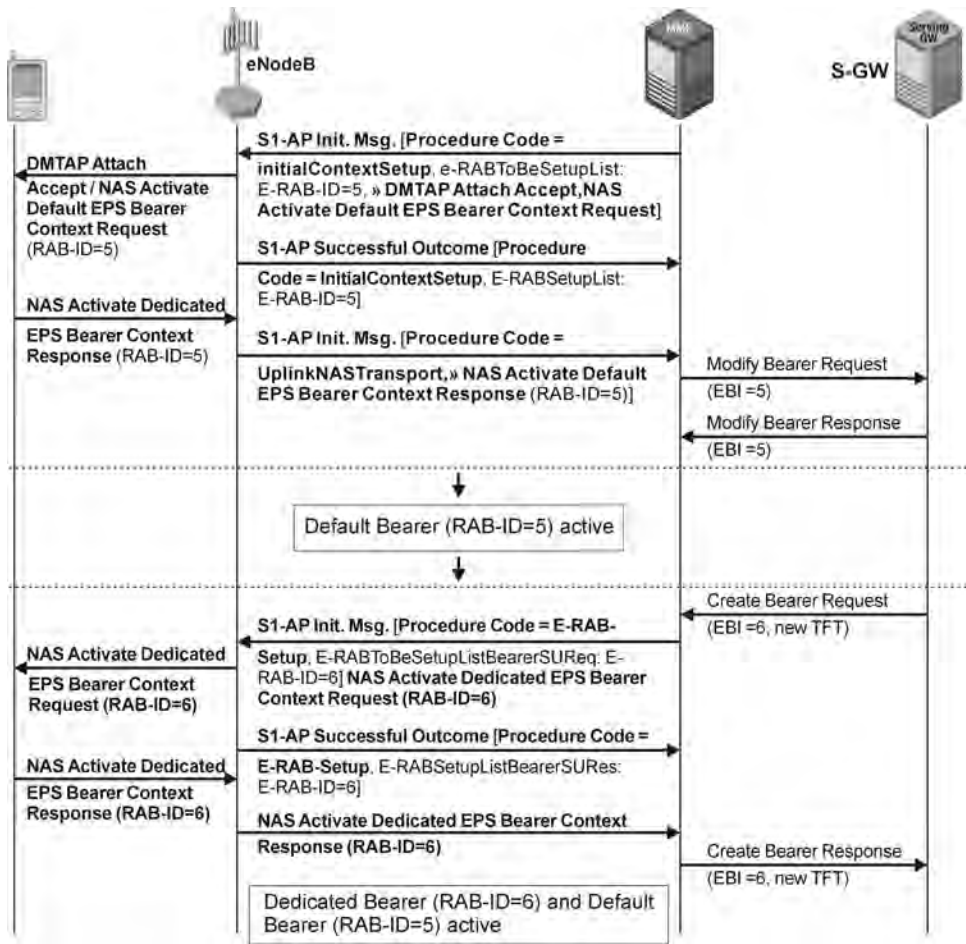
Figure 2.8 Dedicated bearer setup. (Tektronix Communications).
