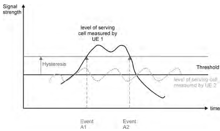
Figure 1.97 Hysteresis parameter for RRC measurements.
