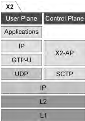
Figure 1.73 Protocol stack X2 control/user plane.
