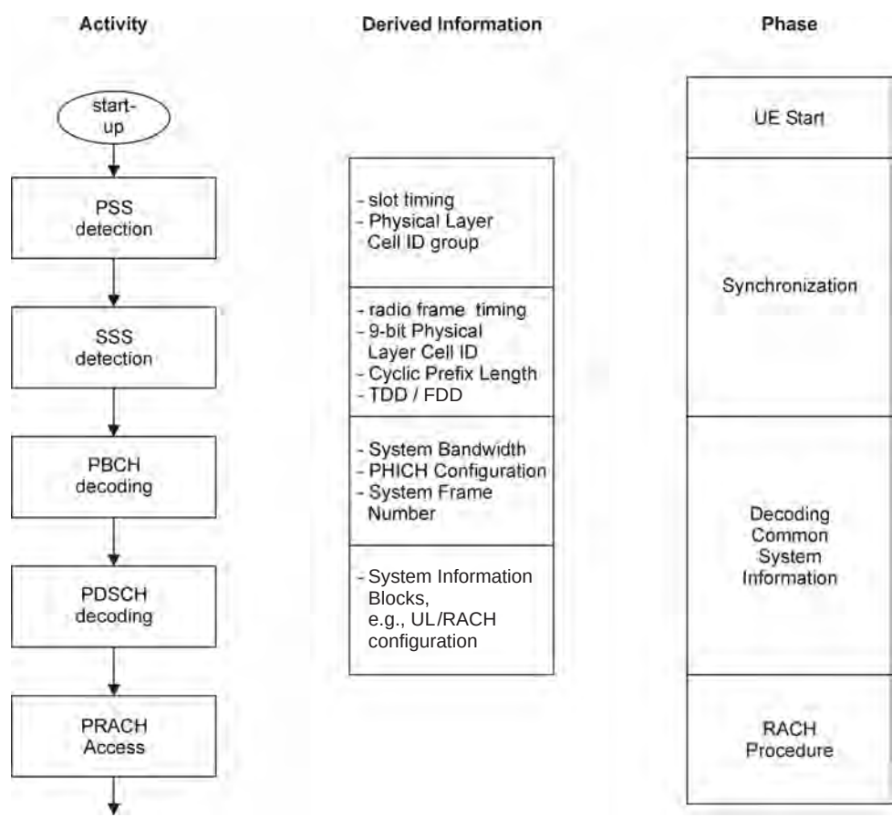
Figure 1.66 Initial cell access with level of retrieved information.
