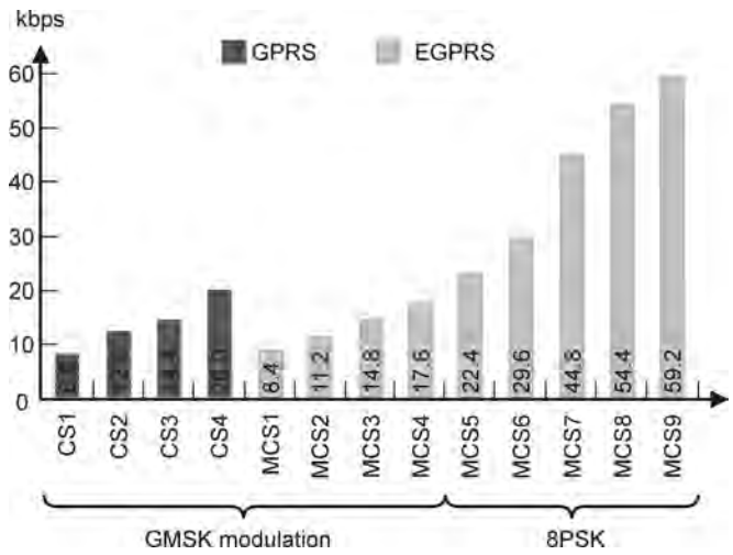
Figure 1.5 Modulation/coding scheme and maximum bit rate in GSM/GPRS vs. EGPRS.
