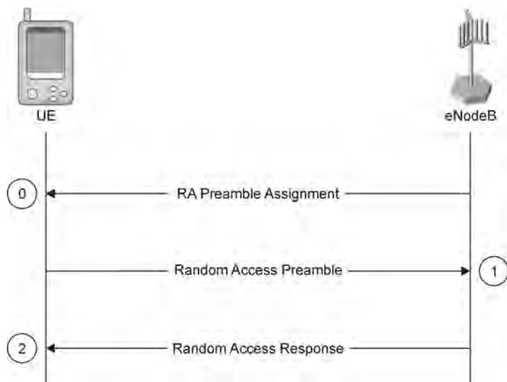
Figure 1.70 Non-contention-based random access procedure. Reproduced with permission from © 3GPP™.
