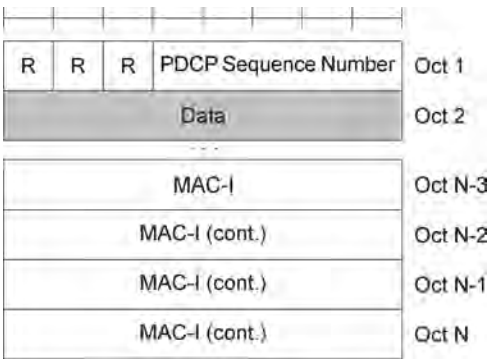
Figure 1.94 Format of PDCP data PDU for transport of signaling radio bearer information. Reproduced with permission from © 3GPP™.
