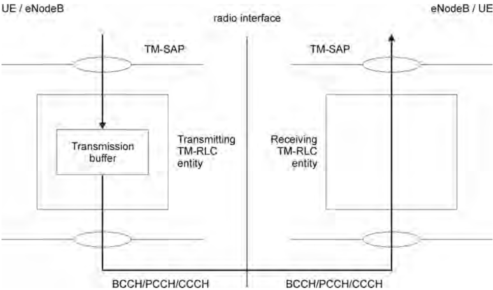
Figure 1.88 Model of two Transparent Mode peer entities. Reproduced with permission from © 3GPP™.
