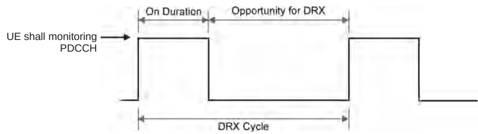
Figure 1.48 DRX cycle. Reproduced with permission from © 3GPP™.
