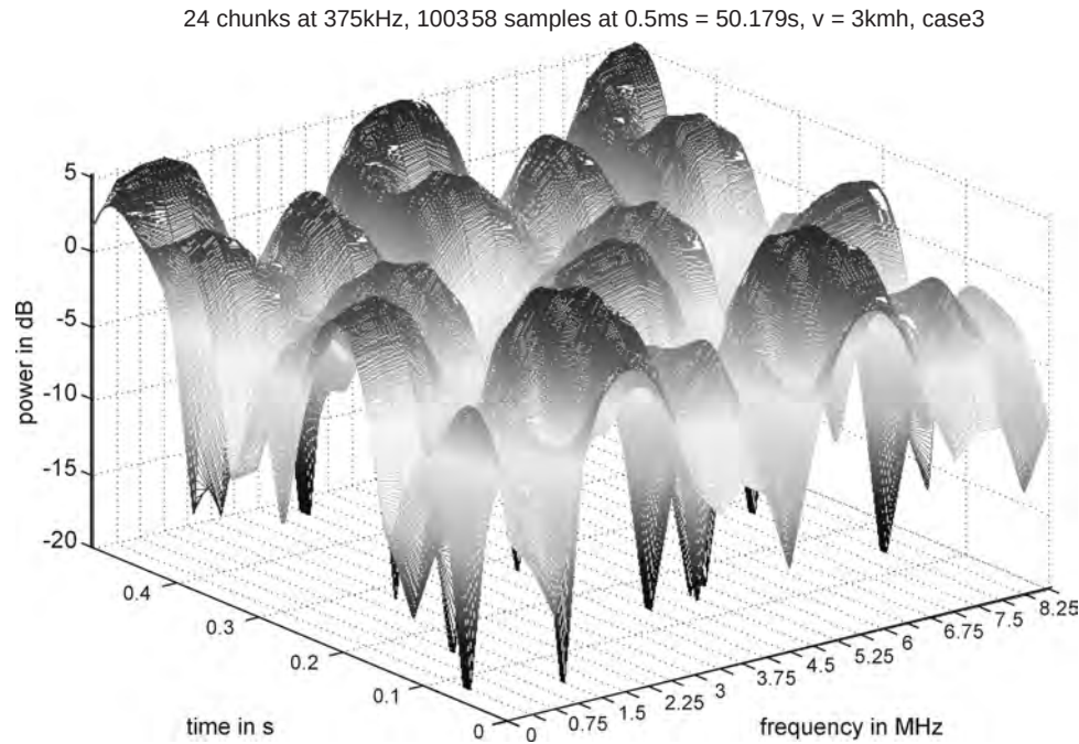
Figure 1.29 Time-variant frequency-selective wireless channel. Reproduced with permission from Nomor.
