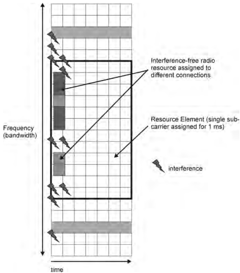
Figure 4.9 Scheduling of radio resources avoiding interference.
