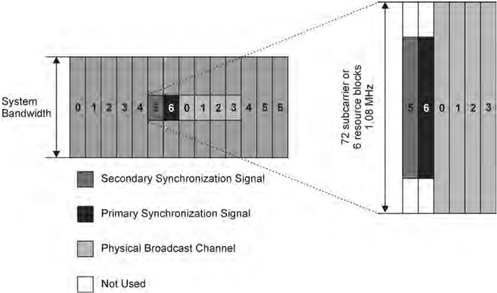
Figure 1.61 Illustration of the location of the physical broadcast channel and the primary and secondary synchronization signals within the first subframe of each radio frame. Reproduced with permission from Nomor.
