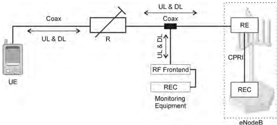
Figure 4.4 Coax-based monitoring of the air interface.
