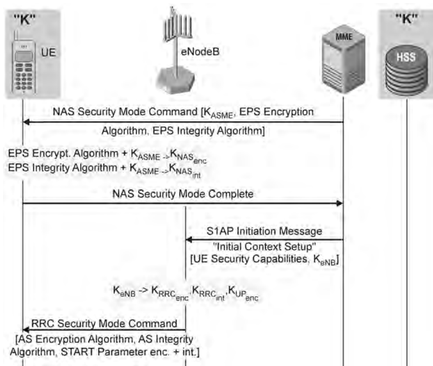
Figure 1.27 NAS security initiation and RRC security initiation.
