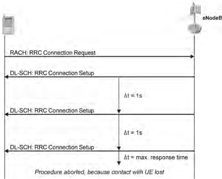
Figure 4.30 RRC setup timeout on UE side.
