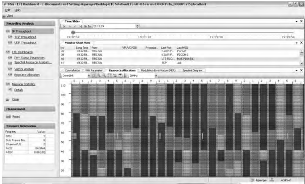
Figure 4.14 Visualized downlink scheduling for four individual subscribers.
