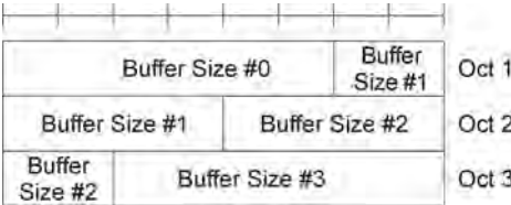
Figure 4.21 Long buffer status MAC control element. Reproduced with permission from © 3GPP™.
