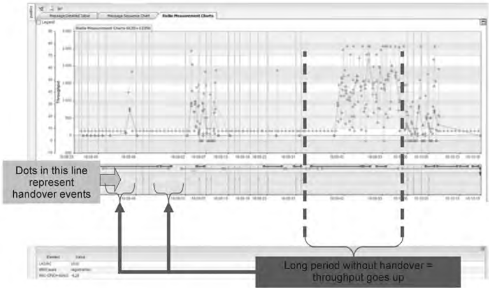
Figure 4.39 Throughput measurement graph of a single connection correlated with occurrence of handover events.
