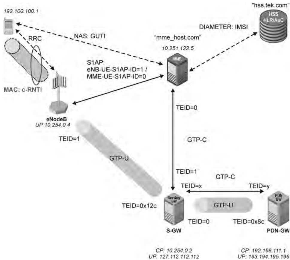
Figure 2.5 Signaling and user plane connection after successful attach. (Tektronix Communications).
