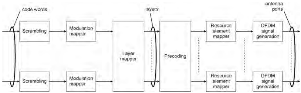
Figure 1.38 Overview of physical channel processing. Reproduced with permission from © 3GPP™.
