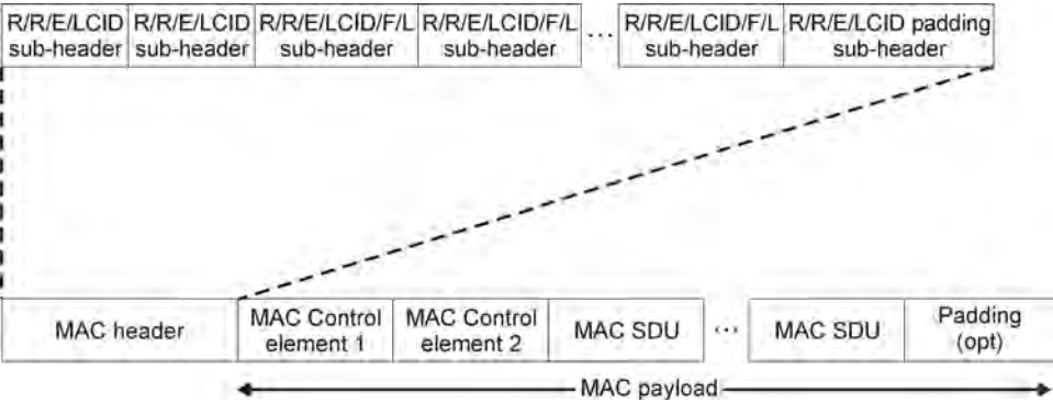
Figure 1.86 Example of MAC PDU consisting of MAC header, MAC control elements, MAC SDUs, and padding (TS36.321). Reproduced with permission from © 3GPP™.
