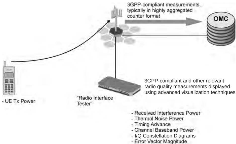
Figure 4.16 Uplink radio quality measurements and layer 2 measurements.
