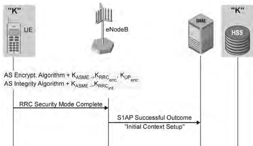
Figure 1.28 RRC security completion.
