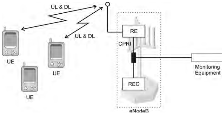
Figure 4.5 CPRI-based monitoring.
