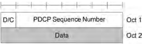
Figure 1.95 Format of PDCP data PDU for transport of user plane information. Reproduced with permission from © 3GPP™.
