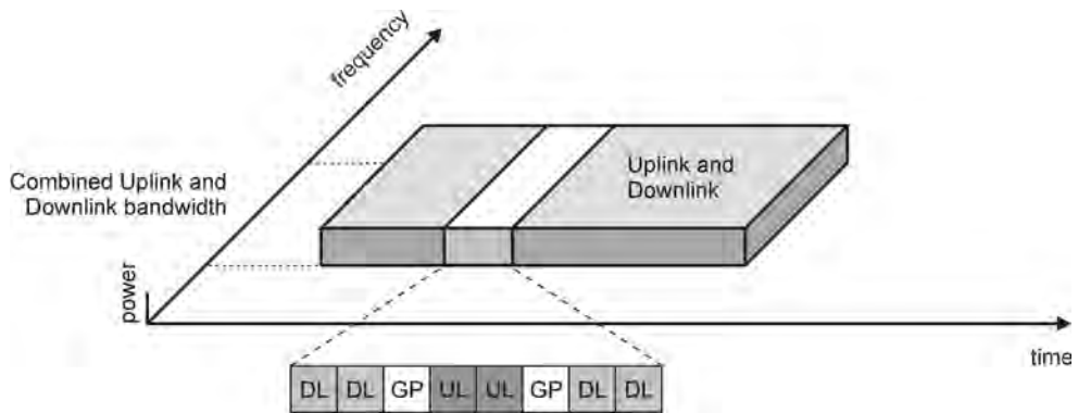
Figure 1.31 TDD system with example duplex slot structure.
