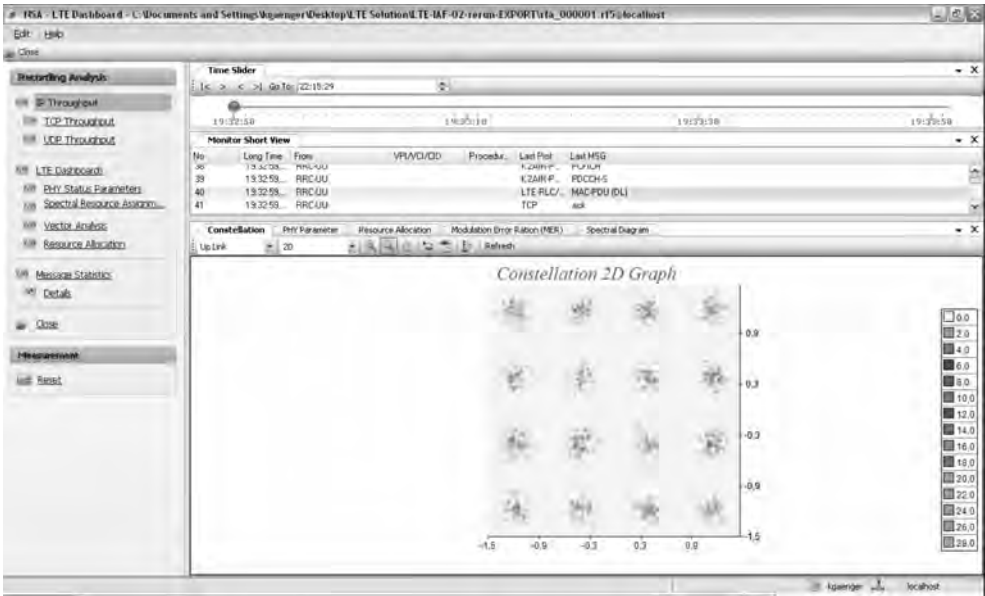
Figure 4.25 Two-dimensional I/Q constellation diagram.
