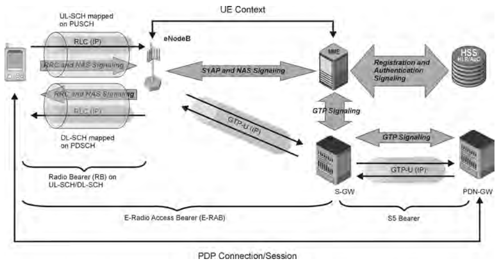
Figure 1.9 Packet data transfer in E-UTRAN/EPC.
