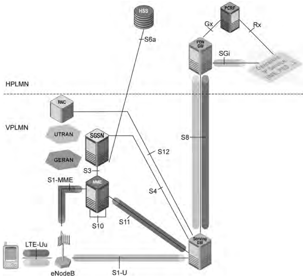
Figure 1.13 Connection via E-UTRAN with roaming in EPC.
