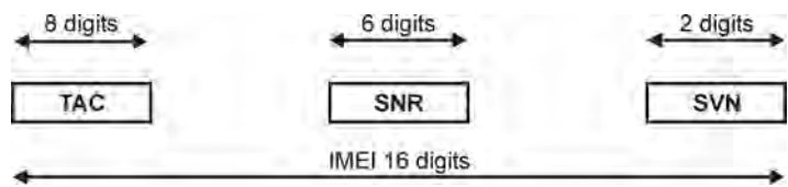
Figure 1.17 Structure of IMEISV (according to 3GPP 23.303). Reproduced with permission from © 3GPP™.
