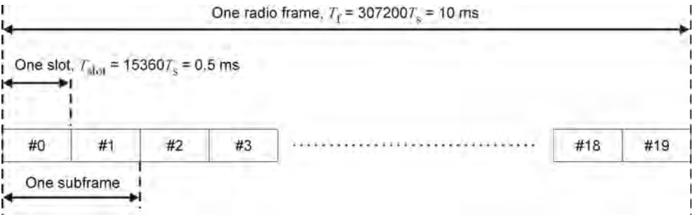
Figure 1.42 Frame structure type 1 used with FDD TS36.211. Reproduced with permission from © 3GPP™.
