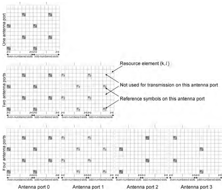
Figure 1.44 Mapping of downlink reference signals (normal cyclic prefix) (TS36.211). Reproduced with permission from © 3GPP™.
