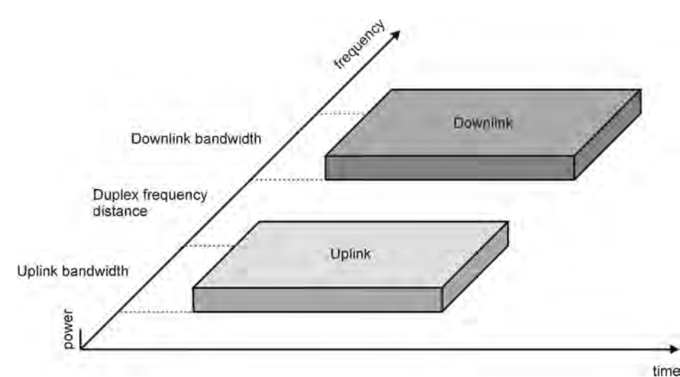
Figure 1.30 FDD system.
