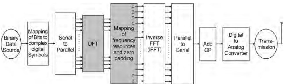
Figure 1.49 Block diagram of SC-FDMA transmitter with localized mapping to frequency resources.
