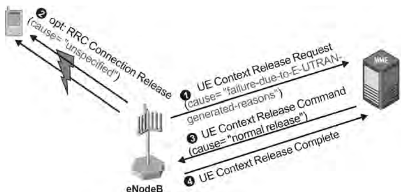
Figure 4.37 Call drop due to transmission failures on the radio interface.
