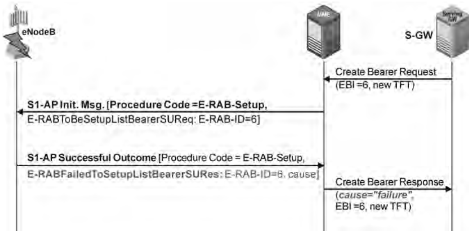
Figure 4.36 Dedicated bearer setup failure.
