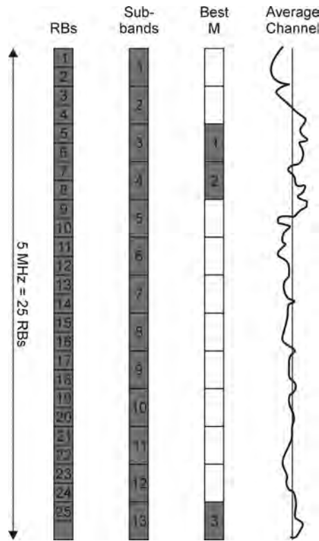
Figure 1.56 CQI illustration with sub-bands and best M reporting. Reproduced with permission from Nomor.
