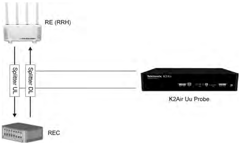
Figure 4.6 Regular two-fiber CPRI architecture.
