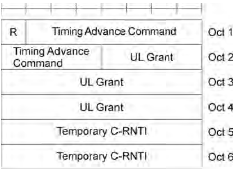
Figure 1.69 A 6-byte MAC RAR (TS36.321). Reproduced with permission from © 3GPP™.
