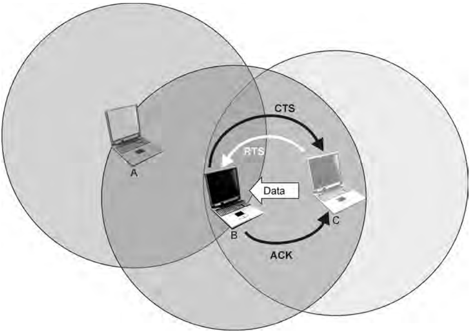
Figure 1.32 Illustration of the hidden terminal effect.
