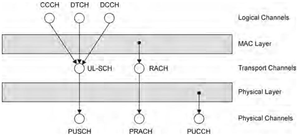
Figure 1.65 Uplink channel mapping and multiplexing from logical channels via transport channels to physical channels.
