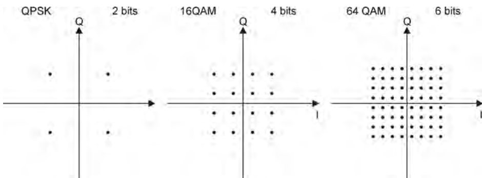
Figure 1.54 Different QAM schemes used with LTE and the number of bits mapped to each scheme.
