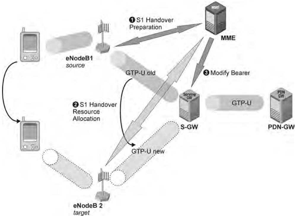
Figure 2.11 Overview of S1 handover. (Tektronix Communications).
