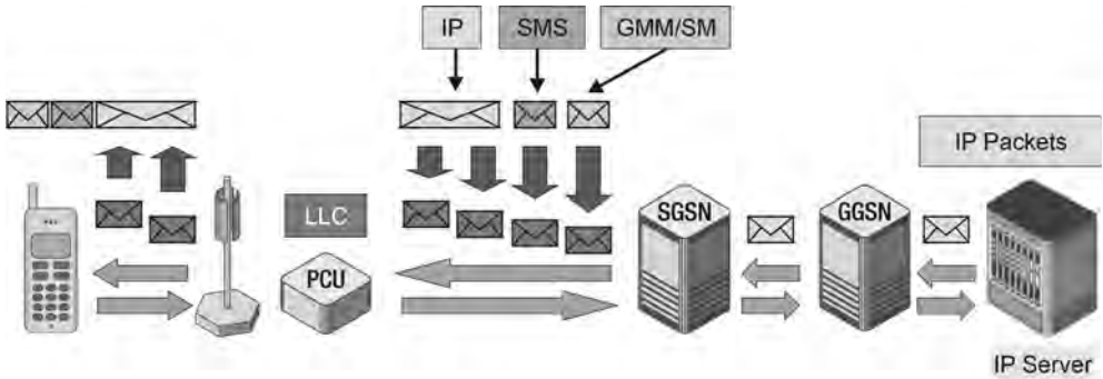
Figure 1.3 Packet data transfer in 2.5G GPRS.
