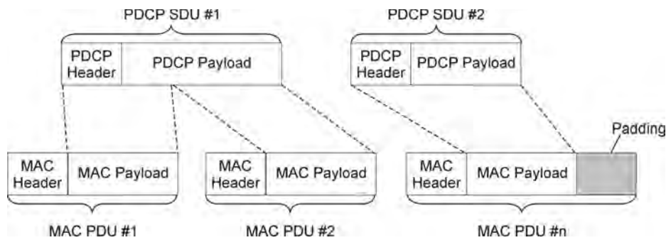
Figure 1.89 Example of RLC segmentation of PDCP SDUs into MAC PDUs. The MAC Payload is equivalent to RLC PDUs.
