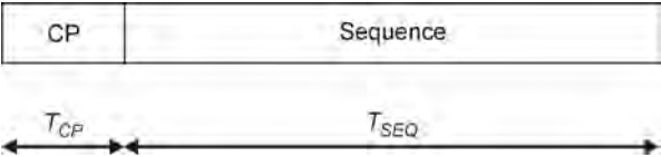
Figure 3.1 Random access preamble format (according to 3GPP 36.211).
