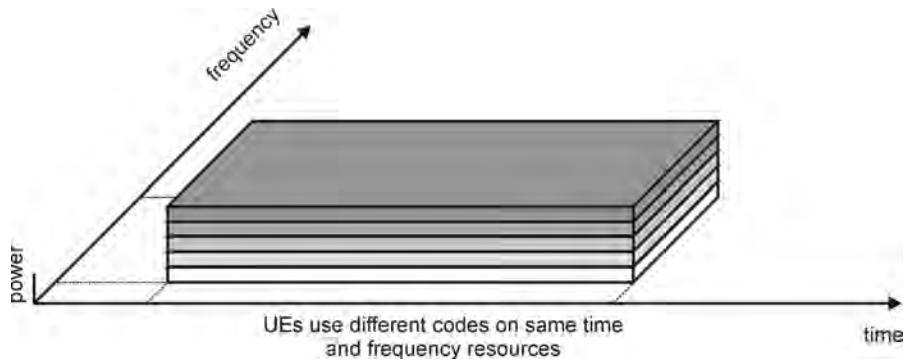
Figure 1.35 Code Division Multiple Access (CDMA).
