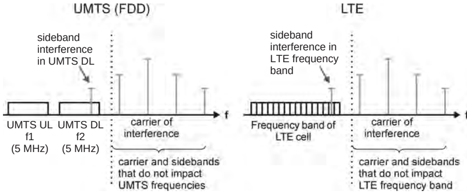
Figure 4.22 Impact of external interference in UMTS and LTE cells.
