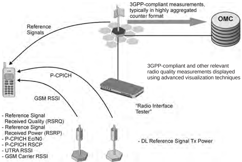
Figure 4.17 Downlink radio quality measurements.
