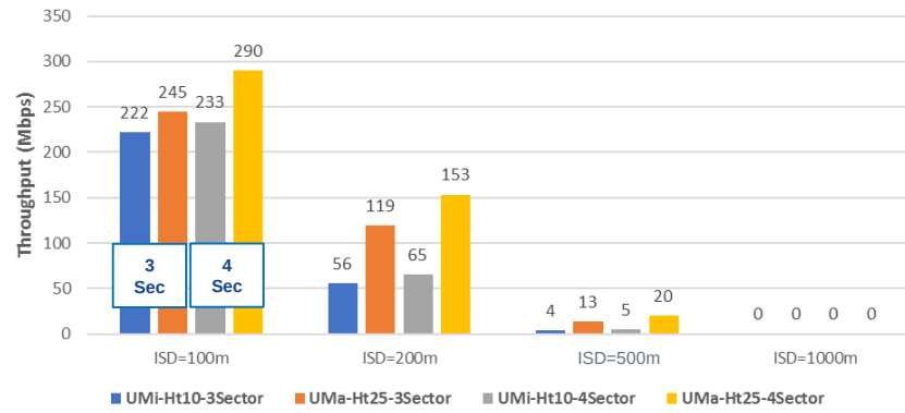
DOWNLINK - 800MHz - EIRP=60dBm - CELL EDGE THROUGHPUT
