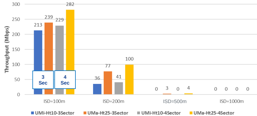
DOWNLINK - 800MHz - EIRP=54dBm - CELL EDGE THROUGHPUT
