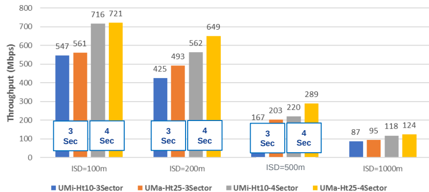
DOWNLINK - 800MHz - EIRP=54dBm - MEAN UE THROUGHPUT
