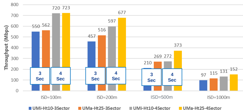
DOWNLINK - 800MHz - EIRP=60dBm - MEAN UE THROUGHPUT
