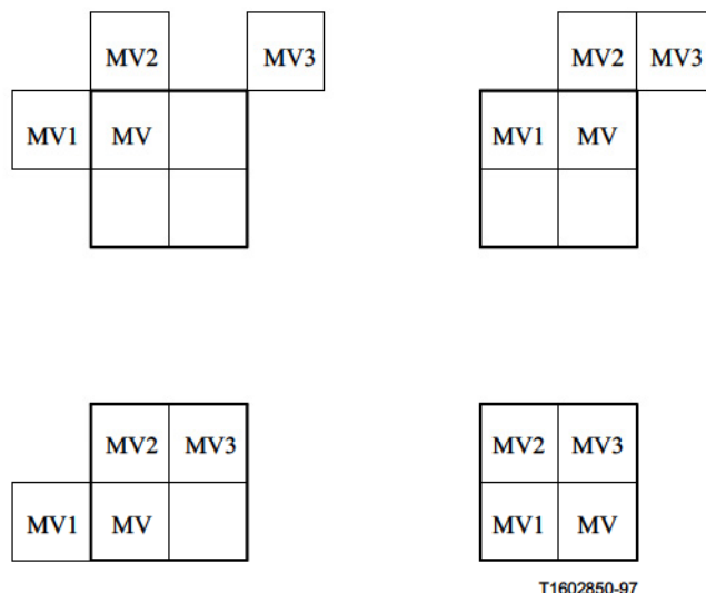
Figure F.1/H.263 – Redefinition of the candidate predictors MV1, MV2 and MV3 for each of the luminance blocks in a macroblock
