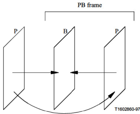
Figure G.1/H.263 – Prediction in PB-frames mode
