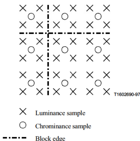
Figure 2/H.263 – Positioning of luminance and chrominance samples
