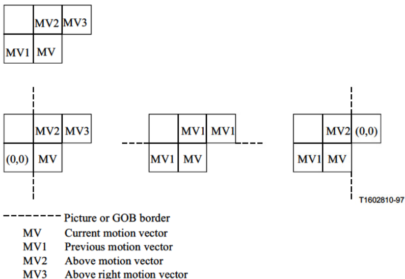
Figure 12/H.263 – Motion vector prediction
