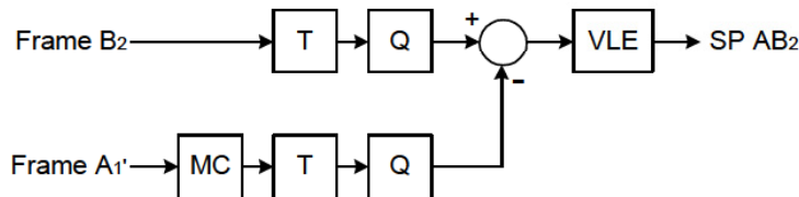
Figure 2-6 Encoding SP-slice AB_2 (simplified)
