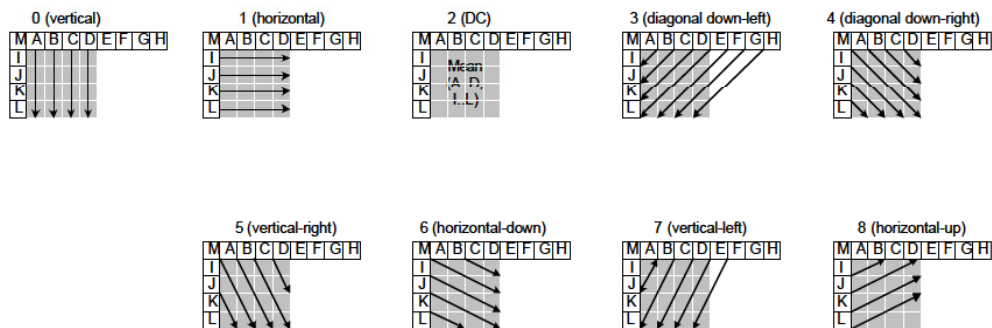
Figure 3 4x4 luma prediction modes
