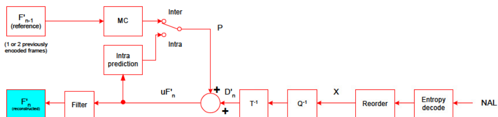
Figure 2-2 AVC Decoder
