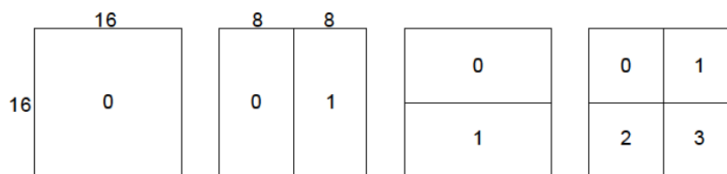
Figure 2-1 Macroblock partitions: 16x16, 8x16, 16x8, 8x8
