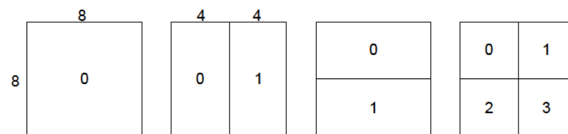
Figure 2-2 Macroblock sub-partitions: 8x8, 4x8, 8x4, 4x4
