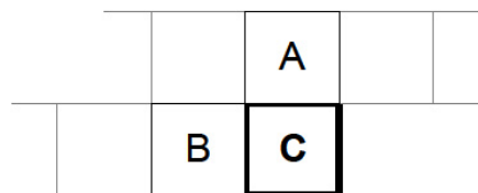
Figure 8 Adjacent 4x4 intra coded blocks
