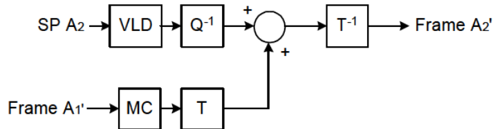
Figure 2-5 Decoding SP-slice A_2 (simplified)
