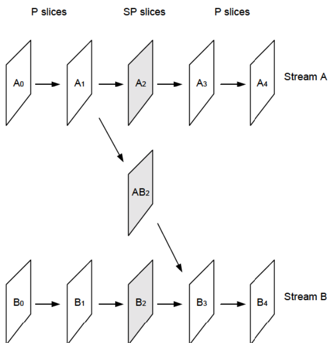
Figure 2-2 Switching streams using SP-slices
