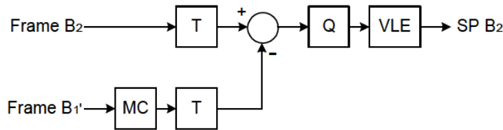
Figure 2-4 Encoding SP-slice B_2 (simplified)
