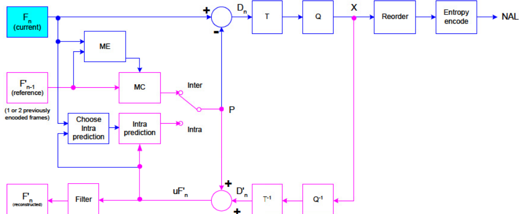
Figure 2-1 AVC Encoder
