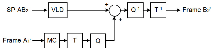
Figure 2-7 Decoding SP-slice AB_2
