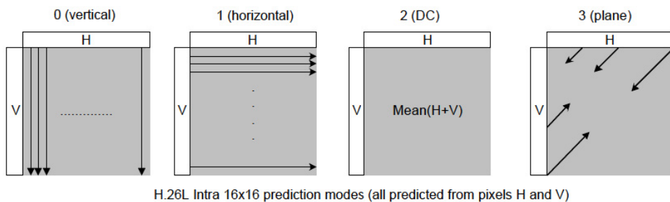
Figure 5 Intra 16x16 prediction modes
