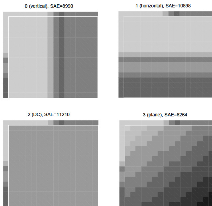
Figure 7 Intra 16x16 predictions
