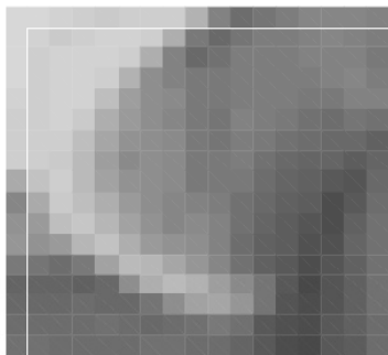
Figure 6 16x16 macroblock
