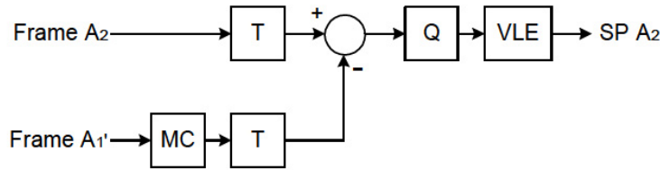
Figure 2-3 Encoding SP slice A_2 (simplified)
